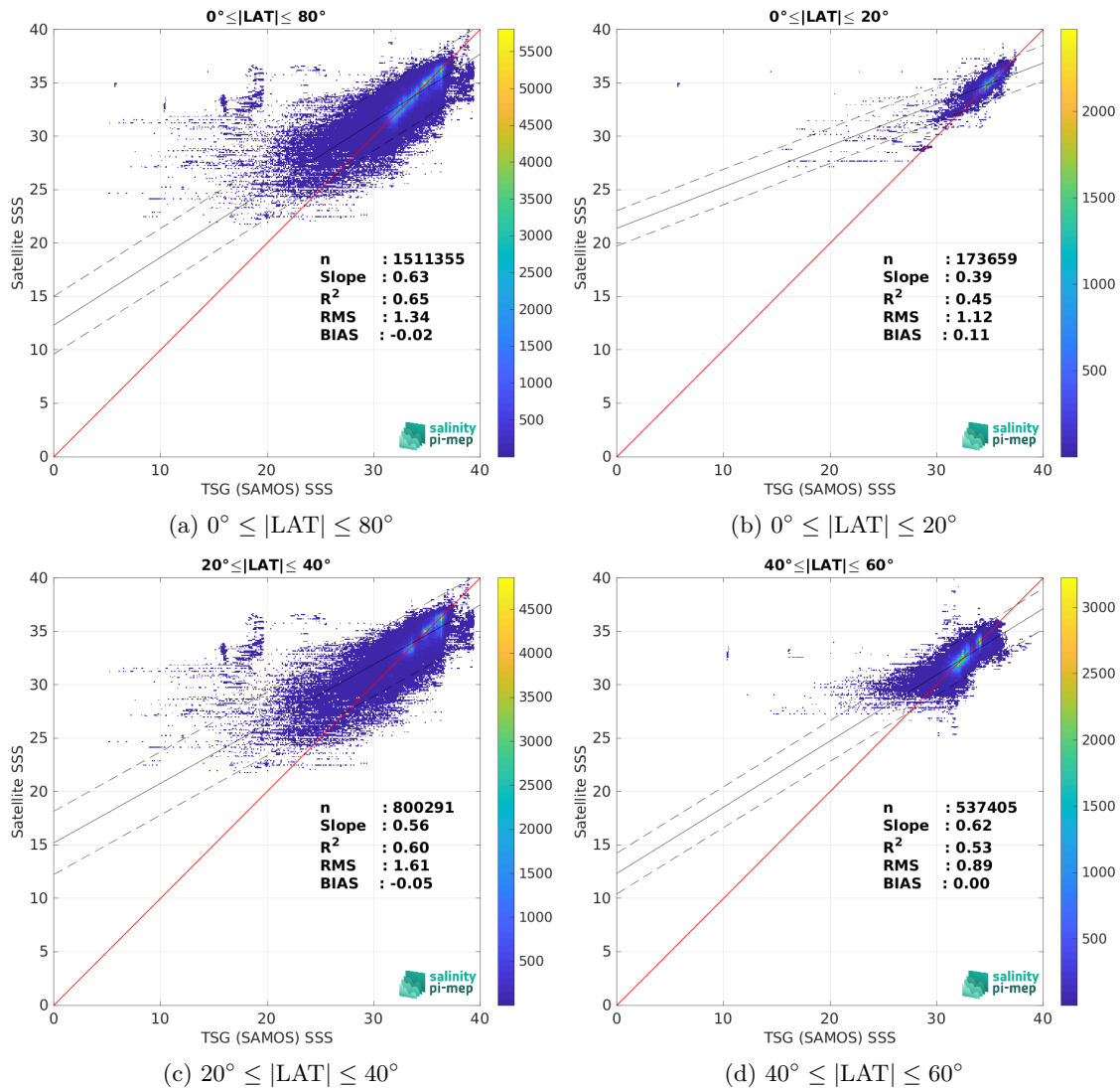
Figure 9: Contour maps of the concentration of SMOS SSS L3 v2 - 9-Days (BEC) SSS (y-axis) versus TSG (SAMOS) SSS (x-axis) at match-up pairs for different latitude bands. For each plot, the red line shows x=y . The black thin and dashed lines indicate a linear fit through the data cloud and the \pm 95\% confidence levels, respectively. The number match-up pairs n , the slope and R^2 coefficient of the linear fit, the root mean square (RMS) and the mean bias between satellite and in situ data are indicated for each latitude band in each plots.
