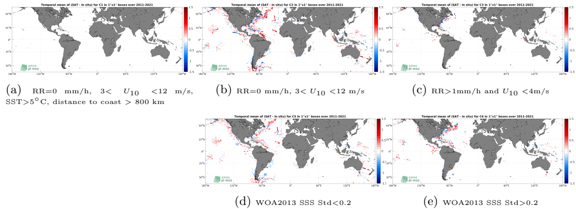
Figure 12: Temporal mean gridded over spatial boxes of size 1^\circ \times 1^\circ of \Delta\text{SSS} (SMOS SSS L3 v2 - 9-Days (BEC) - TSG (SAMOS)) for 5 different subdatasets corresponding to:RR=0 mm/h, 3 < U_{10} < 12 m/s, SST >5^\circ\text{C} , distance to coast > 800 km (a), RR=0 mm/h, 3 < U_{10} < 12 m/s (b), RR >1 mm/h and U_{10} < 4 m/s (c), WOA2013 SSS Std <0.2 (d), WOA2013 SSS Std >0.2 (e).
