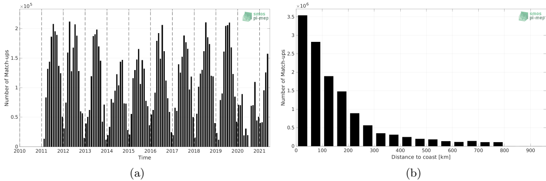
Figure 1: Number of match-ups between TSG (SAMOS) and SMOS SSS L3 v2 - 9-Days (BEC) SSS as a function of time (a) and as function of the distance to coast (b) over the SMOS coastal zone (<800km) 60N-60S Pi-MEP region and for the full satellite product period.
