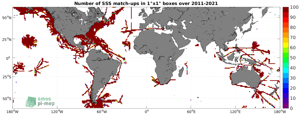
Figure 4: Number of SSS match-ups between TSG (SAMOS) SSS and the SMOS SSS L3 v2 - 9-Days (BEC) SSS product for the SMOS coastal zone (<800km) 60N-60S Pi-MEP region over 1^\circ \times 1^\circ boxes and for the full satellite product period.
