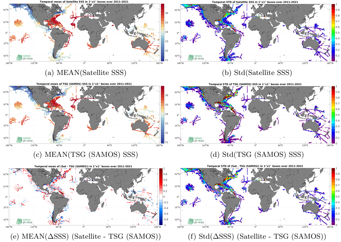
Figure 6: Temporal mean (left) and Std (right) of SSS from SMOS SSS L3 v2 - 9-Days (BEC) (top), TSG (SAMOS) (middle), and of \Delta SSS (Satellite - TSG (SAMOS)). Only match-up pairs are used to generate these maps.
