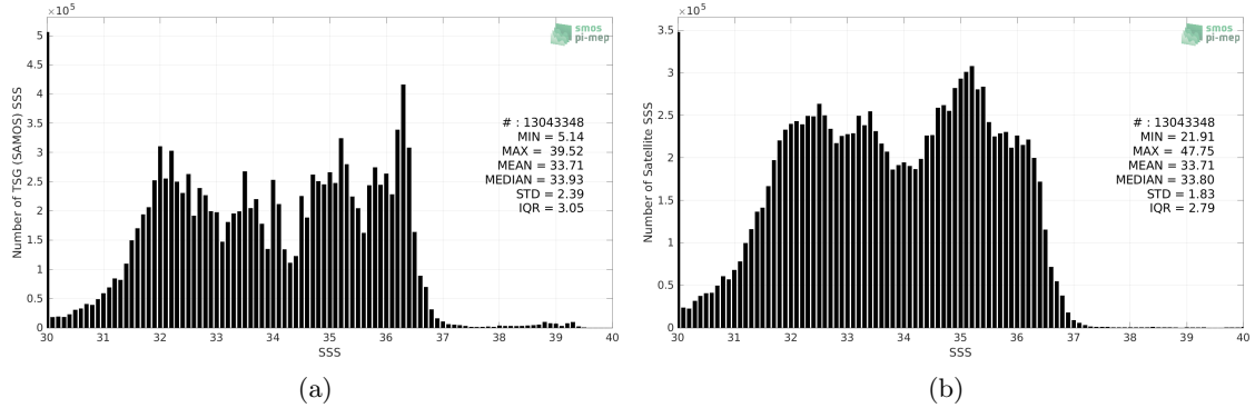
Figure 2: Histograms of SSS from TSG (SAMOS) (a) and SMOS SSS L3 v2 - 9-Days (BEC) (b) considering all match-up pairs per bins of 0.1 over the SMOS coastal zone (<800km) 60N-60S Pi-MEP region and for the full satellite product period.
