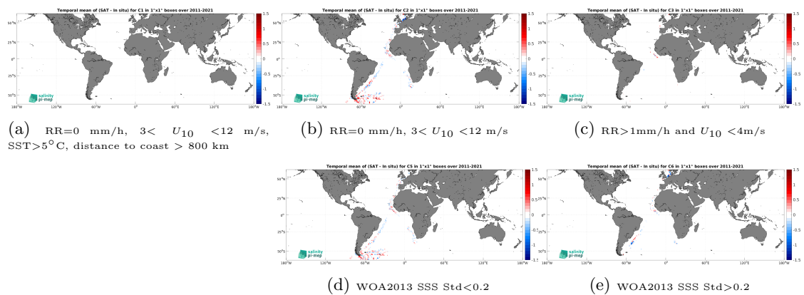
Figure 14: Temporal mean gridded over spatial boxes of size 1^\circ \times 1^\circ of \Delta\text{SSS} (SMOS SSS L3 v2 - 9-Days (BEC) - TSG (Polarstern)) for 5 different subdatasets corresponding to:RR=0 mm/h, 3 < U_{10} < 12 m/s, SST>5°C, distance to coast > 800 km (a), RR=0 mm/h, 3 < U_{10} < 12 m/s (b), RR>1mm/h and U_{10} < 4 m/s (c), WOA2013 SSS Std<0.2 (d), WOA2013 SSS Std>0.2 (e).
