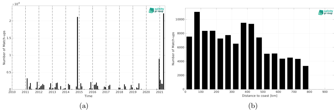
Figure 2: Number of match-ups between TSG (Polarstern) and SMOS SSS L3 v2 - 9-Days (BEC) SSS as a function of time (a) and as function of the distance to coast (b) over the SMOS coastal zone (<800km) 60N-60S Pi-MEP region and for the full satellite product period.
