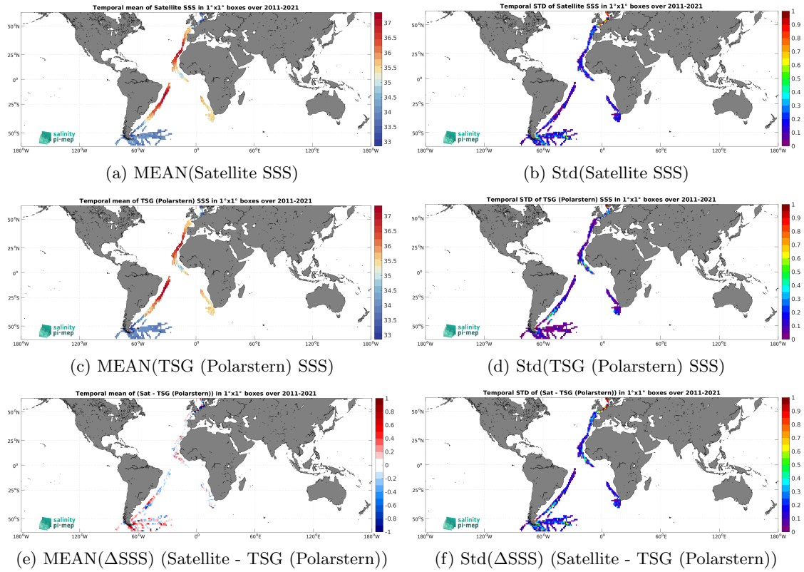
Figure 7: Temporal mean (left) and Std (right) of SSS from SMOS SSS L3 v2 - 9-Days (BEC) (top), TSG (Polarstern) (middle), and of \Delta SSS (Satellite - TSG (Polarstern)). Only match-up pairs are used to generate these maps.
