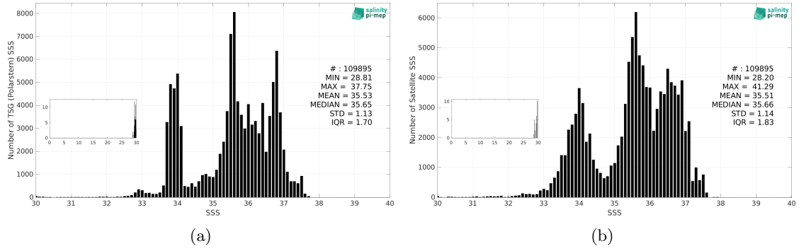
Figure 3: Histograms of SSS from TSG (Polarstern) (a) and SMOS SSS L3 v2 - 9-Days (BEC) (b) considering all match-up pairs per bins of 0.1 over the SMOS coastal zone (<800km) 60N-60S Pi-MEP region and for the full satellite product period.
