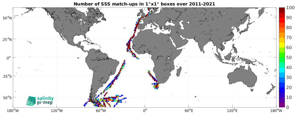
Figure 5: Number of SSS match-ups between TSG (Polarstern) SSS and the SMOS SSS L3 v2 - 9-Days (BEC) SSS product for the SMOS coastal zone (<800km) 60N-60S Pi-MEP region over 1^\circ \times 1^\circ boxes and for the full satellite product period.
