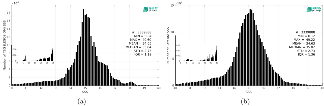
Figure 3: Histograms of SSS from TSG (LEGOS-DM) (a) and SMOS SSS L3 v2 - 9-Days (BEC) (b) considering all match-up pairs per bins of 0.1 over the SMOS coastal zone (<800km) 60N-60S Pi-MEP region and for the full satellite product period.
