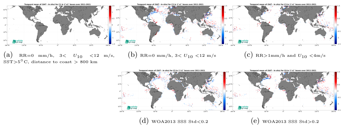
Figure 14: Temporal mean gridded over spatial boxes of size 1^\circ \times 1^\circ of \Delta\text{SSS} (SMOS SSS L3 v2 - 9-Days (BEC) - TSG (LEGOS-DM)) for 5 different subdatasets corresponding to:RR=0 mm/h, 3 < U_{10} < 12 m/s, SST >5^\circ\text{C} , distance to coast > 800 km (a), RR=0 mm/h, 3 < U_{10} < 12 m/s (b), RR >1 mm/h and U_{10} < 4 m/s (c), WOA2013 SSS Std <0.2 (d), WOA2013 SSS Std >0.2 (e).
