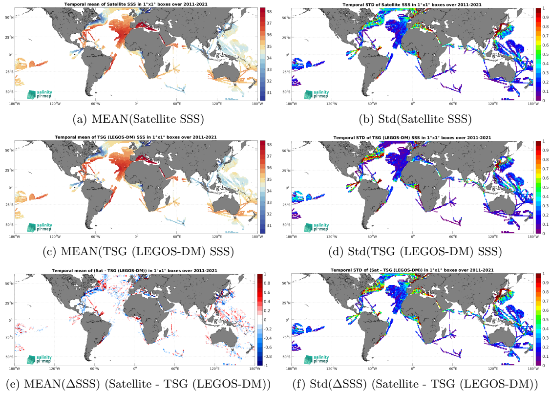
Figure 7: Temporal mean (left) and Std (right) of SSS from SMOS SSS L3 v2 - 9-Days (BEC) (top), TSG (LEGOS-DM) (middle), and of \Delta SSS (Satellite - TSG (LEGOS-DM)). Only match-up pairs are used to generate these maps.
