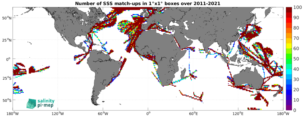
Figure 5: Number of SSS match-ups between TSG (LEGOS-DM) SSS and the SMOS SSS L3 v2 - 9-Days (BEC) SSS product for the SMOS coastal zone (<800km) 60N-60S Pi-MEP region over 1^\circ \times 1^\circ boxes and for the full satellite product period.
