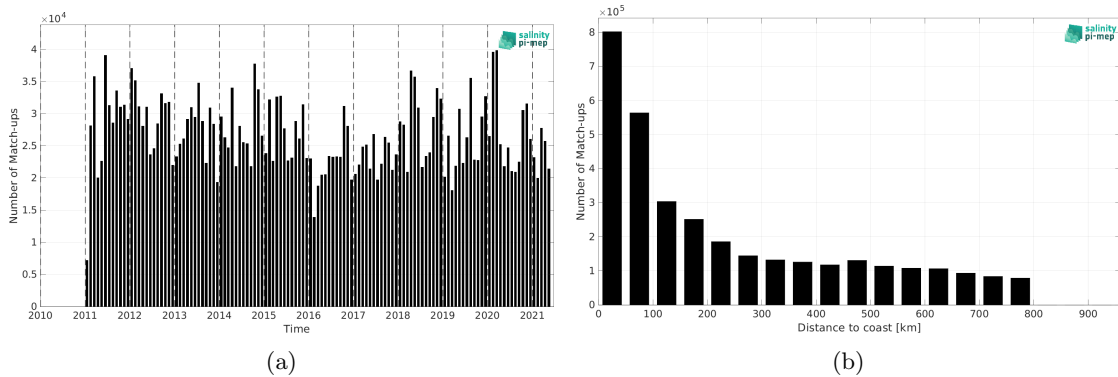
Figure 2: Number of match-ups between TSG (LEGOS-DM) and SMOS SSS L3 v2 - 9-Days (BEC) SSS as a function of time (a) and as function of the distance to coast (b) over the SMOS coastal zone (<800km) 60N-60S Pi-MEP region and for the full satellite product period.
