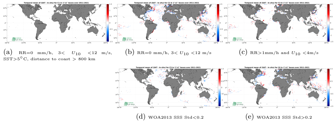
Figure 12: Temporal mean gridded over spatial boxes of size 1^\circ \times 1^\circ of \Delta SSS (SMOS SSS L3 v2 - 9-Days (BEC) - TSG (LEGOS-DM)) for 5 different subdatasets corresponding to:RR=0 mm/h, 3 < U_{10} < 12 m/s, SST >5^\circ\text{C} , distance to coast > 800 km (a), RR=0 mm/h, 3 < U_{10} < 12 m/s (b), RR >1 mm/h and U_{10} < 4 m/s (c), WOA2013 SSS Std <0.2 (d), WOA2013 SSS Std >0.2 (e).
