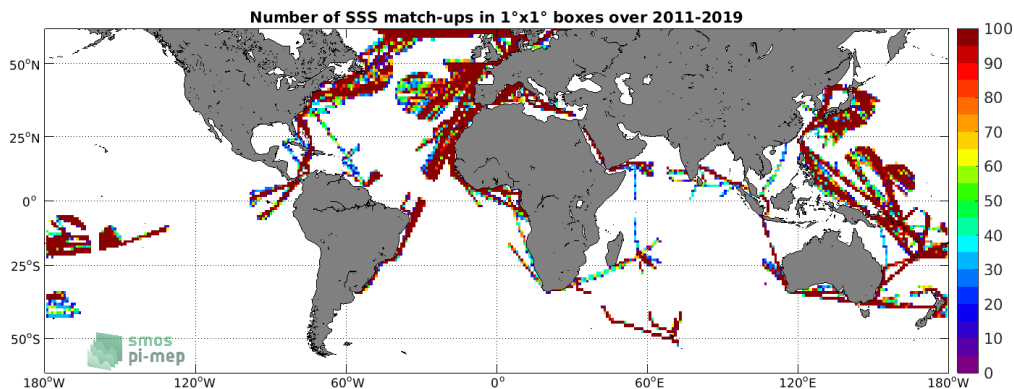
Figure 4: Number of SSS match-ups between TSG (LEGOS-DM) SSS and the SMOS SSS L3 v2 - 9-Days (BEC) SSS product for the SMOS coastal zone (<800km) 60N-60S Pi-MEP region over 1°x1° boxes and for the full satellite product period.
