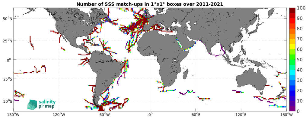
Figure 5: Number of SSS match-ups between TSG (GOSUD-Sailing-ship) SSS and the SMOS SSS L3 v2 - 9-Days (BEC) SSS product for the SMOS coastal zone (<800km) 60N-60S Pi-MEP region over 1^{\circ} \times 1^{\circ} boxes and for the full satellite product period.
