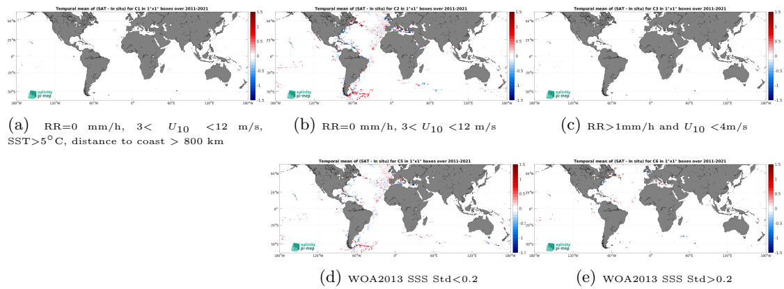
Figure 14: Temporal mean gridded over spatial boxes of size 1^\circ \times 1^\circ of \Delta\text{SSS} (SMOS SSS L3 v2 - 9-Days (BEC) - TSG (GOSUD-Sailing-ship)) for 5 different subdatasets corresponding to:RR=0 mm/h, 3 < U_{10} < 12 m/s, SST >5^\circ\text{C} , distance to coast > 800 km (a), RR=0 mm/h, 3 < U_{10} < 12 m/s (b), RR >1 mm/h and U_{10} < 4 m/s (c), WOA2013 SSS Std <0.2 (d), WOA2013 SSS Std >0.2 (e).
