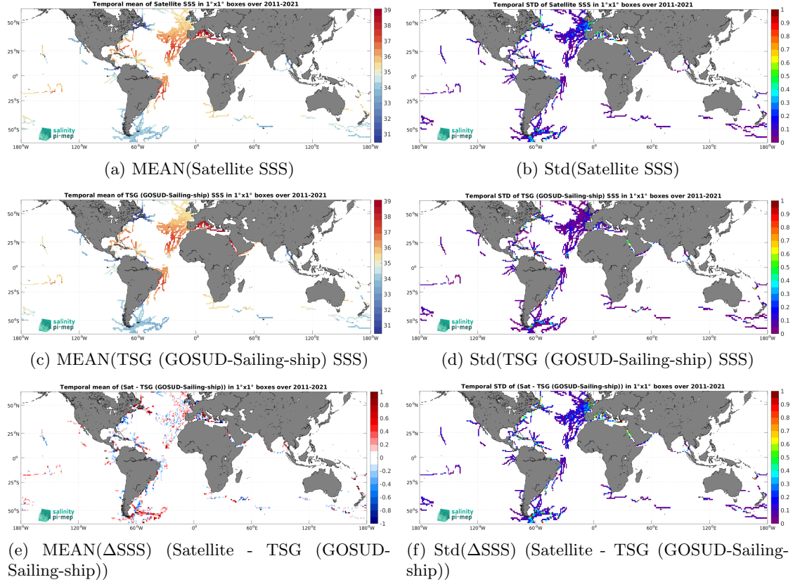
Figure 7: Temporal mean (left) and Std (right) of SSS from SMOS SSS L3 v2 - 9-Days (BEC) (top), TSG (GOSUD-Sailing-ship) (middle), and of \Delta SSS (Satellite - TSG (GOSUD-Sailing-ship)). Only match-up pairs are used to generate these maps.
