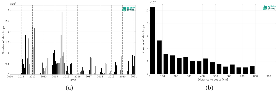
Figure 2: Number of match-ups between TSG (GOSUD-Sailing-ship) and SMOS SSS L3 v2 - 9-Days (BEC) SSS as a function of time (a) and as function of the distance to coast (b) over the SMOS coastal zone (<800km) 60N-60S Pi-MEP region and for the full satellite product period.
