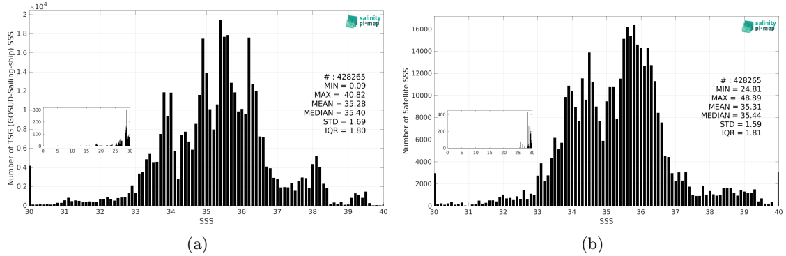
Figure 3: Histograms of SSS from TSG (GOSUD-Sailing-ship) (a) and SMOS SSS L3 v2 - 9-Days (BEC) (b) considering all match-up pairs per bins of 0.1 over the SMOS coastal zone (<800km) 60N-60S Pi-MEP region and for the full satellite product period.
