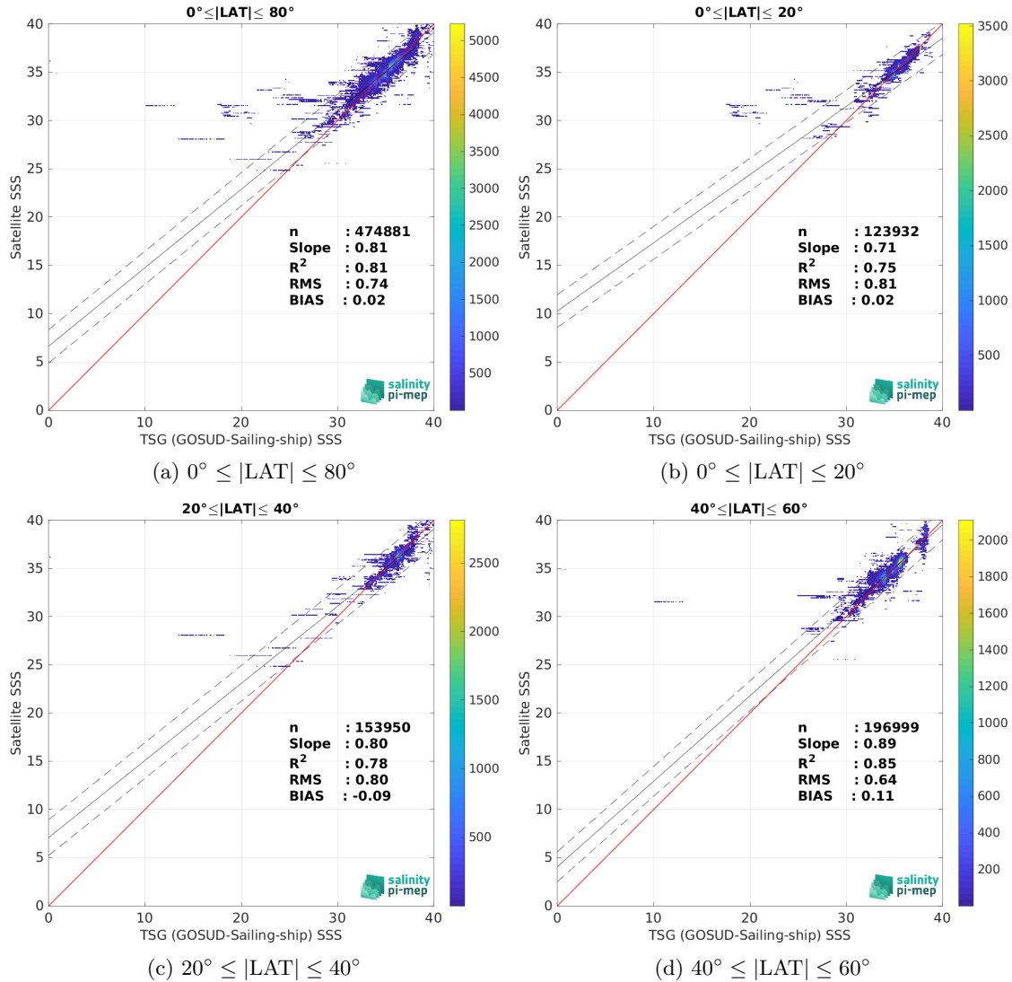
Figure 9: Contour maps of the concentration of SMOS SSS L3 v2 - 9-Days (BEC) SSS (y-axis) versus TSG (GOSUD-Sailing-ship) SSS (x-axis) at match-up pairs for different latitude bands. For each plot, the red line shows x=y . The black thin and dashed lines indicate a linear fit through the data cloud and the \pm 95\% confidence levels, respectively. The number match-up pairs n , the slope and R^2 coefficient of the linear fit, the root mean square (RMS) and the mean bias between satellite and in situ data are indicated for each latitude band in each plots.
