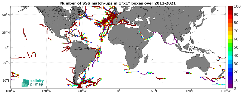
Figure 4: Number of SSS match-ups between TSG (GOSUD-Sailing-ship) SSS and the SMOS SSS L3 v2 - 9-Days (BEC) SSS product for the SMOS coastal zone (<800km) 60N-60S Pi-MEP region over 1^{\circ} \times 1^{\circ} boxes and for the full satellite product period.
