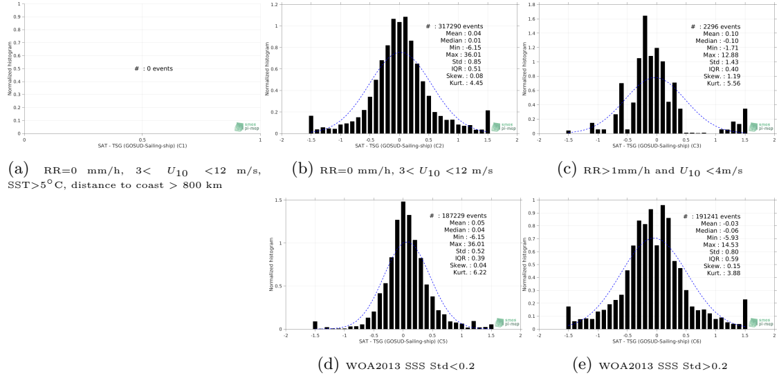
Figure 13: Normalized histogram of \Delta SSS (SMOS SSS L3 v2 - 9-Days (BEC) - TSG (GOSUD-Sailing-ship)) for 5 different subdatasets corresponding to: RR=0 mm/h, 3 < U_{10} < 12 m/s, SST > 5^\circ\text{C} , distance to coast > 800 km (a), RR=0 mm/h, 3 < U_{10} < 12 m/s (b), RR > 1 mm/h and U_{10} < 4 m/s (c), WOA2013 SSS Std < 0.2 (d), WOA2013 SSS Std > 0.2 (e).
