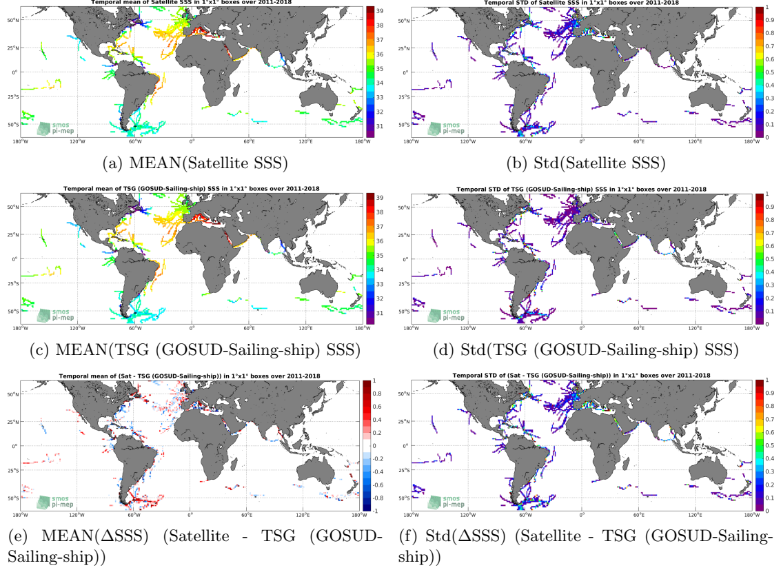
Figure 6: Temporal mean (left) and Std (right) of SSS from SMOS SSS L3 v2 - 9-Days (BEC) (top), TSG (GOSUD-Sailing-ship) (middle), and of \Delta\text{SSS} (Satellite - TSG (GOSUD-Sailing-ship)). Only match-up pairs are used to generate these maps.
