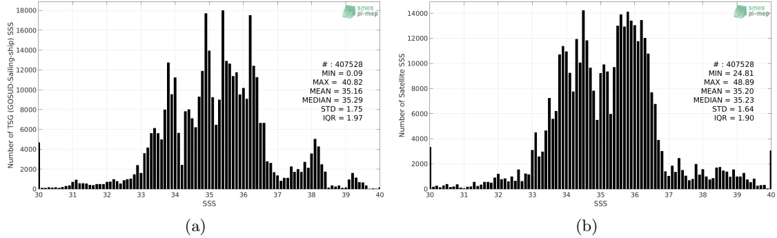
Figure 2: Histograms of SSS from TSG (GOSUD-Sailing-ship) (a) and SMOS SSS L3 v2 - 9-Days (BEC) (b) considering all match-up pairs per bins of 0.1 over the SMOS coastal zone (<800km) 60N-60S Pi-MEP region and for the full satellite product period.
