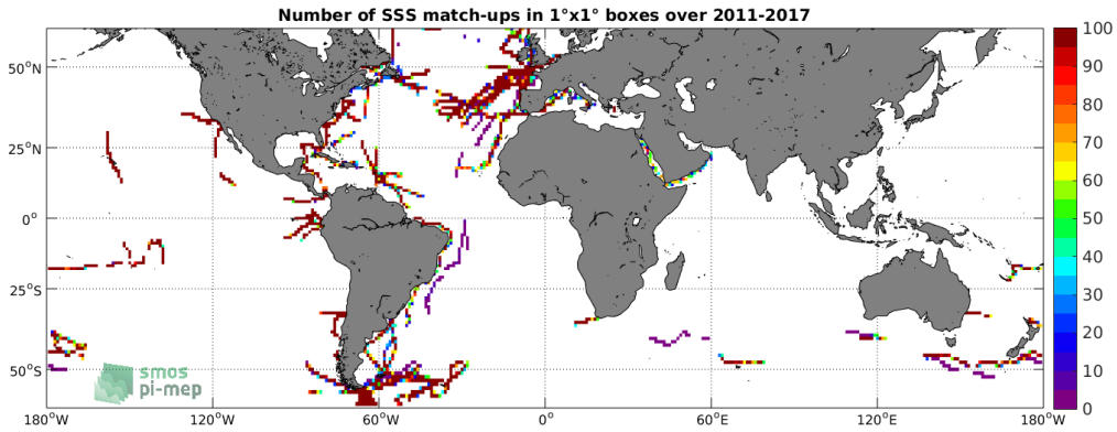
Figure 4: Number of SSS match-ups between TSG (GOSUD-Sailing-ship) SSS and the SMOS L3 v2 - 9-Days (BEC) SSS product for the SMOS coastal zone (<800km) 60N-60S Pi-MEP region over 1°x1° boxes and for the full satellite product period.
