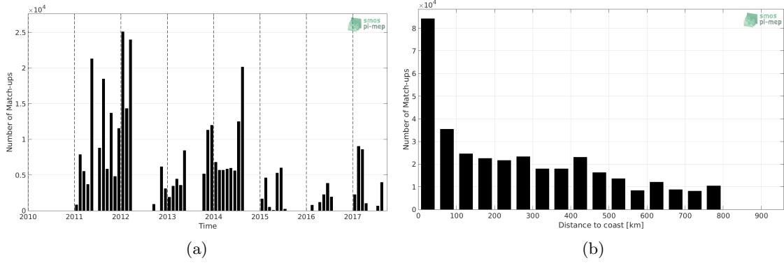
Figure 1: Number of match-ups between TSG (GOSUD-Sailing-ship) and SMOS L3 v2 - 9-Days (BEC) SSS as a function of time (a) and as function of the distance to coast (b) over the SMOS coastal zone (<800km) 60N-60S Pi-MEP region and for the full satellite product period.
