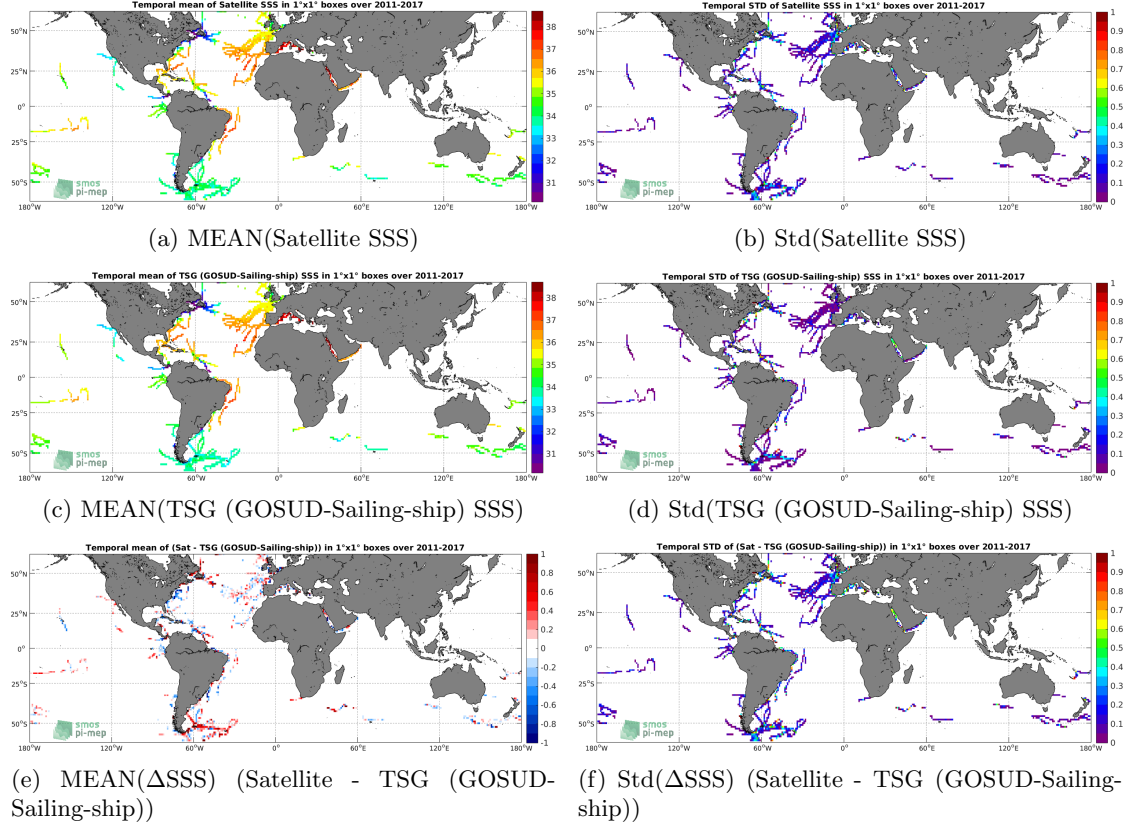
Figure 6: Temporal mean (left) and Std (right) of SSS from SMOS L3 v2 - 9-Days (BEC) (top), TSG (GOSUD-Sailing-ship) (middle), and of \Delta SSS (Satellite - TSG (GOSUD-Sailing-ship)). Only match-up pairs are used to generate these maps.
