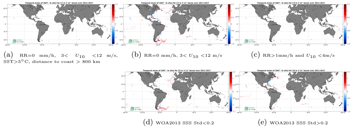
Figure 12: Temporal mean gridded over spatial boxes of size 1^\circ \times 1^\circ of \Delta SSS (SMOS L3 v2 - 9-Days (BEC) - TSG (GOSUD-Sailing-ship)) for 5 different subdatasets corresponding to: RR=0 mm/h, 3 < U_{10} < 12 m/s, SST > 5^\circ C , distance to coast > 800 km (a), RR=0 mm/h, 3 < U_{10} < 12 m/s (b), RR > 1 mm/h and U_{10} < 4 m/s (c), WOA2013 SSS Std < 0.2 (d), WOA2013 SSS Std > 0.2 (e).
