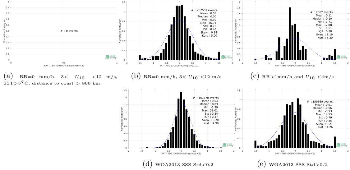
Figure 13: Normalized histogram of \Delta\text{SSS} (SMOS L3 v2 - 9-Days (BEC) - TSG (GOSUD-Sailing-ship)) for 5 different subdatasets corresponding to: RR=0 mm/h, 3 < U_{10} < 12 m/s, SST > 5^\circ\text{C} , distance to coast > 800 km (a), RR=0 mm/h, 3 < U_{10} < 12 m/s (b), RR > 1\text{mm/h} and U_{10} < 4\text{m/s} (c), WOA2013 SSS Std < 0.2 (d), WOA2013 SSS Std > 0.2 (e).
