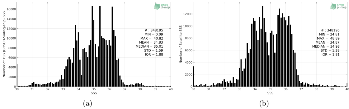
Figure 2: Histograms of SSS from TSG (GOSUD-Sailing-ship) (a) and SMOS L3 v2 - 9-Days (BEC) (b) considering all match-up pairs per bins of 0.1 over the SMOS coastal zone (<800km) 60N-60S Pi-MEP region and for the full satellite product period.
