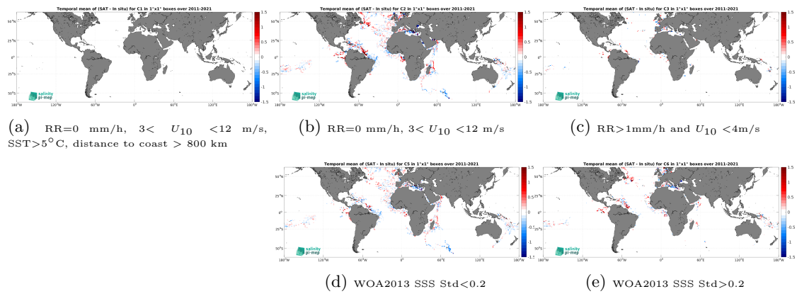
Figure 14: Temporal mean gridded over spatial boxes of size 1^\circ \times 1^\circ of \Delta\text{SSS} (SMOS SSS L3 v2 - 9-Days (BEC) - TSG (GOSUD-Research-vessel)) for 5 different subdatasets corresponding to:RR=0 mm/h, 3 < U_{10} < 12 m/s, SST > 5^\circ\text{C} , distance to coast > 800 km (a), RR=0 mm/h, 3 < U_{10} < 12 m/s (b), RR > 1 mm/h and U_{10} < 4 m/s (c), WOA2013 SSS Std < 0.2 (d), WOA2013 SSS Std > 0.2 (e).
