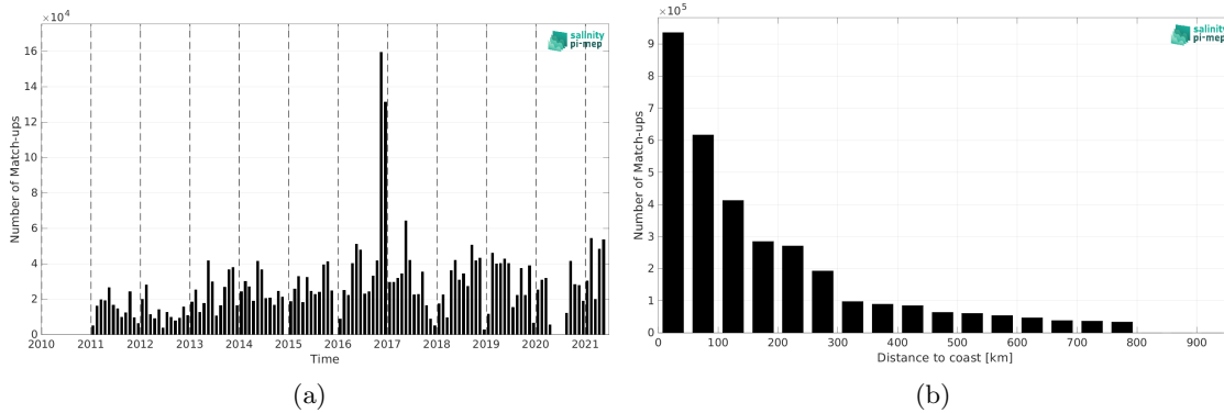
Figure 2: Number of match-ups between TSG (GOSUD-Research-vessel) and SMOS SSS L3 v2 - 9-Days (BEC) SSS as a function of time (a) and as function of the distance to coast (b) over the SMOS coastal zone (<800km) 60N-60S Pi-MEP region and for the full satellite product period.
