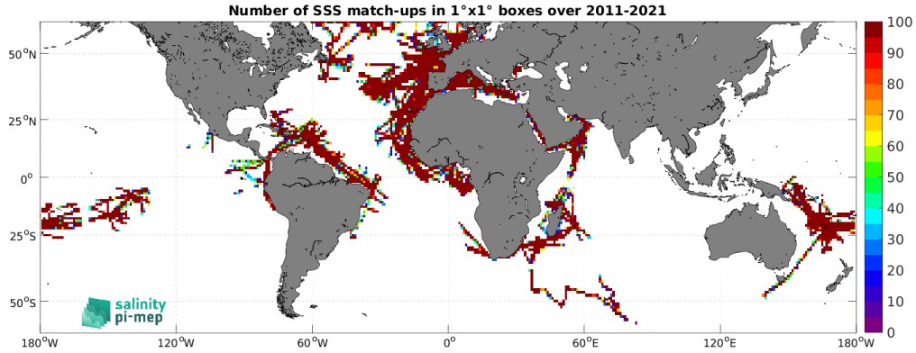
Figure 5: Number of SSS match-ups between TSG (GOSUD-Research-vessel) SSS and the SMOS SSS L3 v2 - 9-Days (BEC) SSS product for the SMOS coastal zone (<800km) 60N-60S Pi-MEP region over 1^{\circ} \times 1^{\circ} boxes and for the full satellite product period.
