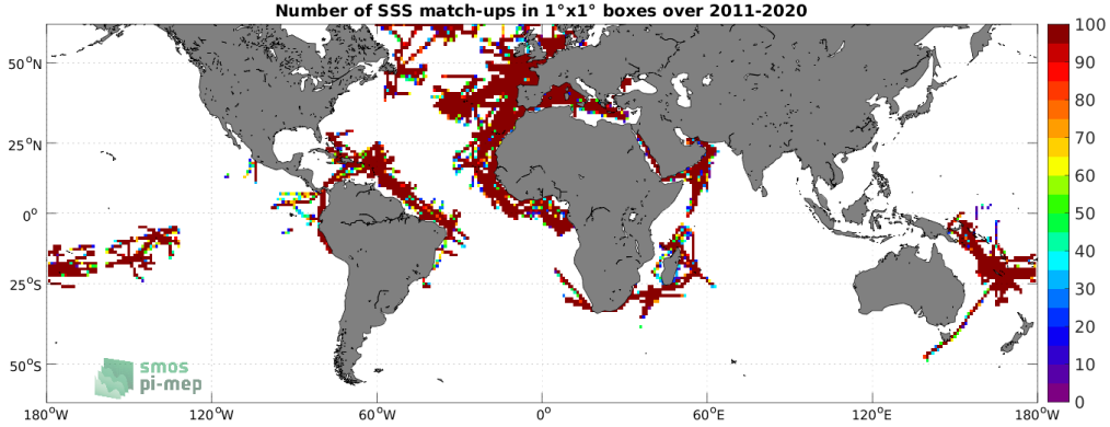
Figure 4: Number of SSS match-ups between TSG (GOSUD-Research-vessel) SSS and the SMOS SSS L3 v2 - 9-Days (BEC) SSS product for the SMOS coastal zone (<800km) 60N-60S Pi-MEP region over 1^{\circ} \times 1^{\circ} boxes and for the full satellite product period.
