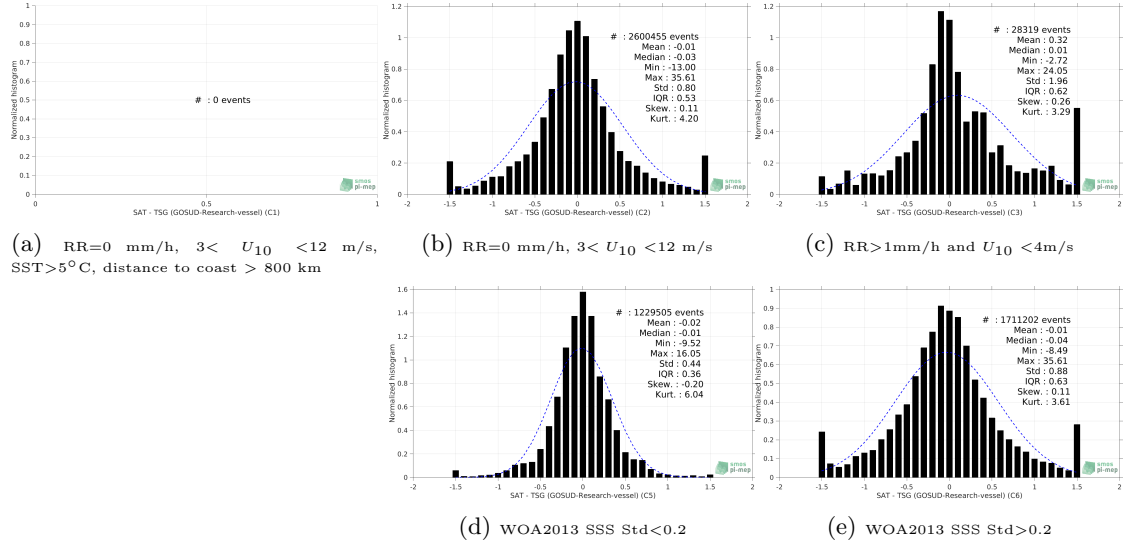
Figure 13: Normalized histogram of \Delta SSS (SMOS SSS L3 v2 - 9-Days (BEC) - TSG (GOSUD-Research-vessel)) for 5 different subdatasets corresponding to: RR=0 mm/h, 3 < U_{10} < 12 m/s, SST > 5^\circ C , distance to coast > 800 km (a), RR=0 mm/h, 3 < U_{10} < 12 m/s (b), RR > 1 mm/h and U_{10} < 4 m/s (c), WOA2013 SSS Std < 0.2 (d), WOA2013 SSS Std > 0.2 (e).
