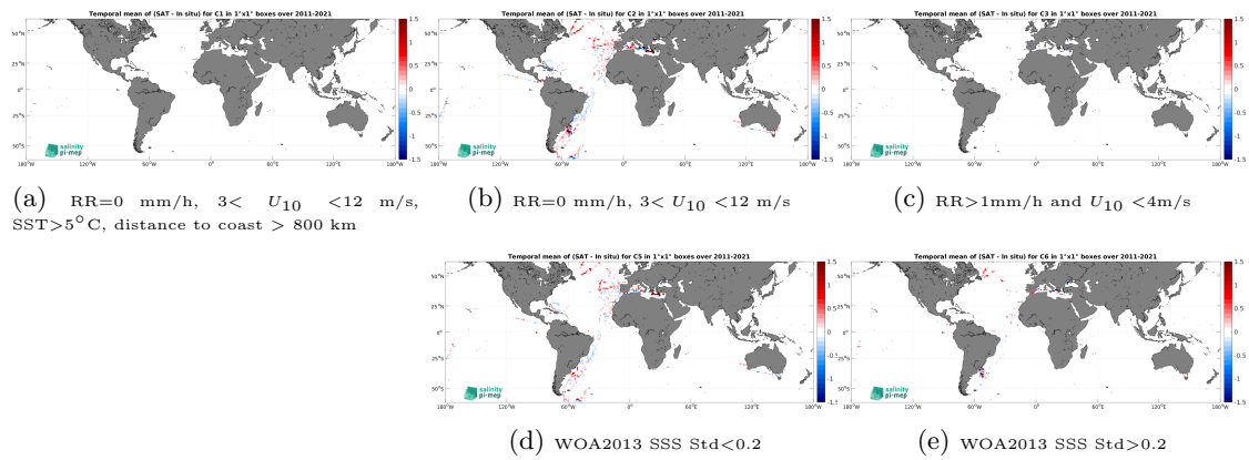
Figure 14: Temporal mean gridded over spatial boxes of size 1^\circ \times 1^\circ of \Delta SSS (SMOS SSS L3 v2 - 9-Days (BEC) - TSG (CSIC-UTM)) for 5 different subdatasets corresponding to:RR=0 mm/h, 3 < U_{10} < 12 m/s, SST >5^\circ\text{C} , distance to coast > 800 km (a), RR=0 mm/h, 3 < U_{10} < 12 m/s (b), RR >1 mm/h and U_{10} < 4 m/s (c), WOA2013 SSS Std <0.2 (d), WOA2013 SSS Std >0.2 (e).
