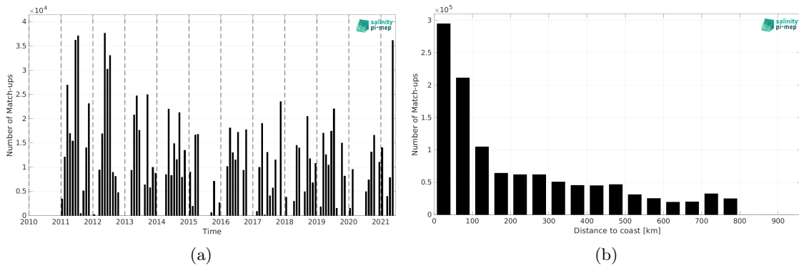
Figure 2: Number of match-ups between TSG (CSIC-UTM) and SMOS SSS L3 v2 - 9-Days (BEC) SSS as a function of time (a) and as function of the distance to coast (b) over the SMOS coastal zone (<800km) 60N-60S Pi-MEP region and for the full satellite product period.
