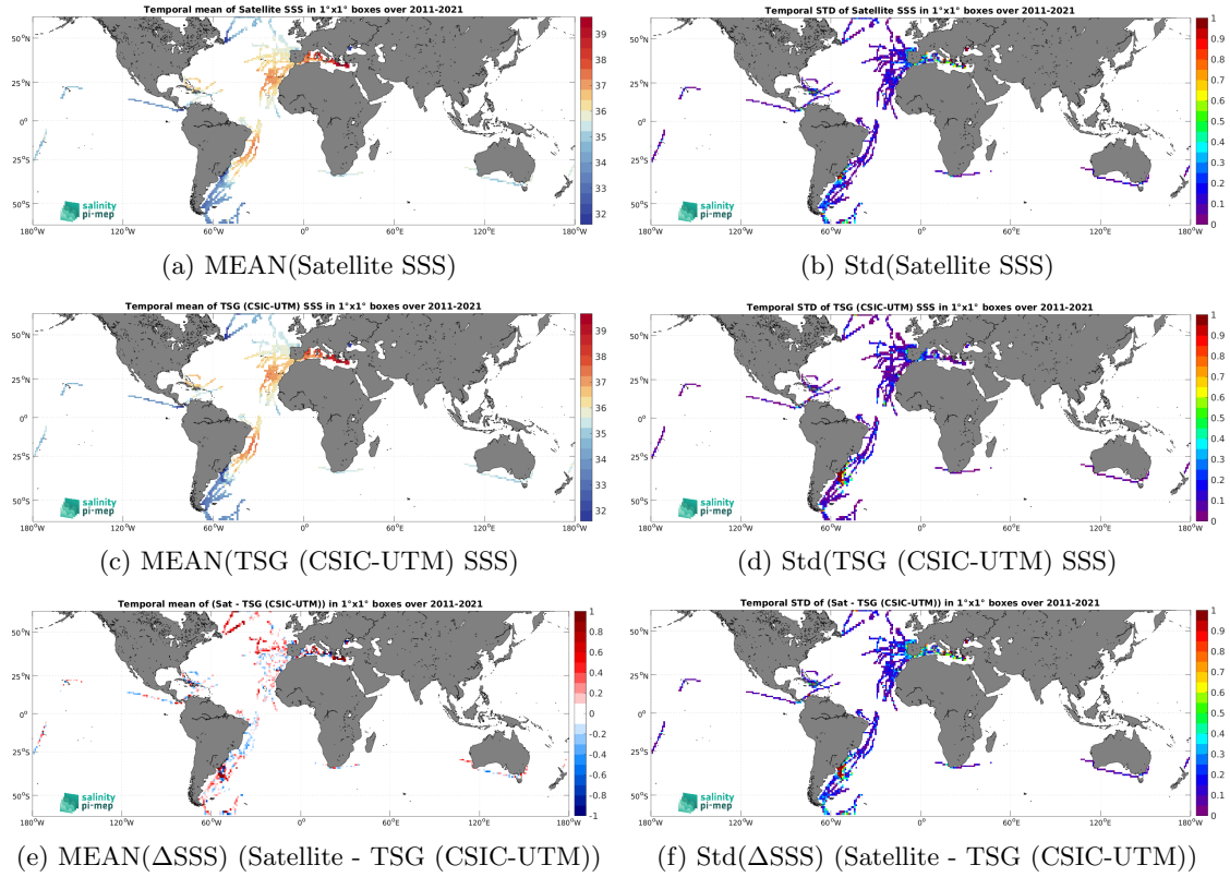
Figure 7: Temporal mean (left) and Std (right) of SSS from SMOS SSS L3 v2 - 9-Days (BEC) (top), TSG (CSIC-UTM) (middle), and of \Delta SSS (Satellite - TSG (CSIC-UTM)). Only match-up pairs are used to generate these maps.
