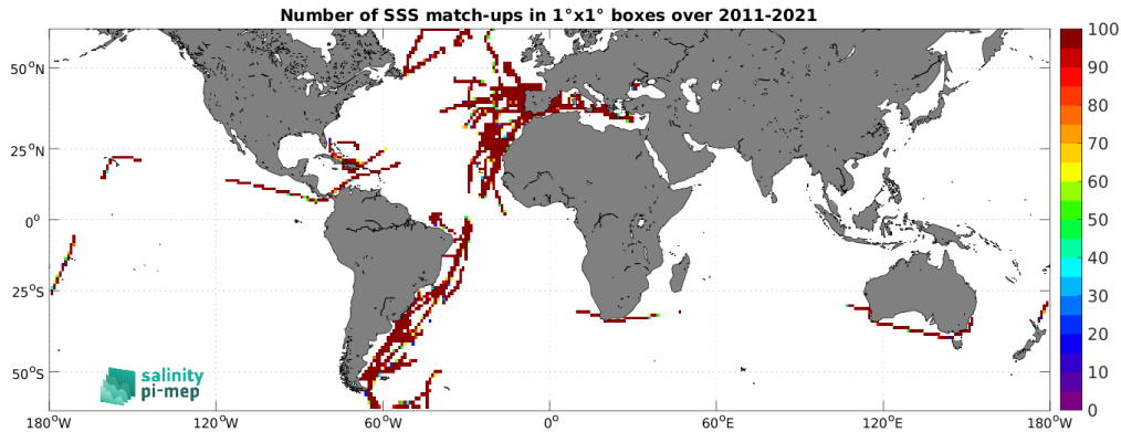
Figure 5: Number of SSS match-ups between TSG (CSIC-UTM) SSS and the SMOS SSS L3 v2 - 9-Days (BEC) SSS product for the SMOS coastal zone (<800km) 60N-60S Pi-MEP region over 1^\circ \times 1^\circ boxes and for the full satellite product period.
