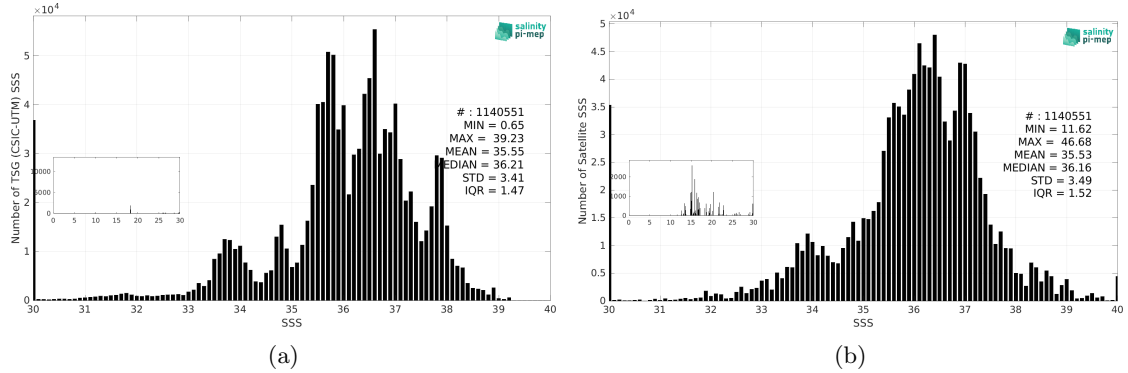
Figure 3: Histograms of SSS from TSG (CSIC-UTM) (a) and SMOS SSS L3 v2 - 9-Days (BEC) (b) considering all match-up pairs per bins of 0.1 over the SMOS coastal zone (<800km) 60N-60S Pi-MEP region and for the full satellite product period.
