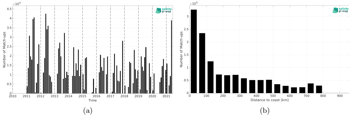
Figure 1: Number of match-ups between TSG (CSIC-UTM) and SMOS SSS L3 v2 - 9-Days (BEC) SSS as a function of time (a) and as function of the distance to coast (b) over the SMOS coastal zone ( < 800\text{km} ) 60N-60S Pi-MEP region and for the full satellite product period.
