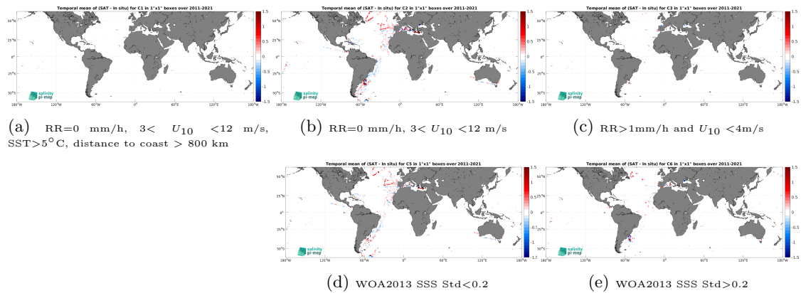
Figure 12: Temporal mean gridded over spatial boxes of size 1^\circ \times 1^\circ of \Delta\text{SSS} (SMOS SSS L3 v2 - 9-Days (BEC) - TSG (CSIC-UTM)) for 5 different subdatasets corresponding to:RR=0 mm/h, 3 < U_{10} < 12 m/s, SST >5^\circ\text{C} , distance to coast > 800 km (a), RR=0 mm/h, 3 < U_{10} < 12 m/s (b), RR >1 mm/h and U_{10} < 4 m/s (c), WOA2013 SSS Std <0.2 (d), WOA2013 SSS Std >0.2 (e).
