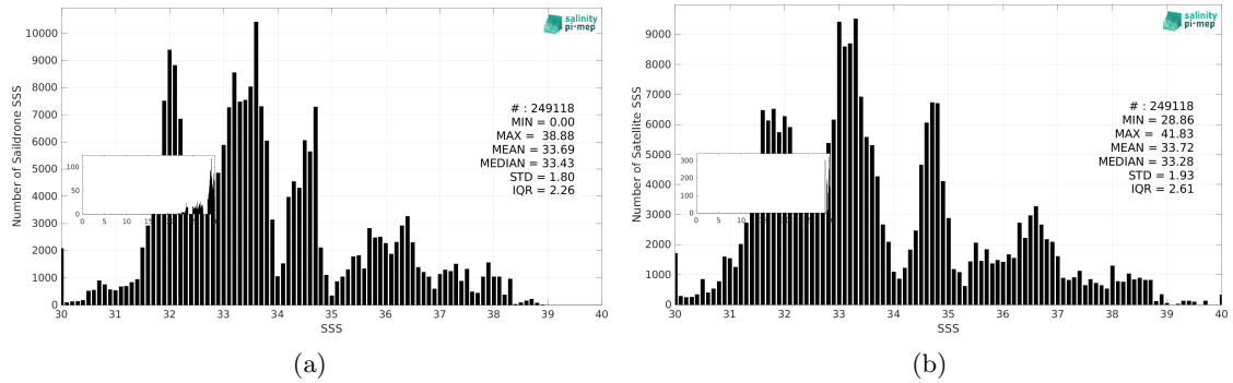
Figure 3: Histograms of SSS from Saildrone (a) and SMOS SSS L3 v2 - 9-Days (BEC) (b) considering all match-up pairs per bins of 0.1 over the SMOS coastal zone (<800km) 60N-60S Pi-MEP region and for the full satellite product period.
