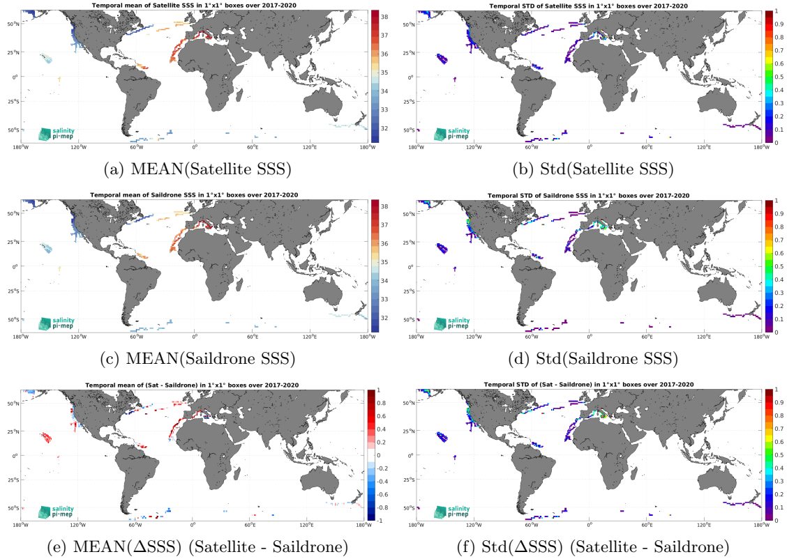
Figure 7: Temporal mean (left) and Std (right) of SSS from SMOS SSS L3 v2 - 9-Days (BEC) (top), Saildrone (middle), and of \Delta SSS (Satellite - Saildrone). Only match-up pairs are used to generate these maps.
