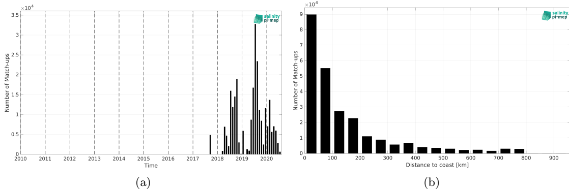
Figure 2: Number of match-ups between Saildrone and SMOS SSS L3 v2 - 9-Days (BEC) SSS as a function of time (a) and as function of the distance to coast (b) over the SMOS coastal zone (<800km) 60N-60S Pi-MEP region and for the full satellite product period.
