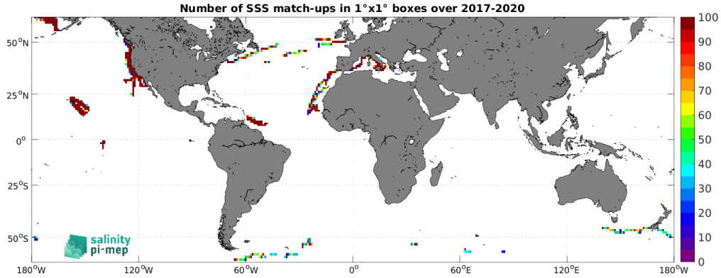
Figure 5: Number of SSS match-ups between Saildrone SSS and the SMOS SSS L3 v2 - 9-Days (BEC) SSS product for the SMOS coastal zone (<800km) 60N-60S Pi-MEP region over 1^\circ \times 1^\circ boxes and for the full satellite product period.
