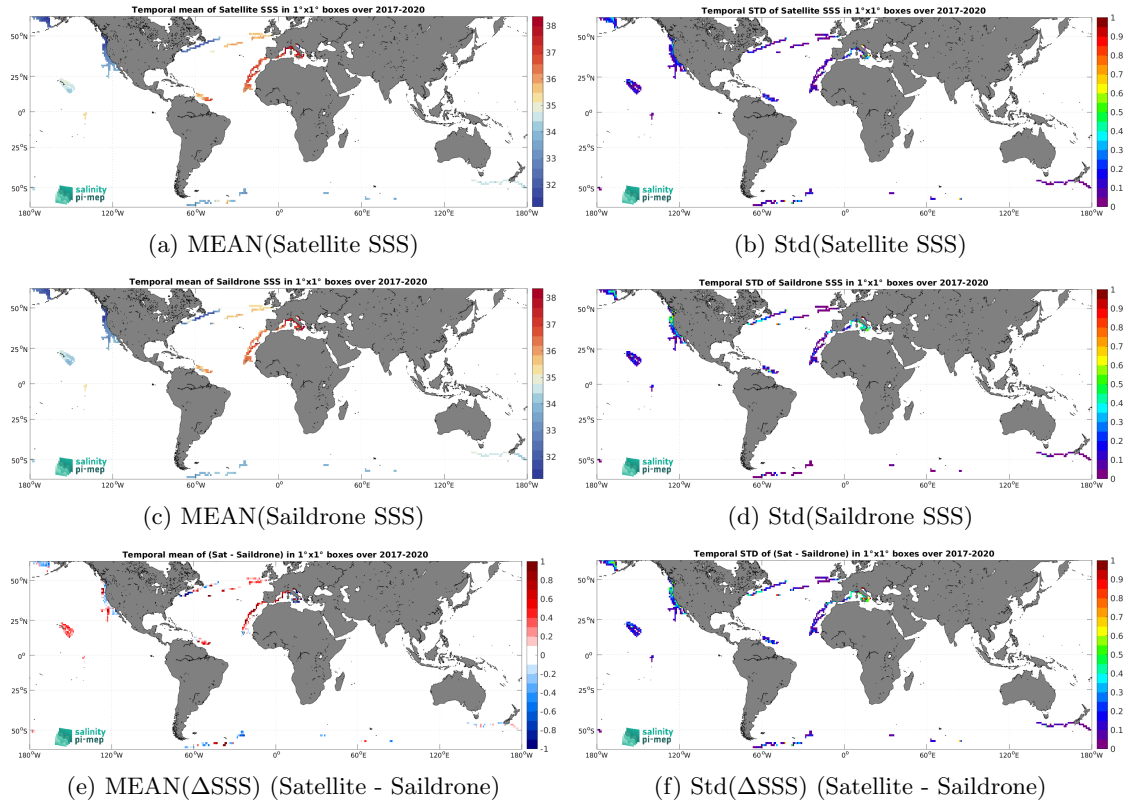
Figure 6: Temporal mean (left) and Std (right) of SSS from SMOS SSS L3 v2 - 9-Days (BEC) (top), Saildrone (middle), and of \Delta SSS (Satellite - Saildrone). Only match-up pairs are used to generate these maps.
