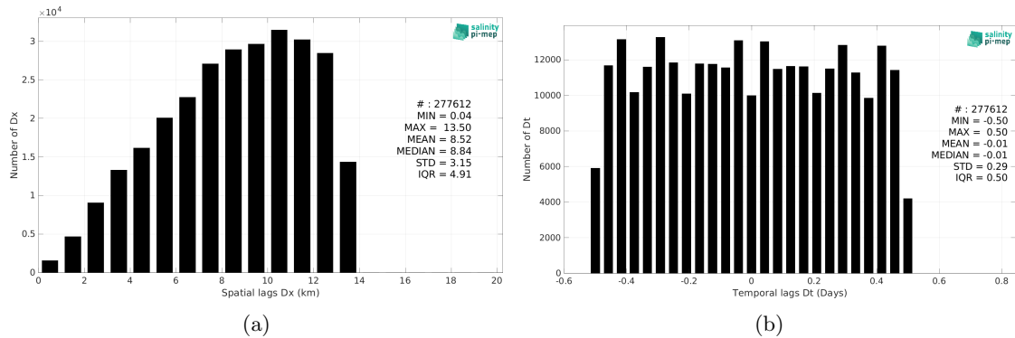
Figure 5: Histograms of the spatial (a) and temporal (b) lags between the location/time of the Saildrone measurement and the date of the corresponding SMOS SSS L3 v2 - 9-Days (BEC) SSS pixel.
