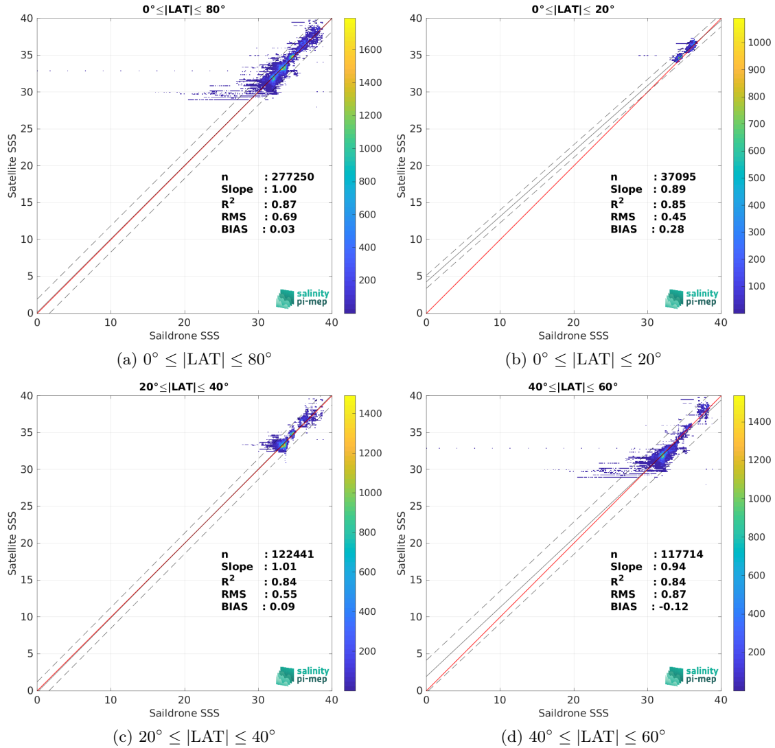
Figure 9: Contour maps of the concentration of SMOS SSS L3 v2 - 9-Days (BEC) SSS (y-axis) versus Saildrone SSS (x-axis) at match-up pairs for different latitude bands. For each plot, the red line shows x=y . The black thin and dashed lines indicate a linear fit through the data cloud and the \pm 95\% confidence levels, respectively. The number match-up pairs n , the slope and R^2 coefficient of the linear fit, the root mean square (RMS) and the mean bias between satellite and in situ data are indicated for each latitude band in each plots.
