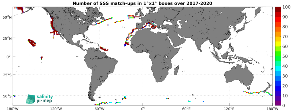
Figure 4: Number of SSS match-ups between Saildrone SSS and the SMOS SSS L3 v2 - 9-Days (BEC) SSS product for the SMOS coastal zone (<800km) 60N-60S Pi-MEP region over 1^\circ \times 1^\circ boxes and for the full satellite product period.
