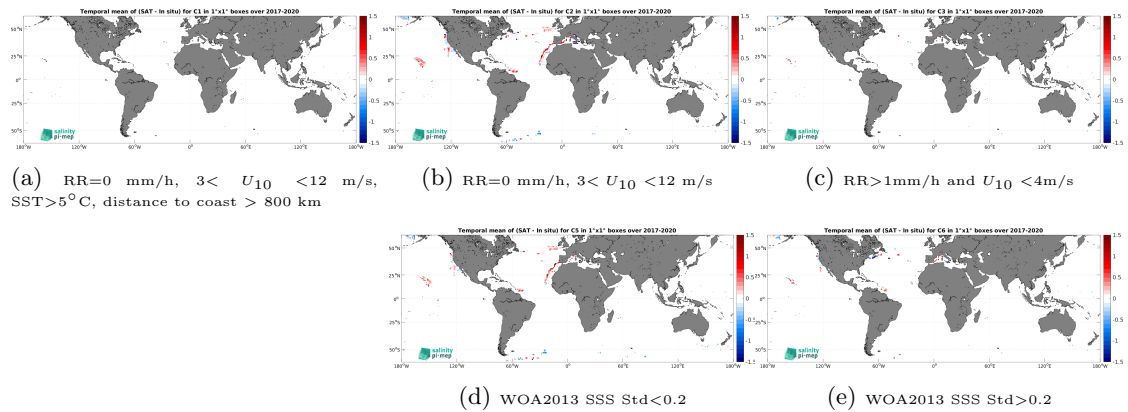
Figure 12: Temporal mean gridded over spatial boxes of size 1^\circ \times 1^\circ of \Delta\text{SSS} (SMOS SSS L3 v2 - 9-Days (BEC) - Saildrone) for 5 different subdatasets corresponding to:RR=0 mm/h, 3 < U_{10} < 12 m/s, SST >5^\circ\text{C} , distance to coast > 800 km (a), RR=0 mm/h, 3 < U_{10} < 12 m/s (b), RR >1 mm/h and U_{10} < 4 m/s (c), WOA2013 SSS Std <0.2 (d), WOA2013 SSS Std >0.2 (e).
