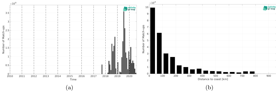
Figure 1: Number of match-ups between Saildrone and SMOS SSS L3 v2 - 9-Days (BEC) SSS as a function of time (a) and as function of the distance to coast (b) over the SMOS coastal zone (<800km) 60N-60S Pi-MEP region and for the full satellite product period.
