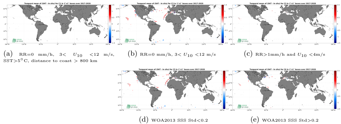
Figure 12: Temporal mean gridded over spatial boxes of size 1^\circ \times 1^\circ of \Delta SSS (SMOS SSS L3 v2 - 9-Days (BEC) - Saildrone) for 5 different subdatasets corresponding to:RR=0 mm/h, 3 < U_{10} < 12 m/s, SST >5^\circ\text{C} , distance to coast > 800 km (a), RR=0 mm/h, 3 < U_{10} < 12 m/s (b), RR >1 mm/h and U_{10} < 4 m/s (c), WOA2013 SSS Std <0.2 (d), WOA2013 SSS Std >0.2 (e).
