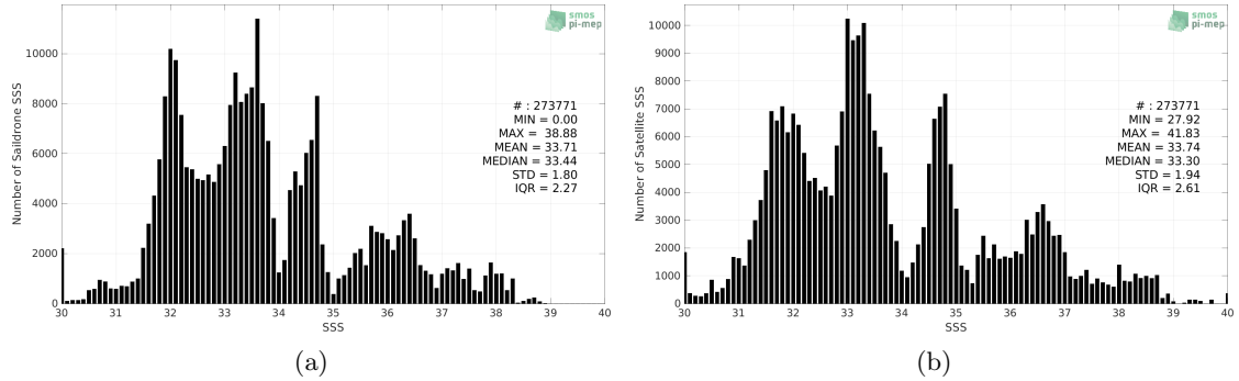
Figure 2: Histograms of SSS from Saildrone (a) and SMOS SSS L3 v2 - 9-Days (BEC) (b) considering all match-up pairs per bins of 0.1 over the SMOS coastal zone (<800km) 60N-60S Pi-MEP region and for the full satellite product period.
