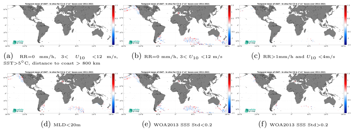
Figure 14: Temporal mean gridded over spatial boxes of size 1^\circ \times 1^\circ of \Delta SSS (SMOS SSS L3 v2 - 9-Days (BEC) - Marine mammals) for 6 different subdatasets corresponding to: RR=0 mm/h, 3 < U_{10} < 12 m/s, SST > 5°C, distance to coast > 800 km (a), RR=0 mm/h, 3 < U_{10} < 12 m/s (b), RR > 1mm/h and U_{10} < 4 m/s (c), MLD < 20m (d), WOA2013 SSS Std < 0.2 (e), WOA2013 SSS Std > 0.2 (f).
