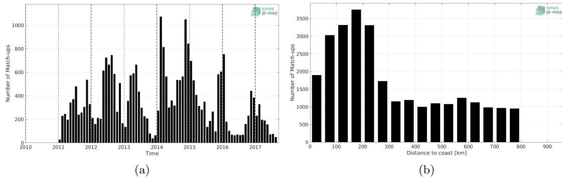
Figure 1: Number of match-ups between Sea mammals and SMOS SSS L3 v2 - 9-Days (BEC) SSS as a function of time (a) and as function of the distance to coast (b) over the SMOS coastal zone (<800km) 60N-60S Pi-MEP region and for the full satellite product period.
