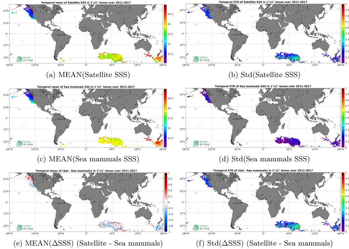
Figure 6: Temporal mean (left) and Std (right) of SSS from SMOS SSS L3 v2 - 9-Days (BEC) (top), Sea mammals (middle), and of \Delta SSS (Satellite - Sea mammals). Only match-up pairs are used to generate these maps.
