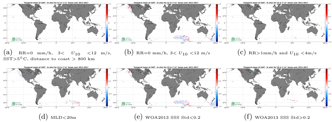
Figure 12: Temporal mean gridded over spatial boxes of size 1^\circ \times 1^\circ of \Delta SSS (SMOS SSS L3 v2 - 9-Days (BEC) - Sea mammals) for 6 different subdatasets corresponding to: RR=0 mm/h, 3 < U_{10} < 12 m/s, SST > 5°C, distance to coast > 800 km (a), RR=0 mm/h, 3 < U_{10} < 12 m/s (b), RR > 1mm/h and U_{10} < 4 m/s (c), MLD < 20m (d), WOA2013 SSS Std < 0.2 (e), WOA2013 SSS Std > 0.2 (f).
