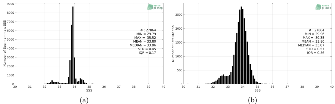
Figure 2: Histograms of SSS from Sea mammals (a) and SMOS SSS L3 v2 - 9-Days (BEC) (b) considering all match-up pairs per bins of 0.1 over the SMOS coastal zone (<800km) 60N-60S Pi-MEP region and for the full satellite product period.
