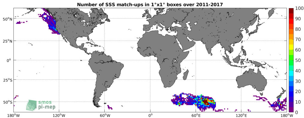
Figure 4: Number of SSS match-ups between Sea mammals SSS and the SMOS SSS L3 v2 - 9-Days (BEC) SSS product for the SMOS coastal zone (<800km) 60N-60S Pi-MEP region over 1°x1° boxes and for the full satellite product period.
