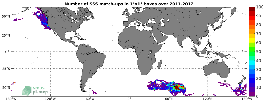
Figure 4: Number of SSS match-ups between Sea mammals SSS and the SMOS SSS L3 v2 - 9-Days (BEC) SSS product for the SMOS coastal zone (<800km) 60N-60S Pi-MEP region over 1^\circ \times 1^\circ boxes and for the full satellite product period.
