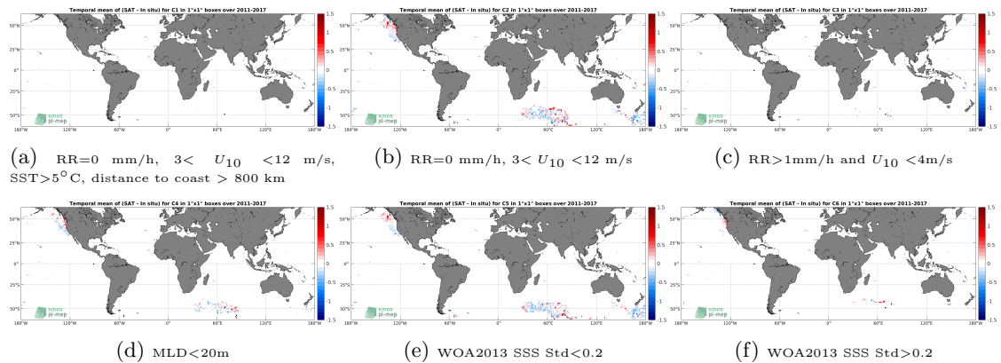
Figure 12: Temporal mean gridded over spatial boxes of size 1^\circ \times 1^\circ of \Delta SSS (SMOS SSS L3 v2 - 9-Days (BEC) - Sea mammals) for 6 different subdatasets corresponding to:RR=0 mm/h, 3 < U_{10} < 12 m/s, SST > 5^\circ\text{C} , distance to coast > 800 km (a), RR=0 mm/h, 3 < U_{10} < 12 m/s (b), RR > 1 mm/h and U_{10} < 4 m/s (c),MLD < 20 m (d),WOA2013 SSS Std < 0.2 (e),WOA2013 SSS Std > 0.2 (f).
