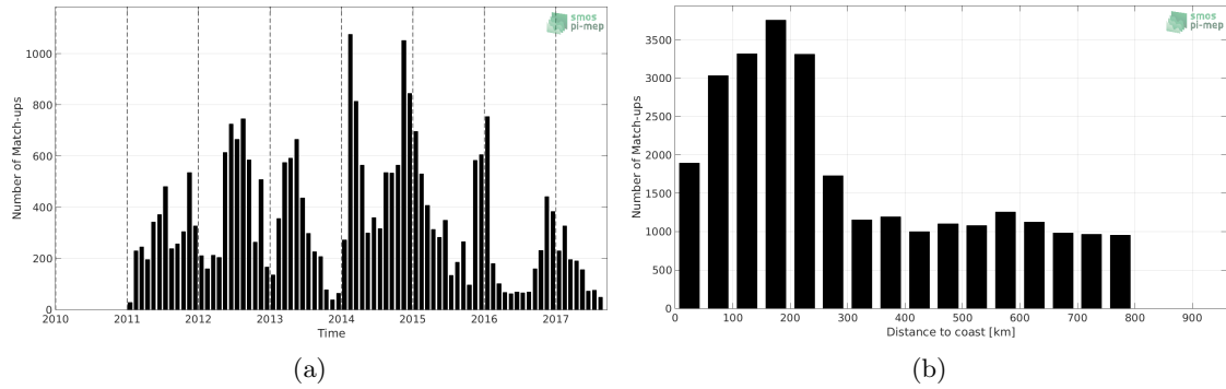
Figure 1: Number of match-ups between Sea mammals and SMOS L3 v2 - 9-Days (BEC) SSS as a function of time (a) and as function of the distance to coast (b) over the SMOS coastal zone (<800km) 60N-60S Pi-MEP region and for the full satellite product period.
