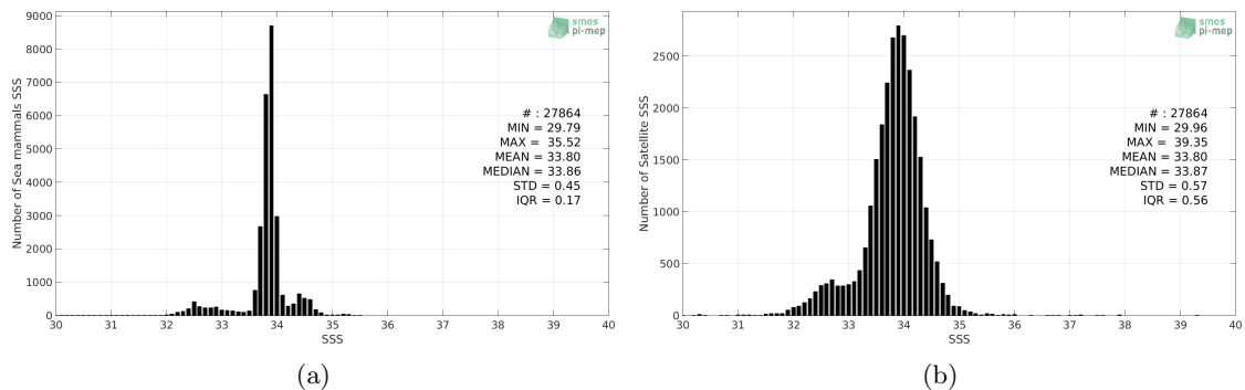
Figure 2: Histograms of SSS from Sea mammals (a) and SMOS L3 v2 - 9-Days (BEC) (b) considering all match-up pairs per bins of 0.1 over the SMOS coastal zone (<800km) 60N-60S Pi-MEP region and for the full satellite product period.
