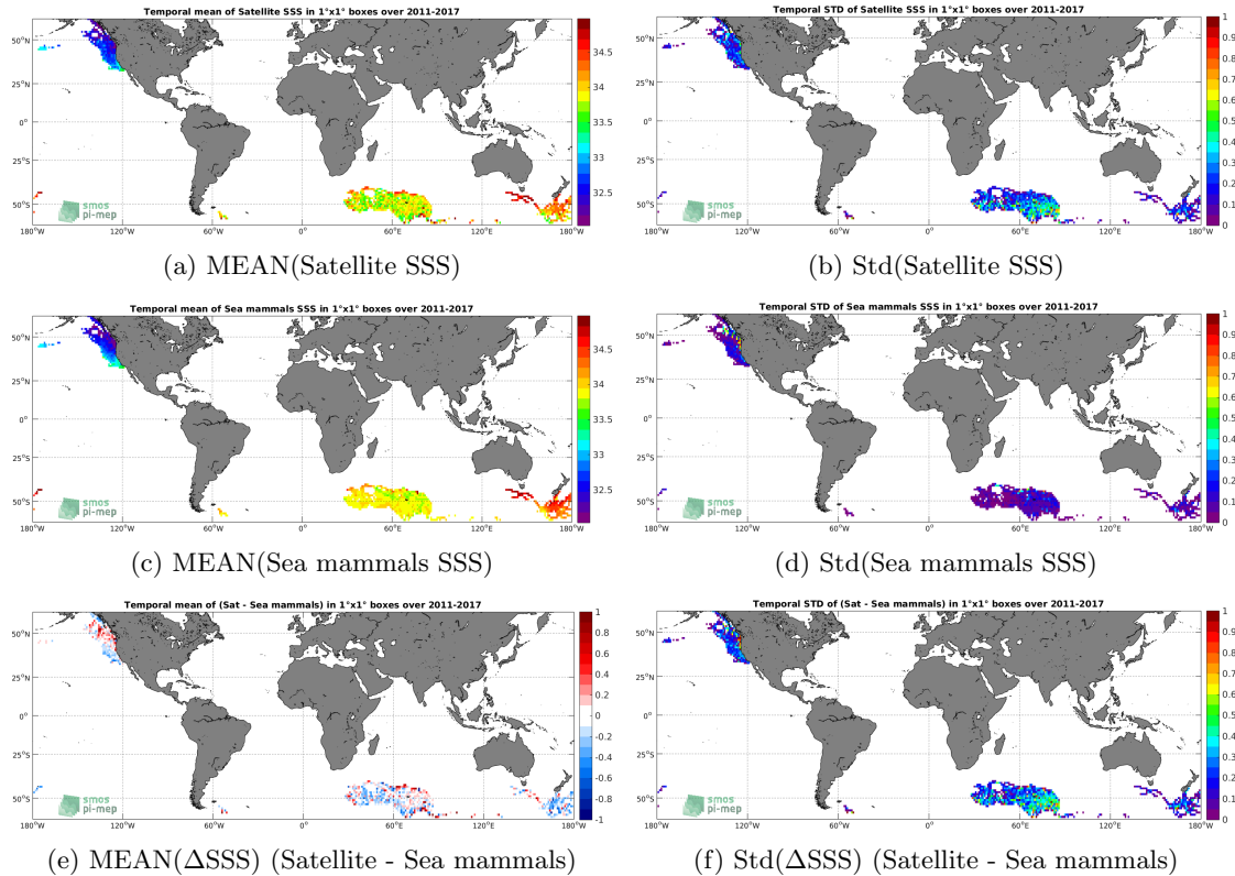
Figure 6: Temporal mean (left) and Std (right) of SSS from SMOS L3 v2 - 9-Days (BEC) (top), Sea mammals (middle), and of \Delta SSS (Satellite - Sea mammals). Only match-up pairs are used to generate these maps.
