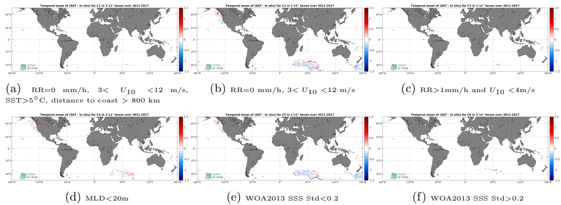
Figure 12: Temporal mean gridded over spatial boxes of size 1^\circ \times 1^\circ of \Delta SSS (SMOS L3 v2 - 9-Days (BEC) - Sea mammals) for 6 different subdatasets corresponding to:RR=0 mm/h, 3 < U_{10} < 12 m/s, SST >5^\circ\text{C} , distance to coast > 800 km (a), RR=0 mm/h, 3 < U_{10} < 12 m/s (b), RR >1 mm/h and U_{10} < 4 m/s (c),MLD <20 m (d),WOA2013 SSS Std <0.2 (e),WOA2013 SSS Std >0.2 (f).
