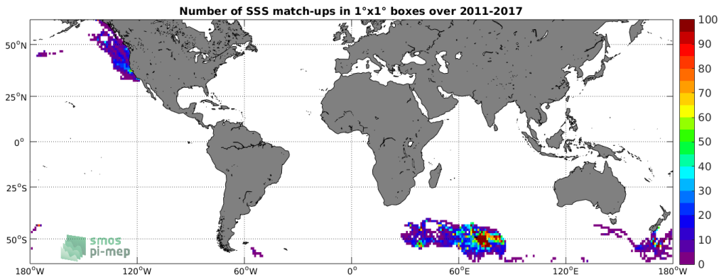
Figure 4: Number of SSS match-ups between Sea mammals SSS and the SMOS L3 v2 - 9-Days (BEC) SSS product for the SMOS coastal zone (<800km) 60N-60S Pi-MEP region over 1°x1° boxes and for the full satellite product period.
