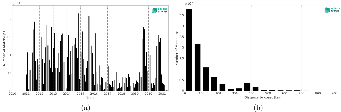
Figure 2: Number of match-ups between ICES and SMOS SSS L3 v2 - 9-Days (BEC) SSS as a function of time (a) and as function of the distance to coast (b) over the SMOS coastal zone (<800km) 60N-60S Pi-MEP region and for the full satellite product period.
