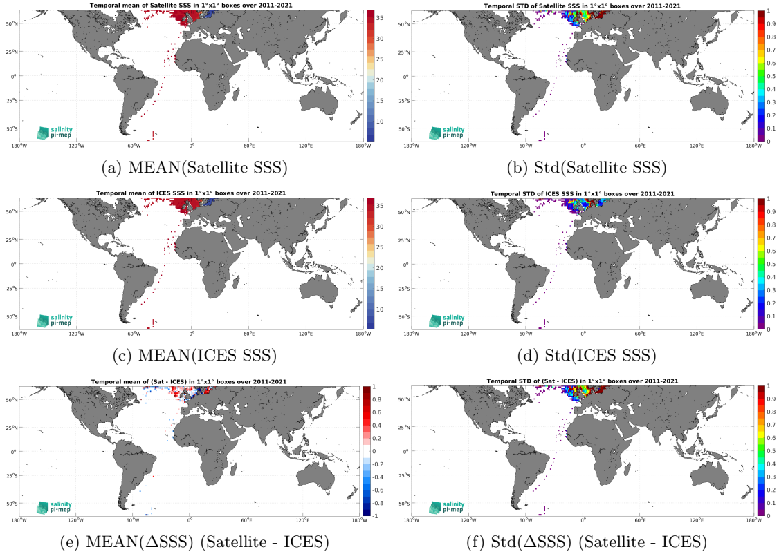
Figure 7: Temporal mean (left) and Std (right) of SSS from SMOS SSS L3 v2 - 9-Days (BEC) (top), ICES (middle), and of \Delta SSS (Satellite - ICES). Only match-up pairs are used to generate these maps.
