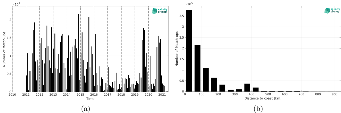
Figure 2: Number of match-ups between ICES and SMOS SSS L3 v2 - 9-Days (BEC) SSS as a function of time (a) and as function of the distance to coast (b) over the SMOS coastal zone ( < 800\text{km} ) 60N-60S Pi-MEP region and for the full satellite product period.
