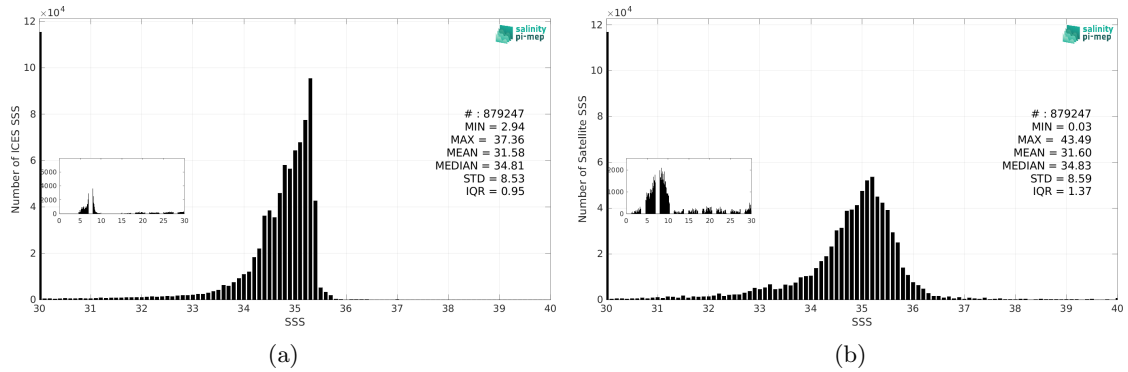
Figure 3: Histograms of SSS from ICES (a) and SMOS SSS L3 v2 - 9-Days (BEC) (b) considering all match-up pairs per bins of 0.1 over the SMOS coastal zone (<800km) 60N-60S Pi-MEP region and for the full satellite product period.
