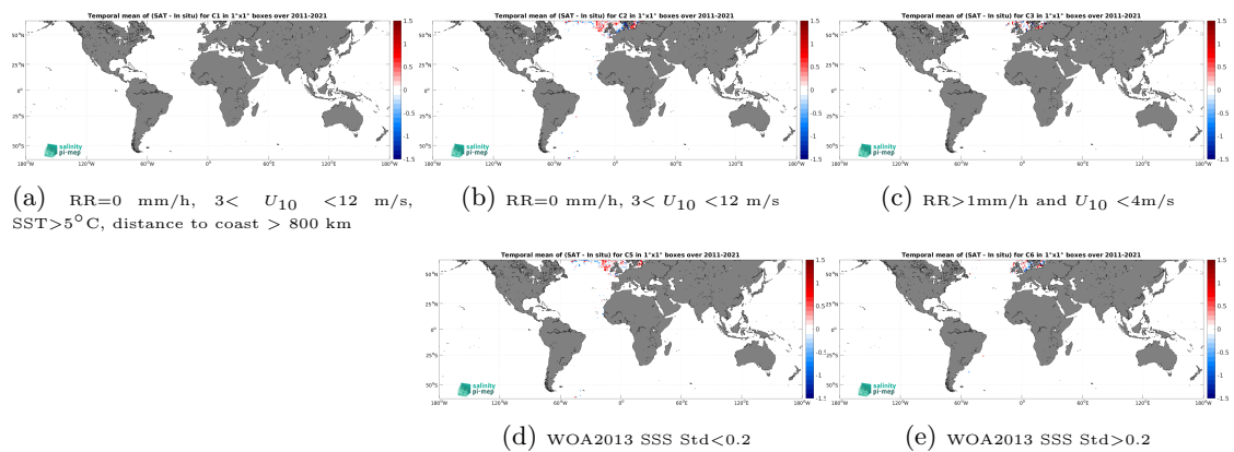
Figure 14: Temporal mean gridded over spatial boxes of size 1^\circ \times 1^\circ of \Delta SSS (SMOS SSS L3 v2 - 9-Days (BEC) - ICES) for 5 different subdatasets corresponding to:RR=0 mm/h, 3 < U_{10} < 12 m/s, SST >5^\circ C, distance to coast > 800 km (a), RR=0 mm/h, 3 < U_{10} < 12 m/s (b), RR >1 mm/h and U_{10} < 4 m/s (c), WOA2013 SSS Std <0.2 (d), WOA2013 SSS Std >0.2 (e).
