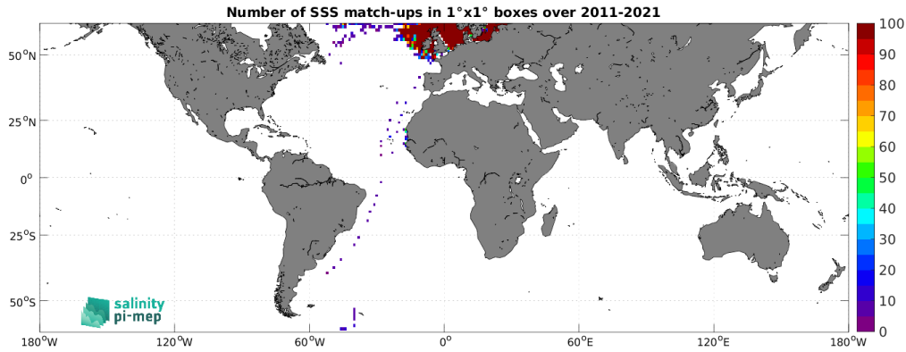
Figure 5: Number of SSS match-ups between ICES SSS and the SMOS SSS L3 v2 - 9-Days (BEC) SSS product for the SMOS coastal zone (<800km) 60N-60S Pi-MEP region over 1^\circ \times 1^\circ boxes and for the full satellite product period.
