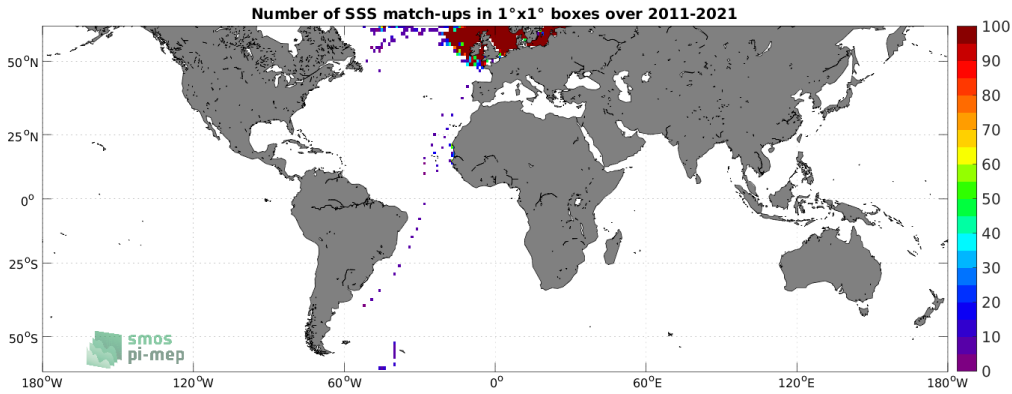
Figure 4: Number of SSS match-ups between ICES SSS and the SMOS SSS L3 v2 - 9-Days (BEC) SSS product for the SMOS coastal zone (<800km) 60N-60S Pi-MEP region over 1^\circ \times 1^\circ boxes and for the full satellite product period.
