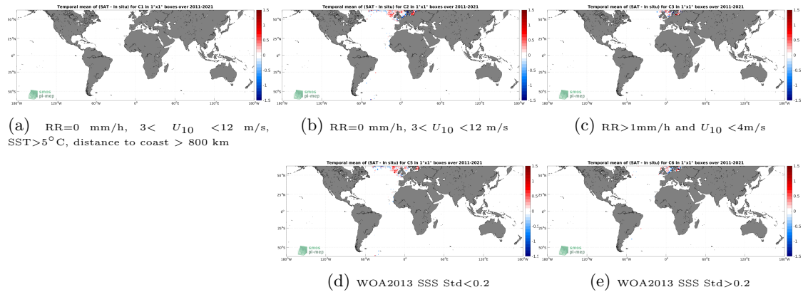
Figure 12: Temporal mean gridded over spatial boxes of size 1^\circ \times 1^\circ of \Delta SSS (SMOS SSS L3 v2 - 9-Days (BEC) - ICES) for 5 different subdatasets corresponding to:RR=0 mm/h, 3 < U_{10} < 12 m/s, SST >5^\circ\text{C} , distance to coast > 800 km (a), RR=0 mm/h, 3 < U_{10} < 12 m/s (b), RR >1 mm/h and U_{10} < 4 m/s (c), WOA2013 SSS Std <0.2 (d), WOA2013 SSS Std >0.2 (e).
