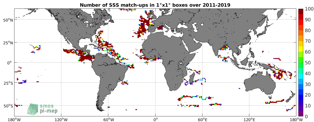
Figure 3: Number of SSS match-ups between Surface drifters SSS and the SMOS SSS L3 v2 - 9-Days (BEC) SSS product for the SMOS coastal zone (<800km) 60N-60S Pi-MEP region over 1°x1° boxes and for the full satellite product period.
