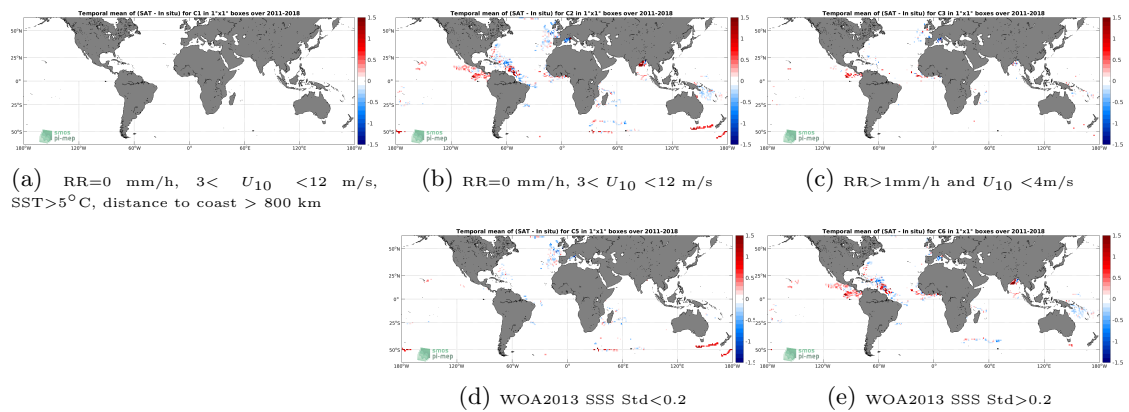
Figure 11: Temporal mean gridded over spatial boxes of size 1^\circ \times 1^\circ of \Delta SSS (SMOS SSS L3 v2 - 9-Days (BEC) - Surface drifters) for 5 different subdatasets corresponding to: RR=0 mm/h, 3 < U_{10} < 12 m/s, SST > 5°C, distance to coast > 800 km (a), RR=0 mm/h, 3 < U_{10} < 12 m/s (b), RR > 1mm/h and U_{10} < 4 m/s (c), WOA2013 SSS Std < 0.2 (d), WOA2013 SSS Std > 0.2 (e).
