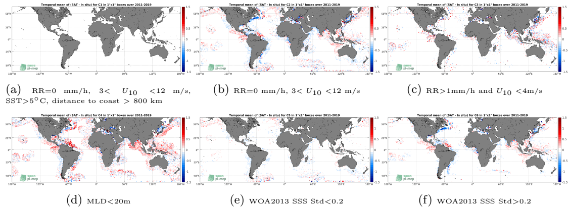
Figure 12: Temporal mean gridded over spatial boxes of size 1^\circ \times 1^\circ of \Delta SSS (SMOS SSS L3 v2 - 9-Days (BEC) - Argo) for 6 different subdatasets corresponding to: RR=0 mm/h, 3 < U_{10} < 12 m/s, SST > 5°C, distance to coast > 800 km (a), RR=0 mm/h, 3 < U_{10} < 12 m/s (b), RR > 1mm/h and U_{10} < 4 m/s (c), MLD < 20m (d), WOA2013 SSS Std < 0.2 (e), WOA2013 SSS Std > 0.2 (f).
