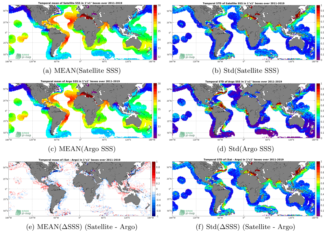
Figure 6: Temporal mean (left) and Std (right) of SSS from SMOS L3 v2 - 9-Days (BEC) (top), Argo (middle), and of \Delta SSS (Satellite - Argo). Only match-up pairs are used to generate these maps.
