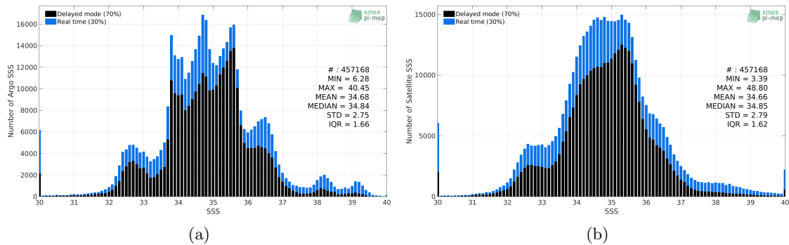
Figure 2: Histograms of SSS from Argo (a) and SMOS L3 v2 - 9-Days (BEC) (b) considering all match-up pairs per bins of 0.1 over the SMOS coastal zone (<800km) 60N-60S Pi-MEP region and for the full satellite product period.
