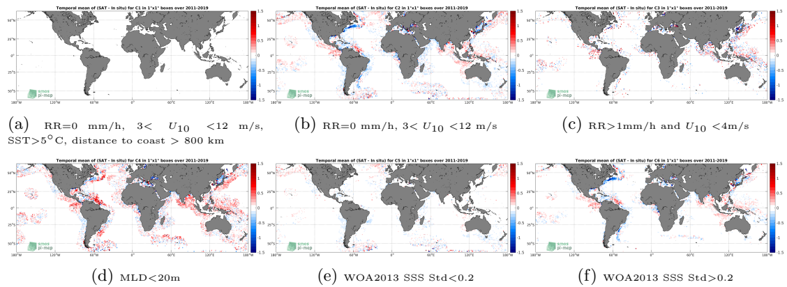
Figure 12: Temporal mean gridded over spatial boxes of size 1^\circ \times 1^\circ of \Delta SSS (SMOS L3 v2 - 9-Days (BEC) - Argo) for 6 different subdatasets corresponding to:RR=0 mm/h, 3 < U_{10} < 12 m/s, SST >5^\circ\text{C} , distance to coast > 800 km (a), RR=0 mm/h, 3 < U_{10} < 12 m/s (b), RR >1 mm/h and U_{10} < 4 m/s (c),MLD <20 m (d),WOA2013 SSS Std <0.2 (e),WOA2013 SSS Std >0.2 (f).
