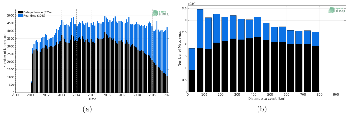
Figure 1: Number of match-ups between Argo and SMOS L3 v2 - 9-Days (BEC) SSS as a function of time (a) and as function of the distance to coast (b) over the SMOS coastal zone (<800km) 60N-60S Pi-MEP region and for the full satellite product period.
