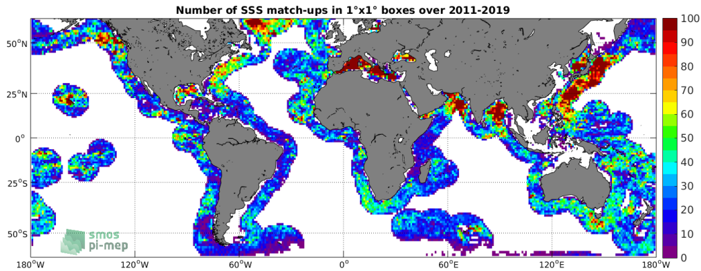
Figure 4: Number of SSS match-ups between Argo SSS and the SMOS L3 v2 - 9-Days (BEC) SSS product for the SMOS coastal zone (<800km) 60N-60S Pi-MEP region over 1°x1° boxes and for the full satellite product period.
