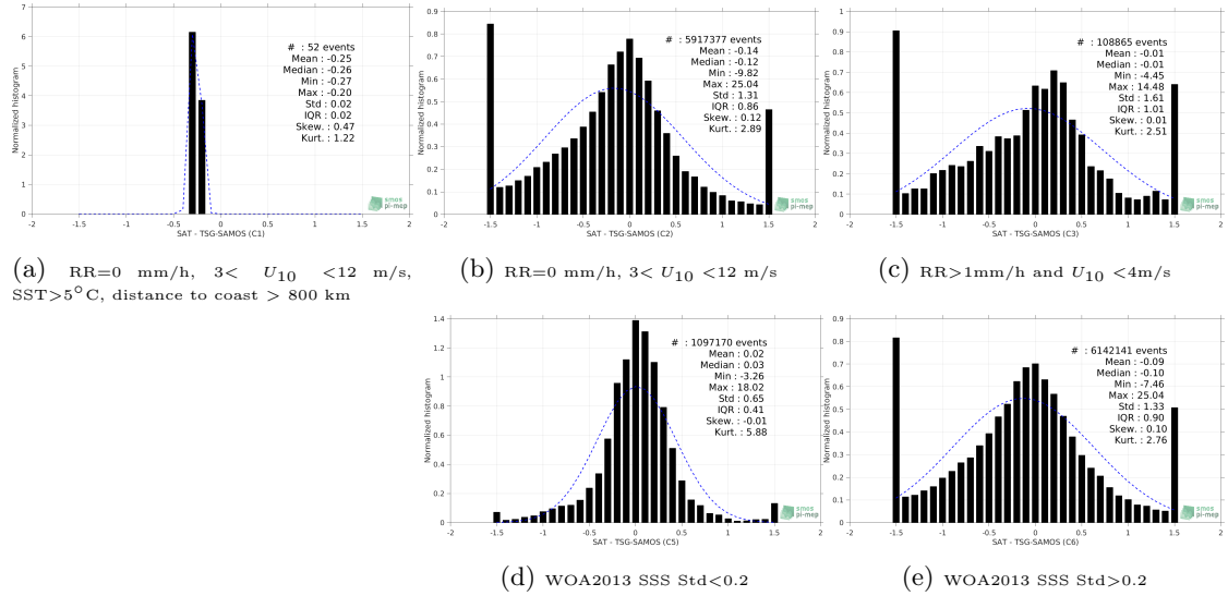
Figure 13: Normalized histogram of \Delta SSS (SMOS-L3-BEC-OA-V1-9DAYS-0.25DEG - TSG-SAMOS) for 5 different subdatasets corresponding to: RR=0 mm/h, 3 < U_{10} < 12 m/s, SST > 5°C, distance to coast > 800 km (a), RR=0 mm/h, 3 < U_{10} < 12 m/s (b), RR > 1mm/h and U_{10} < 4 m/s (c), WOA2013 SSS Std < 0.2 (d), WOA2013 SSS Std > 0.2 (e).
