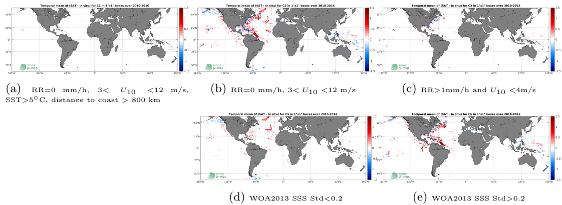
Figure 12: Temporal mean gridded over spatial boxes of size 1^\circ \times 1^\circ of \Delta SSS (SMOS-L3-BEC-OA-V1-9DAYS-0.25DEG - TSG-SAMOS) for 5 different subdatasets corresponding to:RR=0 mm/h, 3 < U_{10} < 12 m/s, SST >5^\circ C, distance to coast > 800 km (a), RR=0 mm/h, 3 < U_{10} < 12 m/s (b), RR >1 mm/h and U_{10} < 4 m/s (c), WOA2013 SSS Std <0.2 (d), WOA2013 SSS Std >0.2 (e).
