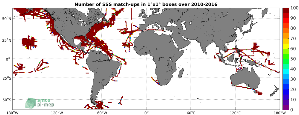
Figure 4: Number of SSS match-ups between TSG-SAMOS SSS and the SMOS-L3-BEC-OA-V1-9DAYS-0.25DEG SSS product for the SMOS coastal zone ( \pm 800\text{km} ) 60N-60S Pi-MEP region over 1^\circ \times 1^\circ boxes and for the full satellite product period.
