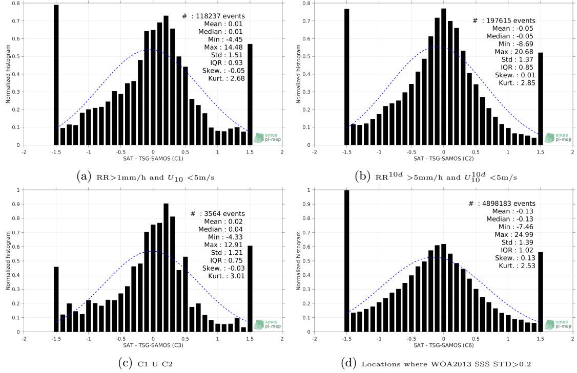
Figure 13: Normalized histogram of \Delta SSS (SMOS-L3-BEC-OA-V1-9DAYS-0.25DEG - TSG-SAMOS) for 6 different subdatasets corresponding to: RR > 1\text{mm/h} and U_{10} < 5\text{m/s} (a), RR^{10d} > 5\text{mm/h} and U_{10}^{10d} < 5\text{m/s} (b), C1 U C2 (c), Locations where WOA2013 SSS STD > 0.2 (d).
