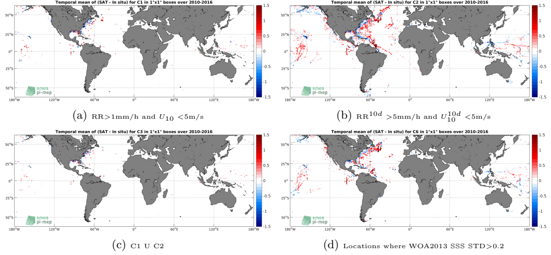
Figure 12: Temporal mean gridded over spatial boxes of size 1^\circ \times 1^\circ of \Delta SSS (SMOS-L3-BEC-OA-V1-9DAYS-0.25DEG - TSG-SAMOS) for 4 different subdatasets corresponding to: RR > 1mm/h and U_{10} < 5\text{m/s} (a), RR^{10d} > 5\text{mm/h} and U_{10}^{10d} < 5\text{m/s} (b), C1 U C2 (c), Locations where WOA2013 SSS STD > 0.2 (d).
