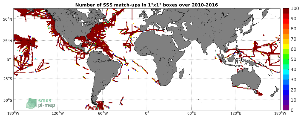
Figure 4: Number of SSS match-ups between TSG-SAMOS SSS and the SMOS-L3-BEC-OA-V1-9DAYS-0.25DEG SSS product for the SMOS coastal zone ( \leq 800\text{km} ) 60N-60S Pi-MEP region over 1^\circ \times 1^\circ boxes and for the full satellite product period.
