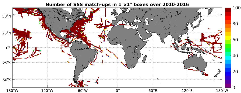
Figure 4: Number of SSS match-ups between TSG-SAMOS SSS and the SMOS-L3-BEC-OA-V1-9DAYS-0.25DEG SSS product for the SMOS coastal zone ( \approx 800 km) 60N-60S Pi-MEP region over 1^\circ \times 1^\circ boxes and for the full satellite product period.
