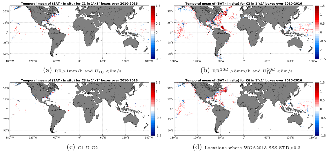
Figure 12: Temporal mean gridded over spatial boxes of size 1^\circ \times 1^\circ of \Delta SSS (SMOS-L3-BEC-OA-V1-9DAYS-0.25DEG - TSG-SAMOS) for 4 different subdatasets corresponding to:RR >1 mm/h and U_{10} < 5 m/s (a), RR 10d > 5 mm/h and U_{10}^{10d} < 5 m/s (b), C1 U C2 (c),Locations where WOA2013 SSS STD >0.2 (d).
