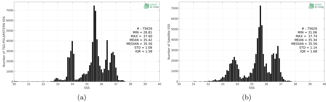
Figure 2: Histograms of SSS from TSG-POLARSTERN (a) and SMOS-L3-BEC-OA-V1-9DAYS-0.25DEG (b) considering all match-up pairs per bins of 0.1 over the SMOS coastal zone ( \approx 800 km) 60N-60S Pi-MEP region and for the full satellite product period.
