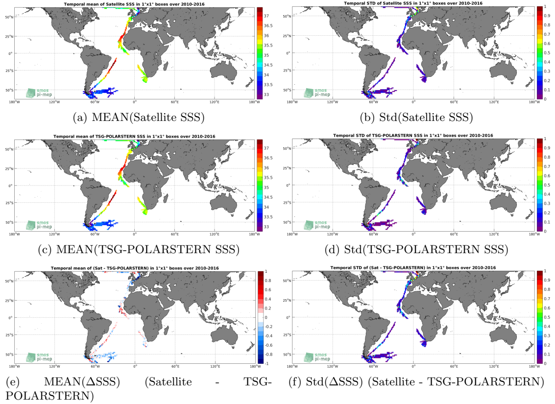
Figure 6: Temporal mean (left) and Std (right) of SSS from SMOS-L3-BEC-OA-V1-9DAYS-0.25DEG (top), TSG-POLARSTERN (middle), and of \Delta SSS (Satellite - TSG-POLARSTERN). Only match-up pairs are used to generate these maps.
