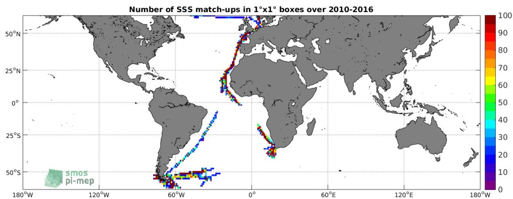
Figure 4: Number of SSS match-ups between TSG-POLARSTERN SSS and the SMOS-L3-BEC-OA-V1-9DAYS-0.25DEG SSS product for the SMOS coastal zone ( \pm 800\text{km} ) 60N-60S Pi-MEP region over 1^\circ \times 1^\circ boxes and for the full satellite product period.
