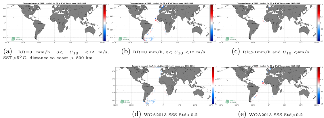
Figure 12: Temporal mean gridded over spatial boxes of size 1^\circ \times 1^\circ of \Delta SSS (SMOS-L3-BEC-OA-V1-9DAYS-0.25DEG - TSG-POLARSTERN) for 5 different subdatasets corresponding to:RR=0 mm/h, 3 < U_{10} < 12 m/s, SST >5^\circ\text{C} , distance to coast > 800 km (a), RR=0 mm/h, 3 < U_{10} < 12 m/s (b), RR >1 mm/h and U_{10} < 4 m/s (c), WOA2013 SSS Std <0.2 (d), WOA2013 SSS Std >0.2 (e).
