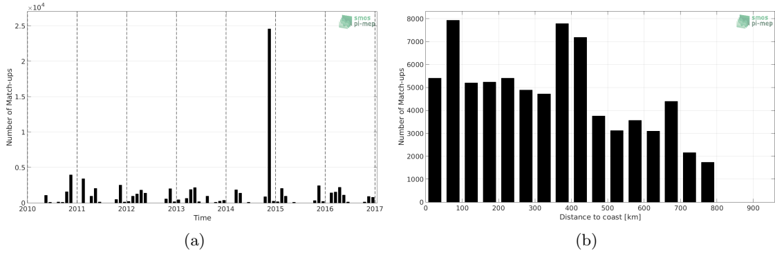
Figure 1: Number of match-ups between TSG-POLARSTERN and SMOS-L3-BEC-OA-V1-9DAYS-0.25DEG SSS as a function of time (a) and as function of the distance to coast (b) over the SMOS coastal zone ( \approx 800 km) 60N-60S Pi-MEP region and for the full satellite product period.
