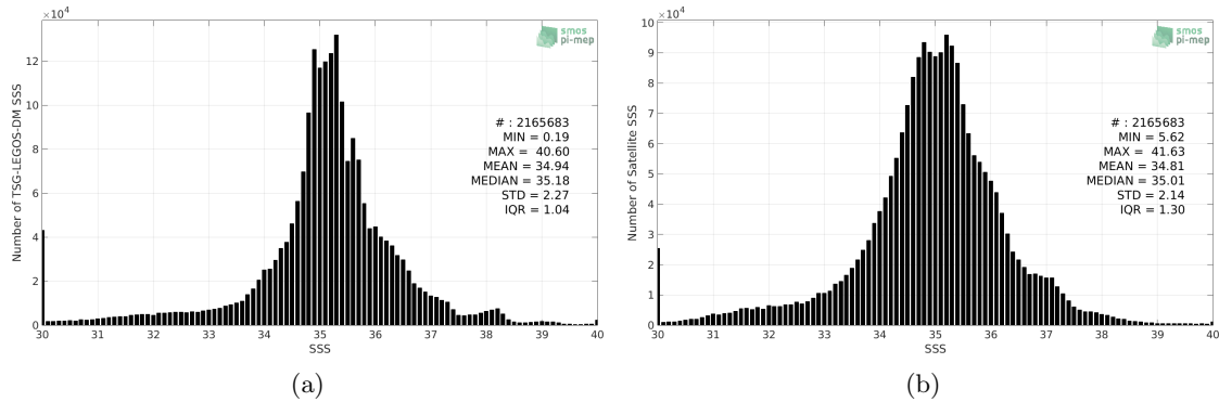
Figure 2: Histograms of SSS from TSG-LEGOS-DM (a) and SMOS-L3-BEC-OA-V1-9DAYS-0.25DEG (b) considering all match-up pairs per bins of 0.1 over the SMOS coastal zone ( \geq 800 km) 60N-60S Pi-MEP region and for the full satellite product period.
