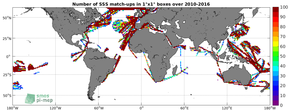
Figure 4: Number of SSS match-ups between TSG-LEGOS-DM SSS and the SMOS-L3-BEC-OA-V1-9DAYS-0.25DEG SSS product for the SMOS coastal zone ( \geq 800\text{km} ) 60N-60S Pi-MEP region over 1^\circ \times 1^\circ boxes and for the full satellite product period.
