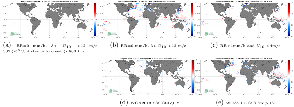
Figure 12: Temporal mean gridded over spatial boxes of size 1^\circ \times 1^\circ of \Delta SSS (SMOS-L3-BEC-OA-V1-9DAYS-0.25DEG - TSG-LEGOS-DM) for 5 different subdatasets corresponding to: RR=0 mm/h, 3 < U_{10} < 12 m/s, SST > 5^\circ C , distance to coast > 800 km (a), RR=0 mm/h, 3 < U_{10} < 12 m/s (b), RR > 1 mm/h and U_{10} < 4 m/s (c), WOA2013 SSS Std < 0.2 (d), WOA2013 SSS Std > 0.2 (e).
