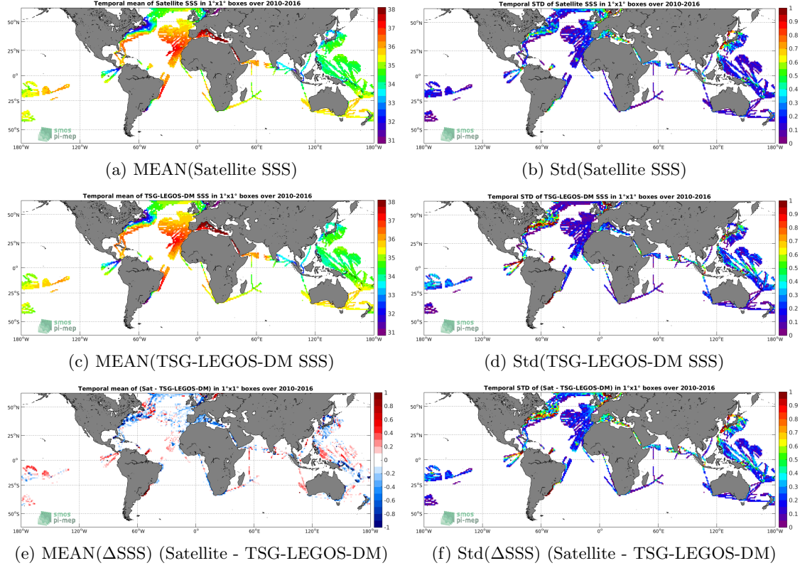
Figure 6: Temporal mean (left) and Std (right) of SSS from SMOS-L3-BEC-OA-V1-9DAYS-0.25DEG (top), TSG-LEGOS-DM (middle), and of \Delta SSS (Satellite - TSG-LEGOS-DM). Only match-up pairs are used to generate these maps.
