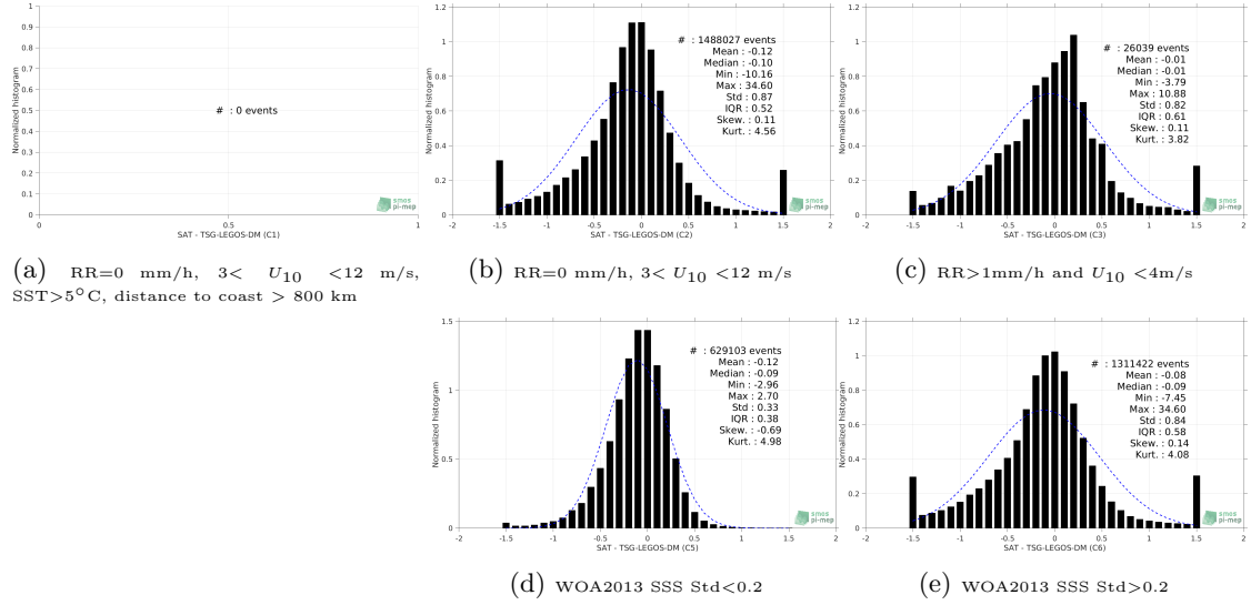
Figure 13: Normalized histogram of \Delta SSS (SMOS-L3-BEC-OA-V1-9DAYS-0.25DEG - TSG-LEGOS-DM) for 5 different subdatasets corresponding to: RR=0 mm/h, 3 < U_{10} < 12 m/s, SST > 5^\circ C , distance to coast > 800 km (a), RR=0 mm/h, 3 < U_{10} < 12 m/s (b), RR > 1 mm/h and U_{10} < 4 m/s (c), WOA2013 SSS Std < 0.2 (d), WOA2013 SSS Std > 0.2 (e).
