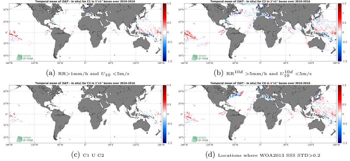
Figure 12: Temporal mean gridded over spatial boxes of size 1^\circ \times 1^\circ of \Delta SSS (SMOS-L3-BEC-OA-V1-9DAYS-0.25DEG - TSG-LEGOS-DM) for 4 different subdatasets corresponding to: RR > 1\text{mm/h} and U_{10} < 5\text{m/s} (a), RR^{10d} > 5\text{mm/h} and U_{10}^{10d} < 5\text{m/s} (b), C1 U C2 (c), Locations where WOA2013 SSS STD > 0.2 (d).
