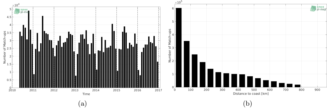
Figure 1: Number of match-ups between TSG-LEGOS-DM and SMOS-L3-BEC-OA-V1-9DAYS-0.25DEG SSS as a function of time (a) and as function of the distance to coast (b) over the SMOS coastal zone ( \leq 800 km) 60N-60S Pi-MEP region and for the full satellite product period.
