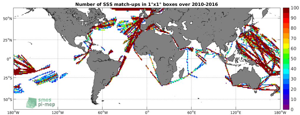
Figure 4: Number of SSS match-ups between TSG-LEGOS-DM SSS and the SMOS-L3-BEC-OA-V1-9DAYS-0.25DEG SSS product for the SMOS coastal zone ( \geq 800 km) 60N-60S Pi-MEP region over 1^\circ \times 1^\circ boxes and for the full satellite product period.
