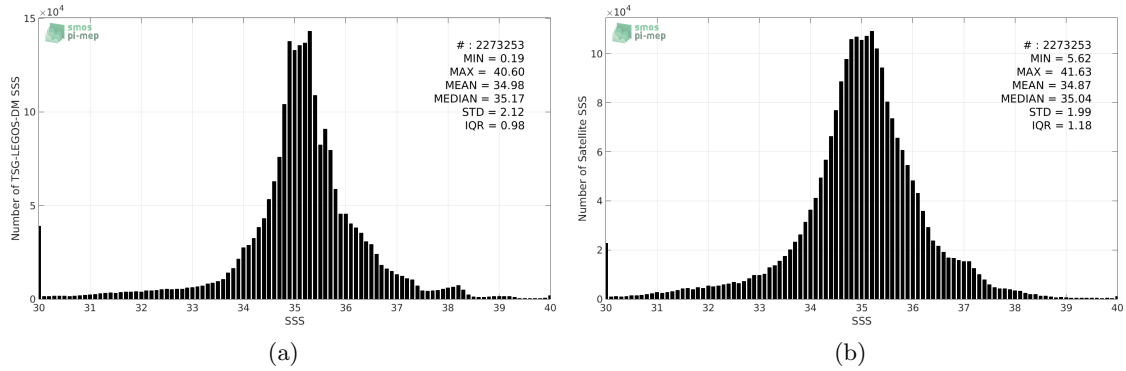
Figure 2: Histograms of SSS from TSG-LEGOS-DM (a) and SMOS-L3-BEC-OA-V1-9DAYS-0.25DEG (b) considering all match-up pairs per bins of 0.1 over the SMOS coastal zone ( \leq 800 km) 60N-60S Pi-MEP region and for the full satellite product period.
