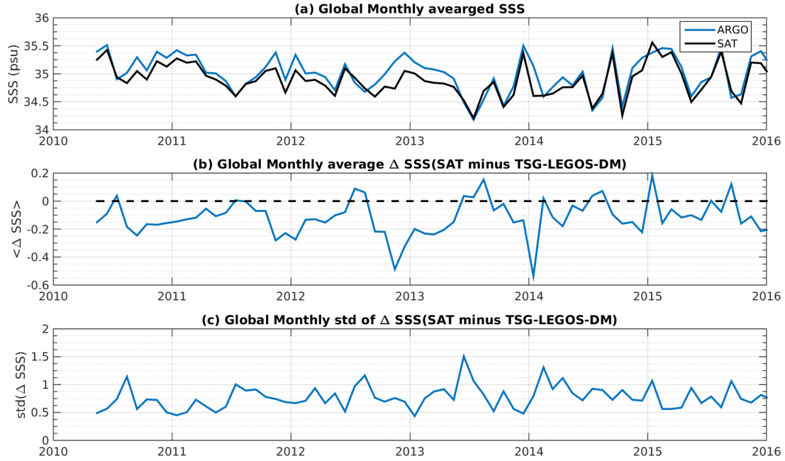
Figure 7: Time series of the monthly averaged mean SSS (top), mean \Delta SSS (Satellite - TSG-LEGOS-DM) and STD of \Delta SSS (Satellite - TSG-LEGOS-DM) over the SMOS coastal zone ( \geq 800 km) 60N-60S Pi-MEP region considering all match-ups collected by the Pi-MEP platform.
