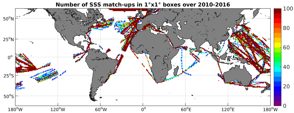
Figure 4: Number of SSS match-ups between TSG-LEGOS-DM SSS and the SMOS-L3-BEC-OA-V1-9DAYS-0.25DEG SSS product for the SMOS coastal zone ( \pm 800\text{km} ) 60N-60S Pi-MEP region over 1^\circ \times 1^\circ boxes and for the full satellite product period.
