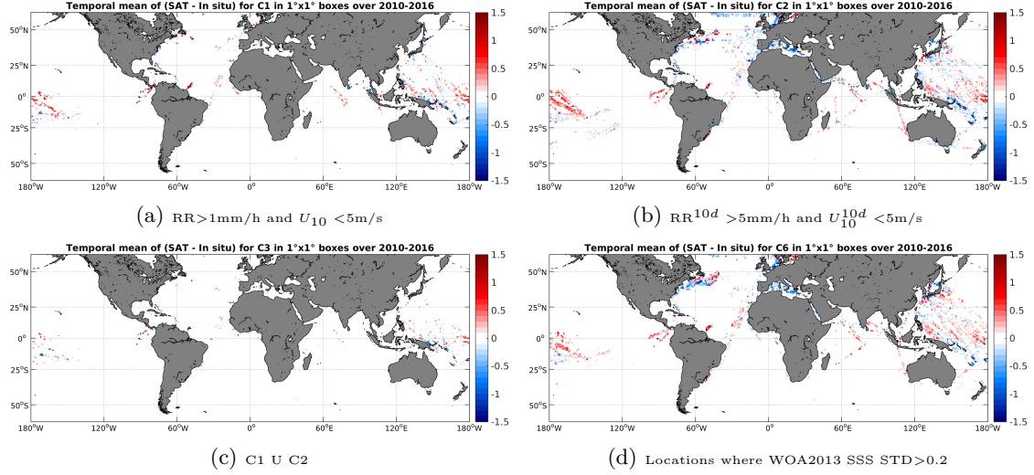
Figure 12: Temporal mean gridded over spatial boxes of size 1^\circ \times 1^\circ of \Delta SSS (SMOS-L3-BEC-OA-V1-9DAYS-0.25DEG - TSG-LEGOS-DM) for 4 different subdatasets corresponding to: RR > 1mm/h and U_{10} < 5 m/s (a), RR^{10d} > 5 mm/h and U_{10}^{10d} < 5 m/s (b), C1 U C2 (c), Locations where WOA2013 SSS STD > 0.2 (d).
