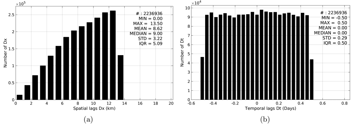
Figure 5: Histograms of the spatial (a) and temporal (b) lags between the time of the TSG-LEGOS-DM measurements and the date of the corresponding SMOS-L3-BEC-OA-V1-9DAYS-0.25DEG SSS product.
