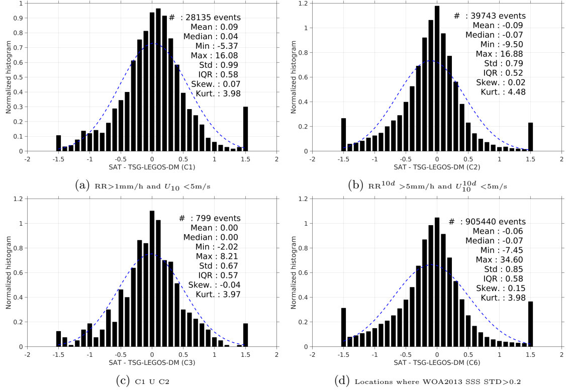
Figure 13: Normalized histogram of \Delta SSS (SMOS-L3-BEC-OA-V1-9DAYS-0.25DEG - TSG-LEGOS-DM) for 6 different subdatasets corresponding to: RR > 1\text{mm/h} and U_{10} < 5\text{m/s} (a), RR^{10d} > 5\text{mm/h} and U_{10}^{10d} < 5\text{m/s} (b), C1 U C2 (c), Locations where WOA2013 SSS STD > 0.2 (d).
