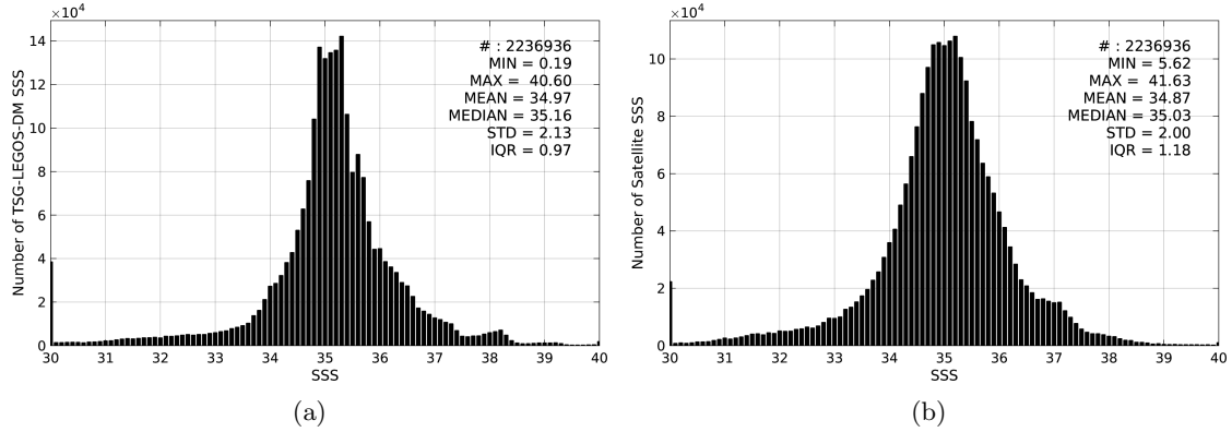
Figure 2: Histograms of SSS from TSG-LEGOS-DM (a) and SMOS-L3-BEC-OA-V1-9DAYS-0.25DEG (b) considering all match-up pairs per bins of 0.1 over the SMOS coastal zone ( \geq 800 km) 60N-60S Pi-MEP region and for the full satellite product period.
