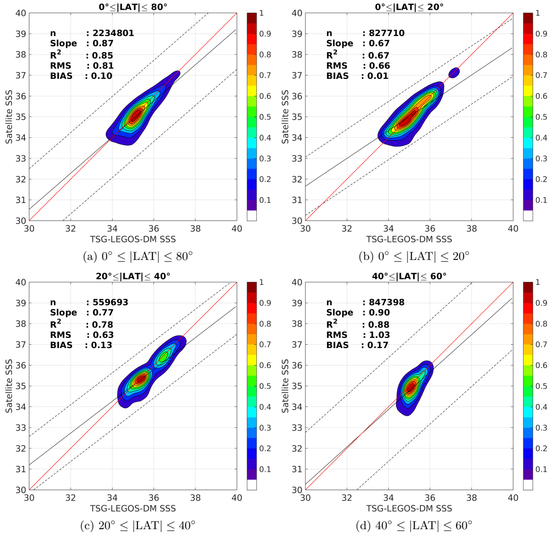
Figure 9: Contour maps of the concentration of SMOS-L3-BEC-OA-V1-9DAYS-0.25DEG SSS (y-axis) versus TSG-LEGOS-DM SSS (x-axis) at match-up pairs for different latitude bands. For each plot, the red line shows x=y . The black thin and dashed lines indicate a linear fit through the data cloud and the \pm 95\% confidence levels, respectively. The number match-up pairs n , the slope and R^2 coefficient of the linear fit, the root mean square (RMS) and the mean bias between satellite and in situ data are indicated for each latitude band in each plots.
