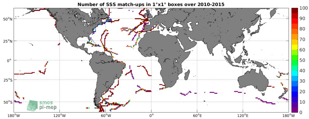
Figure 4: Number of SSS match-ups between TSG-GOSUD-Sailing-ship SSS and the SMOS-L3-BEC-OA-V1-9DAYS-0.25DEG SSS product for the SMOS coastal zone ( \pm 800\text{km} ) 60N-60S Pi-MEP region over 1^\circ \times 1^\circ boxes and for the full satellite product period.
