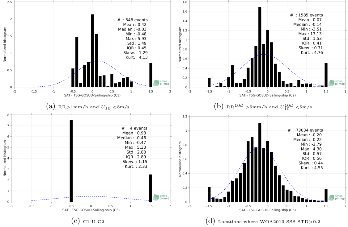
Figure 13: Normalized histogram of \Delta SSS (SMOS-L3-BEC-OA-V1-9DAYS-0.25DEG - TSG-GOSUD-Sailing-ship) for 6 different subdatasets corresponding to: RR > 1\text{mm/h} and U_{10} < 5\text{m/s} (a), RR^{10d} > 5\text{mm/h} and U_{10}^{10d} < 5\text{m/s} (b), C1 U C2 (c), Locations where WOA2013 SSS STD > 0.2 (d).
