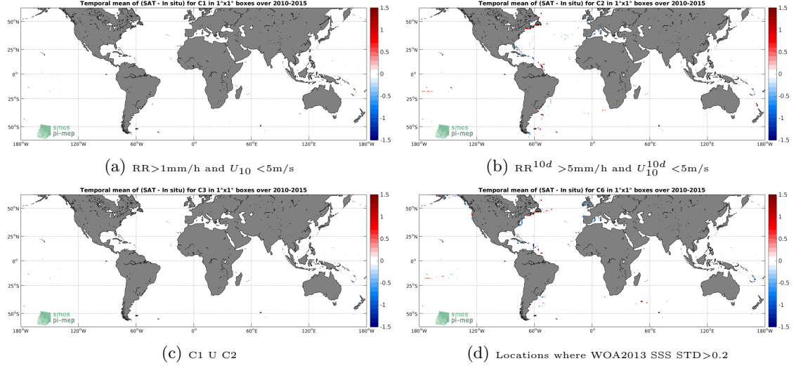
Figure 12: Temporal mean gridded over spatial boxes of size 1^\circ \times 1^\circ of \Delta SSS (SMOS-L3-BEC-OA-V1-9DAYS-0.25DEG - TSG-GOSUD-Sailing-ship) for 4 different subdatasets corresponding to: RR > 1\text{mm/h} and U_{10} < 5\text{m/s} (a), RR^{10d} > 5\text{mm/h} and U_{10}^{10d} < 5\text{m/s} (b), C1 U C2 (c), Locations where WOA2013 SSS STD > 0.2 (d).
