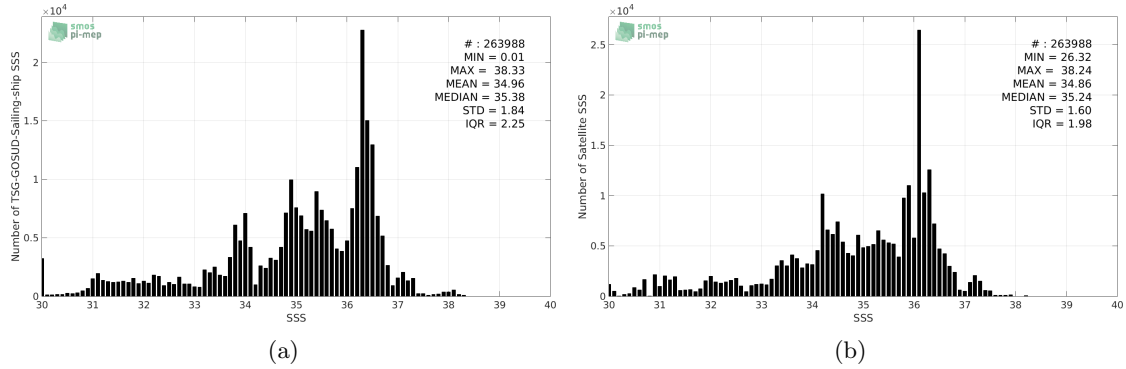
Figure 2: Histograms of SSS from TSG-GOSUD-Sailing-ship (a) and SMOS-L3-BEC-OA-V1-9DAYS-0.25DEG (b) considering all match-up pairs per bins of 0.1 over the SMOS coastal zone ( \approx 800 km) 60N-60S Pi-MEP region and for the full satellite product period.
