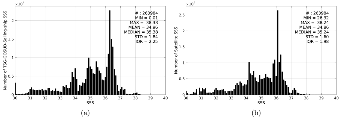
Figure 2: Histograms of SSS from TSG-GOSUD-Sailing-ship (a) and SMOS-L3-BEC-OA-V1-9DAYS-0.25DEG (b) considering all match-up pairs per bins of 0.1 over the SMOS coastal zone ( \leq 800 km) 60N-60S Pi-MEP region and for the full satellite product period.
