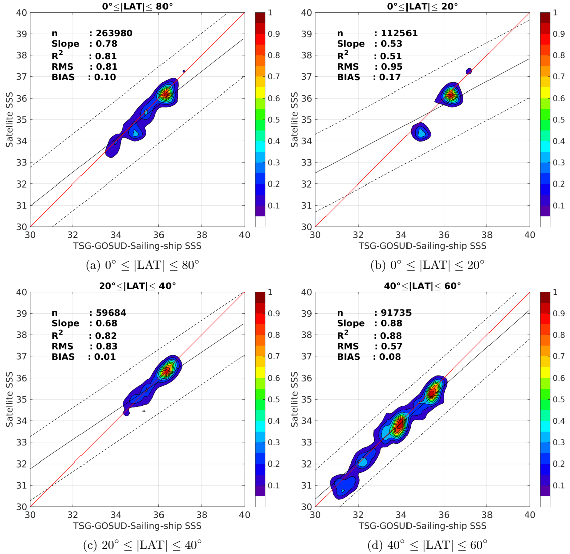
Figure 9: Contour maps of the concentration of SMOS-L3-BEC-OA-V1-9DAYS-0.25DEG SSS (y-axis) versus TSG-GOSUD-Sailing-ship SSS (x-axis) at match-up pairs for different latitude bands. For each plot, the red line shows x=y . The black thin and dashed lines indicate a linear fit through the data cloud and the \pm 95\% confidence levels, respectively. The number match-up pairs n , the slope and R^2 coefficient of the linear fit, the root mean square (RMS) and the mean bias between satellite and in situ data are indicated for each latitude band in each plots.
