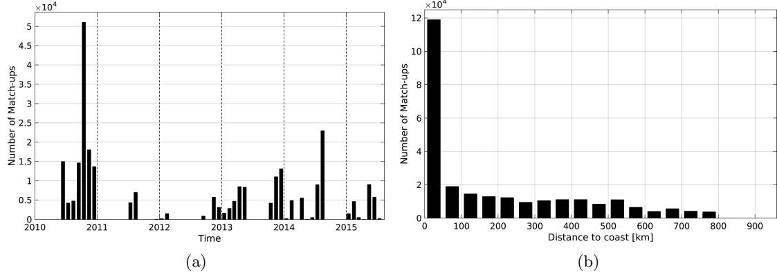
Figure 1: Number of match-ups between TSG-GOSUD-Sailing-ship and SMOS-L3-BEC-OA-V1-9DAYS-0.25DEG SSS as a function of time (a) and as function of the distance to coast (b) over the SMOS coastal zone ( \leq 800 km) 60N-60S Pi-MEP region and for the full satellite product period.
