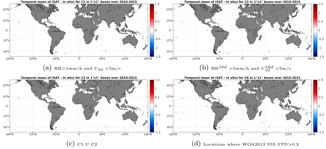
Figure 12: Temporal mean gridded over spatial boxes of size 1^\circ \times 1^\circ of \Delta SSS (SMOS-L3-BEC-OA-V1-9DAYS-0.25DEG - TSG-GOSUD-Sailing-ship) for 4 different subdatasets corresponding to: RR > 1mm/h and U_{10} < 5 m/s (a), RR^{10d} > 5 mm/h and U_{10}^{10d} < 5 m/s (b), C1 U C2 (c), Locations where WOA2013 SSS STD > 0.2 (d).
