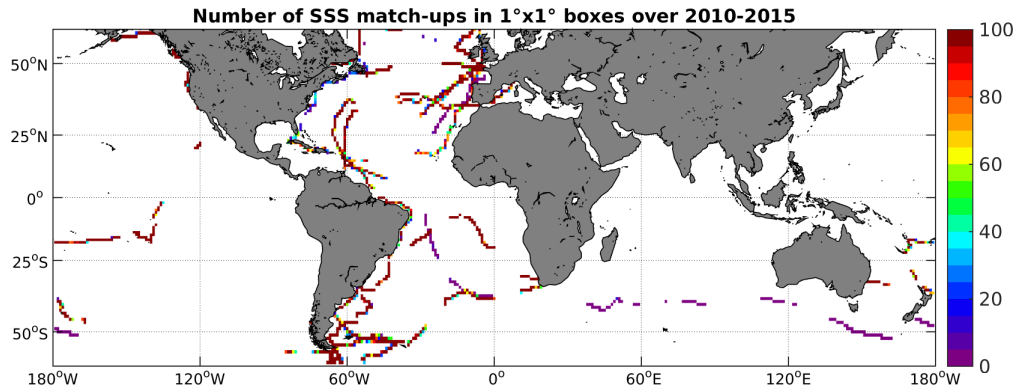
Figure 4: Number of SSS match-ups between TSG-GOSUD-Sailing-ship SSS and the SMOS-L3-BEC-OA-V1-9DAYS-0.25DEG SSS product for the SMOS coastal zone ( \pm 800 km) 60N-60S Pi-MEP region over 1^\circ \times 1^\circ boxes and for the full satellite product period.
