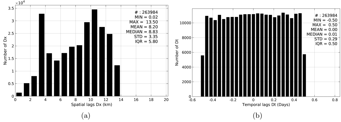
Figure 5: Histograms of the spatial (a) and temporal (b) lags between the time of the TSG-GOSUD-Sailing-ship measurements and the date of the corresponding SMOS-L3-BEC-OA-V1-9DAYS-0.25DEG SSS product.
