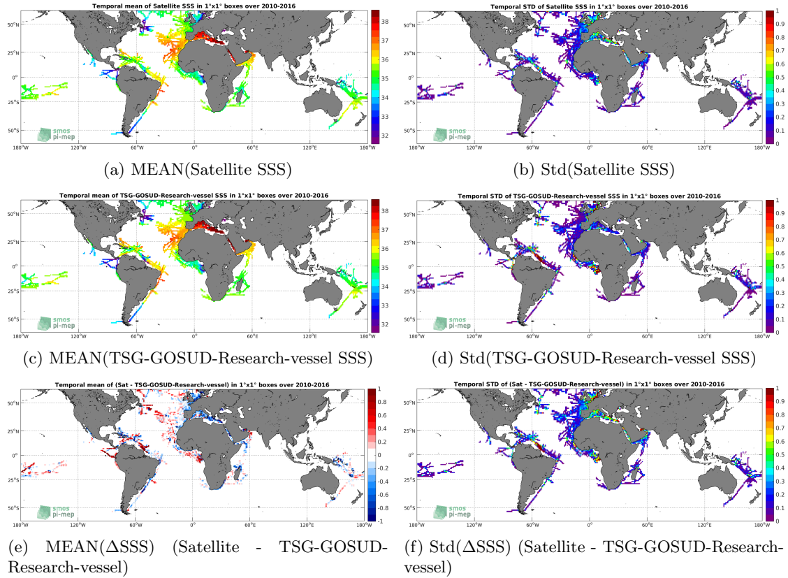
Figure 6: Temporal mean (left) and Std (right) of SSS from SMOS-L3-BEC-OA-V1-9DAYS-0.25DEG (top), TSG-GOSUD-Research-vessel (middle), and of \Delta SSS (Satellite - TSG-GOSUD-Research-vessel). Only match-up pairs are used to generate these maps.
