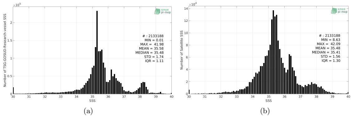
Figure 2: Histograms of SSS from TSG-GOSUD-Research-vessel (a) and SMOS-L3-BEC-OA-V1-9DAYS-0.25DEG (b) considering all match-up pairs per bins of 0.1 over the SMOS coastal zone ( \approx 800 km) 60N-60S Pi-MEP region and for the full satellite product period.
