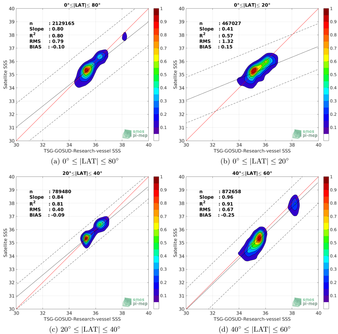
Figure 9: Contour maps of the concentration of SMOS-L3-BEC-OA-V1-9DAYS-0.25DEG SSS (y-axis) versus TSG-GOSUD-Research-vessel SSS (x-axis) at match-up pairs for different latitudinal bands. For each plot, the red line shows x=y . The black thin and dashed lines indicate a linear fit through the data cloud and the \pm 95\% confidence levels, respectively. The number match-up pairs n , the slope and R^2 coefficient of the linear fit, the root mean square (RMS) and the mean bias between satellite and in situ data are indicated for each latitude band in each plots.
