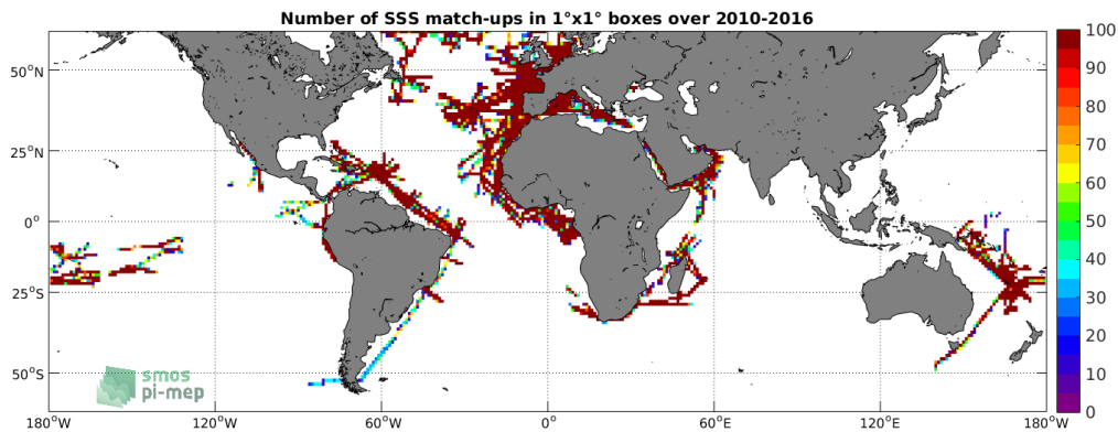
Figure 4: Number of SSS match-ups between TSG-GOSUD-Research-vessel SSS and the SMOS-L3-BEC-OA-V1-9DAYS-0.25DEG SSS product for the SMOS coastal zone ( \approx 800\text{km} ) 60N-60S Pi-MEP region over 1^\circ \times 1^\circ boxes and for the full satellite product period.
