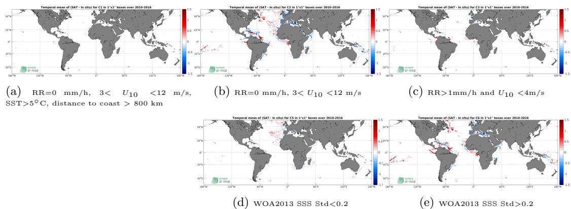
Figure 12: Temporal mean gridded over spatial boxes of size 1^\circ \times 1^\circ of \Delta SSS (SMOS-L3-BEC-OA-V1-9DAYS-0.25DEG - TSG-GOSUD-Research-vessel) for 5 different subdatasets corresponding to:RR=0 mm/h, 3 < U_{10} < 12 m/s, SST >5^\circ\text{C} , distance to coast > 800 km (a), RR=0 mm/h, 3 < U_{10} < 12 m/s (b), RR >1 mm/h and U_{10} < 4 m/s (c), WOA2013 SSS Std <0.2 (d), WOA2013 SSS Std >0.2 (e).
