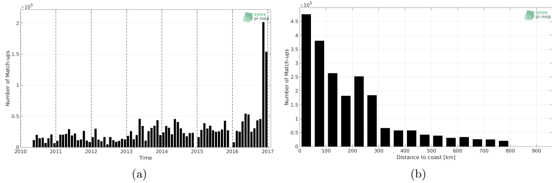
Figure 1: Number of match-ups between TSG-GOSUD-Research-vessel and SMOS-L3-BEC-OA-V1-9DAYS-0.25DEG SSS as a function of time (a) and as function of the distance to coast (b) over the SMOS coastal zone ( \approx 800 km) 60N-60S Pi-MEP region and for the full satellite product period.
