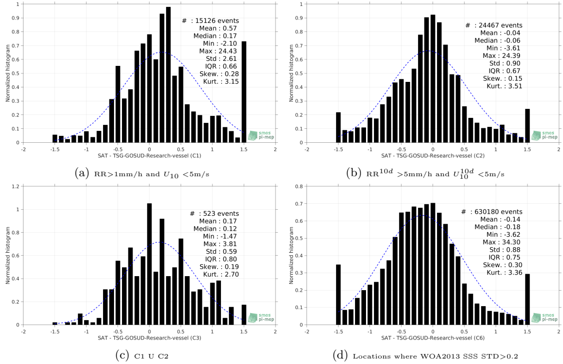
Figure 13: Normalized histogram of \Delta SSS (SMOS-L3-BEC-OA-V1-9DAYS-0.25DEG - TSG-GOSUD-Research-vessel) for 6 different subdatasets corresponding to: RR > 1mm/h and U_{10} < 5 m/s (a), RR 10d > 5mm/h and U_{10}^{10d} < 5 m/s (b), C1 U C2 (c), Locations where WOA2013 SSS STD > 0.2 (d).
