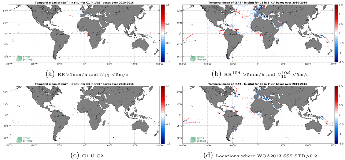
Figure 12: Temporal mean gridded over spatial boxes of size 1^\circ \times 1^\circ of \Delta SSS (SMOS-L3-BEC-OA-V1-9DAYS-0.25DEG - TSG-GOSUD-Research-vessel) for 4 different subdatasets corresponding to: RR > 1\text{mm/h} and U_{10} < 5\text{m/s} (a), RR^{10d} > 5\text{mm/h} and U_{10}^{10d} < 5\text{m/s} (b), C1 U C2 (c), Locations where WOA2013 SSS STD > 0.2 (d).
