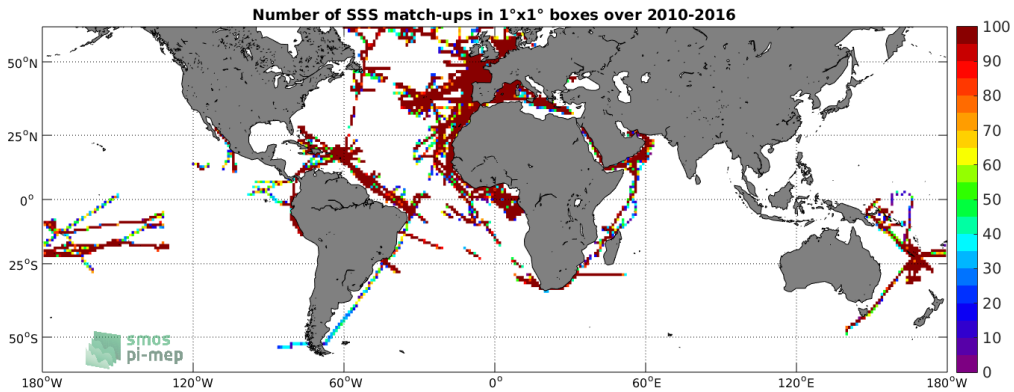
Figure 4: Number of SSS match-ups between TSG-GOSUD-Research-vessel SSS and the SMOS-L3-BEC-OA-V1-9DAYS-0.25DEG SSS product for the SMOS coastal zone ( \pm 800\text{km} ) 60N-60S Pi-MEP region over 1^\circ \times 1^\circ boxes and for the full satellite product period.
