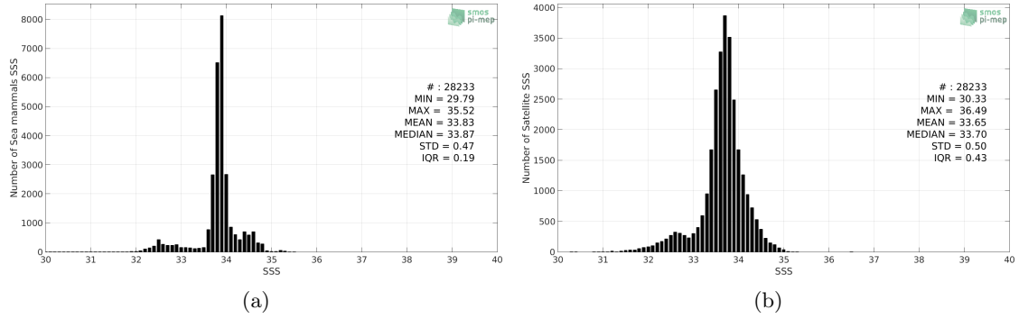
Figure 2: Histograms of SSS from Sea mammals (a) and SMOS-L3-BEC-OA-V1-9DAYS-0.25DEG (b) considering all match-up pairs per bins of 0.1 over the SMOS coastal zone ( \leq 800 km) 60N-60S Pi-MEP region and for the full satellite product period.
