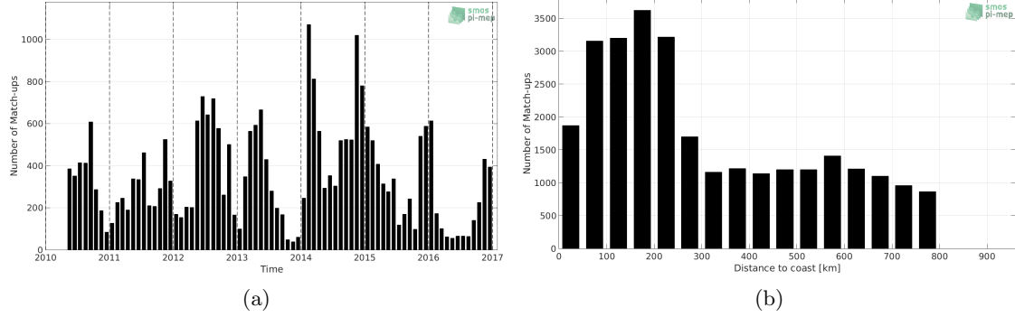
Figure 1: Number of match-ups between Sea mammals and SMOS-L3-BEC-OA-V1-9DAYS-0.25DEG SSS as a function of time (a) and as function of the distance to coast (b) over the SMOS coastal zone ( \leq 800 km) 60N-60S Pi-MEP region and for the full satellite product period.
