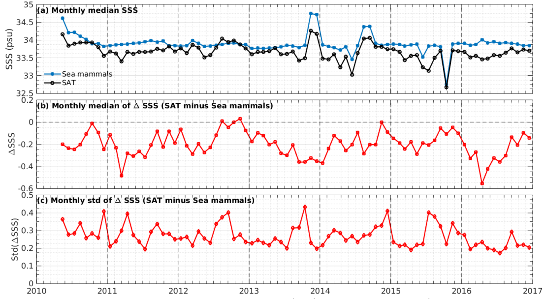
Figure 7: Time series of the monthly median SSS (top), median of \Delta SSS (Satellite - Sea mammals) and Std of \Delta SSS (Satellite - Sea mammals) over the SMOS coastal zone ( \pm 800 km) 60N-60S Pi-MEP region considering all match-ups collected by the Pi-MEP.
