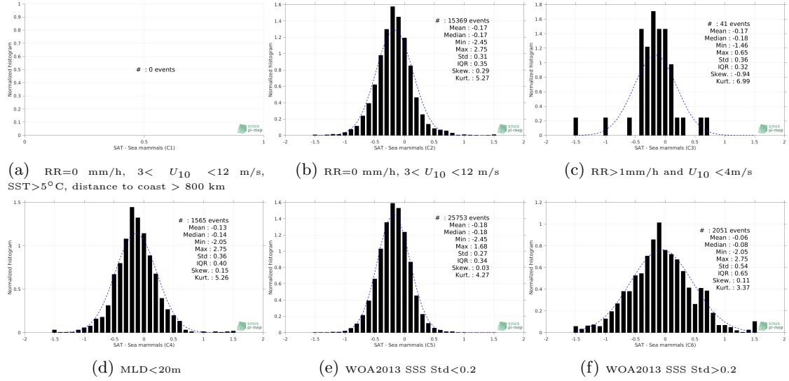
Figure 13: Normalized histogram of \Delta SSS (SMOS-L3-BEC-OA-V1-9DAYS-0.25DEG - Sea mammals) for 6 different subdatasets corresponding to: RR=0 mm/h, 3 < U_{10} < 12 m/s, SST>5°C, distance to coast > 800 km (a), RR=0 mm/h, 3 < U_{10} < 12 m/s (b), RR>1mm/h and U_{10} < 4 m/s (c), MLD<20m (d), WOA2013 SSS Std<0.2 (e), WOA2013 SSS Std>0.2 (f).
