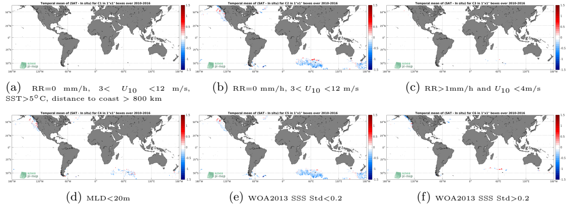
Figure 12: Temporal mean gridded over spatial boxes of size 1^\circ \times 1^\circ of \Delta SSS (SMOS-L3-BEC-OA-V1-9DAYS-0.25DEG - Sea mammals) for 6 different subdatasets corresponding to: RR=0 mm/h, 3 < U_{10} < 12 m/s, SST > 5^\circ C , distance to coast > 800 km (a), RR=0 mm/h, 3 < U_{10} < 12 m/s (b), RR > 1 mm/h and U_{10} < 4 m/s (c), MLD < 20 m (d), WOA2013 SSS Std < 0.2 (e), WOA2013 SSS Std > 0.2 (f).
