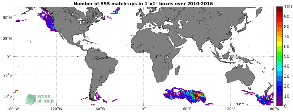
Figure 4: Number of SSS match-ups between Sea mammals SSS and the SMOS-L3-BEC-OA-V1-9DAYS-0.25DEG SSS product for the SMOS coastal zone ( \geq 800\text{km} ) 60N-60S Pi-MEP region over 1^\circ \times 1^\circ boxes and for the full satellite product period.
