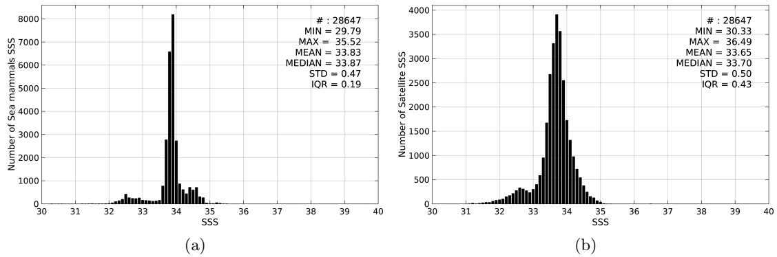
Figure 2: Histograms of SSS from Sea mammals (a) and SMOS-L3-BEC-OA-V1-9DAYS-0.25DEG (b) considering all match-up pairs per bins of 0.1 over the SMOS coastal zone ( \leq 800 km) 60N-60S Pi-MEP region and for the full satellite product period.
