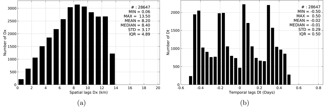
Figure 5: Histograms of the spatial (a) and temporal (b) lags between the time of the Sea mammals measurements and the date of the corresponding SMOS-L3-BEC-OA-V1-9DAYS-0.25DEG SSS product.
