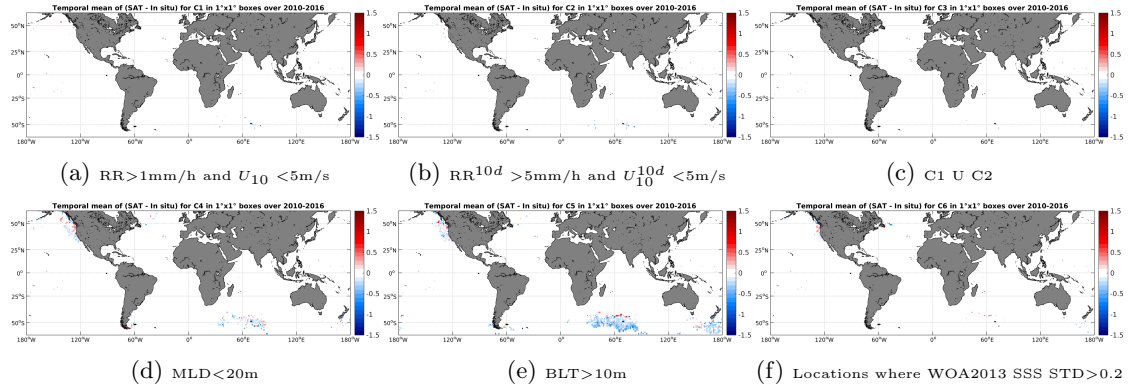
Figure 12: Temporal mean gridded over spatial boxes of size 1^\circ \times 1^\circ of \Delta SSS (SMOS-L3-BEC-OA-V1-9DAYS-0.25DEG - Sea mammals) for 6 different subdatasets corresponding to: RR > 1\text{mm/h} and U_{10} < 5\text{m/s} (a), RR^{10d} > 5\text{mm/h} and U_{10}^{10d} < 5\text{m/s} (b), C1 \cup C2 (c), MLD < 20\text{m} (d), BLT > 10\text{m} (e), Locations where WOA2013 SSS STD > 0.2 (f).
