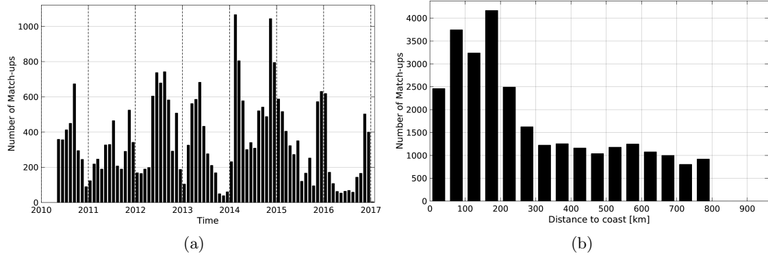
Figure 1: Number of match-ups between Sea mammals and SMOS-L3-BEC-OA-V1-9DAYS-0.25DEG SSS as a function of time (a) and as function of the distance to coast (b) over the SMOS coastal zone ( \leq 800 km) 60N-60S Pi-MEP region and for the full satellite product period.
