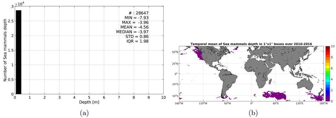
Figure 3: Histograms of the depth of the upper level SSS measurements from Sea mammals in the Match-up DataBase for the SMOS coastal zone ( \pm 800\text{km} ) 60N-60S Pi-MEP region (a) and temporal mean spatial distribution of pressure of the in situ SSS data over 1^\circ \times 1^\circ boxes and for the full satellite product period (b).
