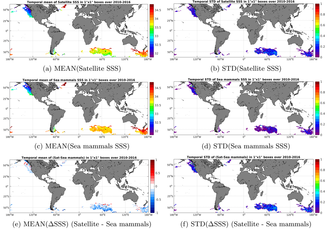
Figure 6: Temporal mean (left) and STD (right) of SSS from SMOS-L3-BEC-OA-V1-9DAYS-0.25DEG (top), Sea mammals (middle), and of \Delta SSS (Satellite - Sea mammals). Only match-up pairs are used to generate these maps.
