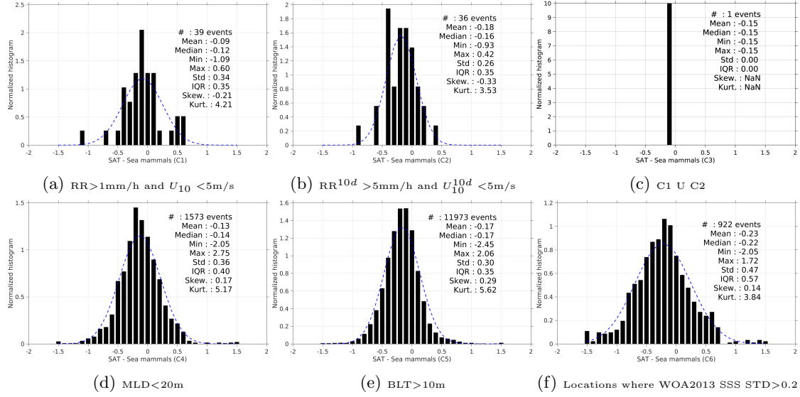
Figure 13: Normalized histogram of \Delta SSS (SMOS-L3-BEC-OA-V1-9DAYS-0.25DEG - Sea mammals) for 6 different subdatasets corresponding to: RR > 1\text{mm/h} and U_{10} < 5\text{m/s} (a), RR^{10d} > 5\text{mm/h} and U_{10}^{10d} < 5\text{m/s} (b), C1 U C2 (c), MLD < 20\text{m} (d), BLT > 10\text{m} (e), Locations where WOA2013 SSS STD > 0.2 (f).
