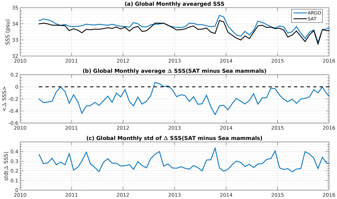
Figure 7: Time series of the monthly averaged mean SSS (top), mean \Delta SSS (Satellite - Sea mammals) and STD of \Delta SSS (Satellite - Sea mammals) over the SMOS coastal zone ( \pm 800\text{km} ) 60N-60S Pi-MEP region considering all match-ups collected by the Pi-MEP platform.
