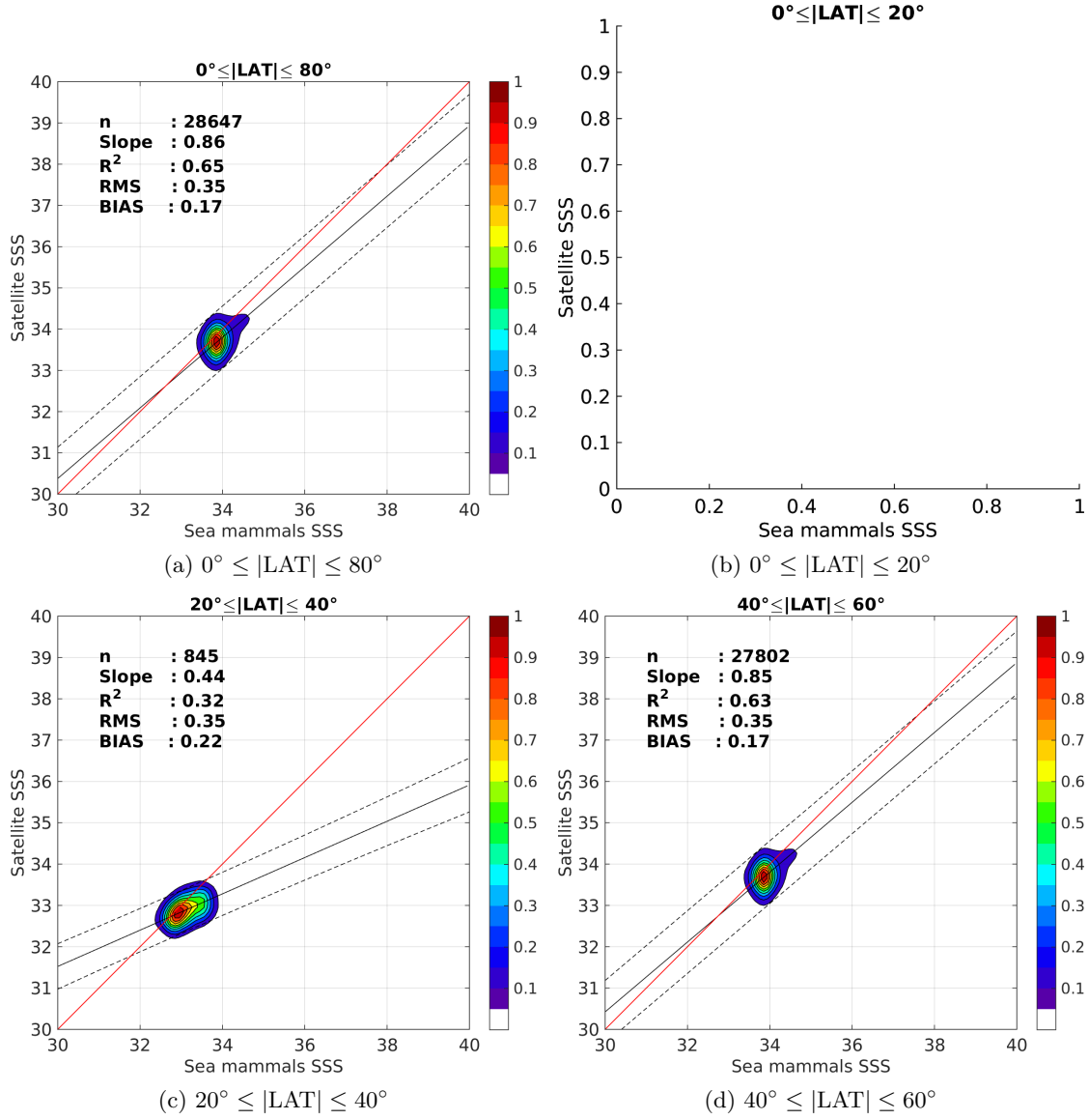
Figure 9: Contour maps of the concentration of SMOS-L3-BEC-OA-V1-9DAYS-0.25DEG SSS (y-axis) versus Sea mammals SSS (x-axis) at match-up pairs for different latitude bands. For each plot, the red line shows x=y . The black thin and dashed lines indicate a linear fit through the data cloud and the \pm 95\% confidence levels, respectively. The number match-up pairs n , the slope and R^2 coefficient of the linear fit, the root mean square (RMS) and the mean bias between satellite and in situ data are indicated for each latitude band in each plots.
