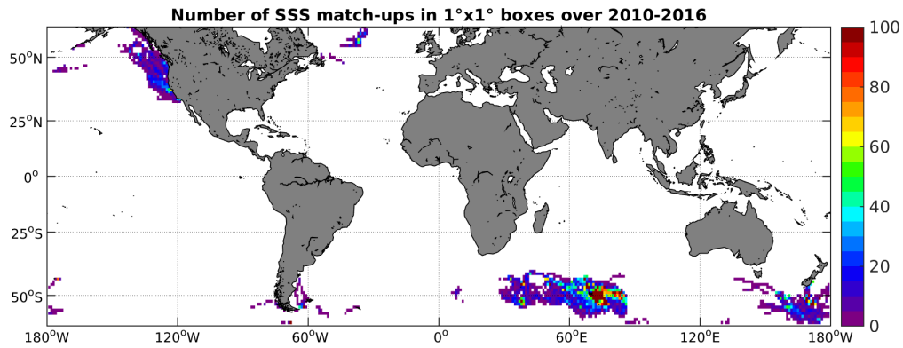
Figure 4: Number of SSS match-ups between Sea mammals SSS and the SMOS-L3-BEC-OA-V1-9DAYS-0.25DEG SSS product for the SMOS coastal zone ( \pm 800\text{km} ) 60N-60S Pi-MEP region over 1^\circ \times 1^\circ boxes and for the full satellite product period.
