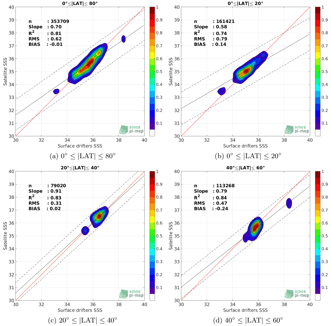
Figure 8: Contour maps of the concentration of SMOS-L3-BEC-OA-V1-9DAYS-0.25DEG SSS (y-axis) versus Surface drifters SSS (x-axis) at match-up pairs for different latitude bands. For each plot, the red line shows x=y . The black thin and dashed lines indicate a linear fit through the data cloud and the \pm 95\% confidence levels, respectively. The number match-up pairs n , the slope and R^2 coefficient of the linear fit, the root mean square (RMS) and the mean bias between satellite and in situ data are indicated for each latitude band in each plots.
