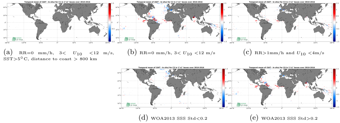
Figure 11: Temporal mean gridded over spatial boxes of size 1^\circ \times 1^\circ of \Delta SSS (SMOS-L3-BEC-OA-V1-9DAYS-0.25DEG - Surface drifters) for 5 different subdatasets corresponding to: RR=0 mm/h, 3 < U_{10} < 12 m/s, SST > 5^\circ C , distance to coast > 800 km (a), RR=0 mm/h, 3 < U_{10} < 12 m/s (b), RR > 1 mm/h and U_{10} < 4 m/s (c), WOA2013 SSS Std < 0.2 (d), WOA2013 SSS Std > 0.2 (e).
