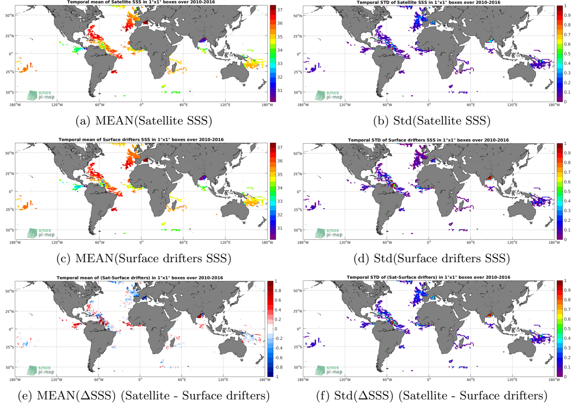
Figure 5: Temporal mean (left) and Std (right) of SSS from SMOS-L3-BEC-OA-V1-9DAYS-0.25DEG (top), Surface drifters (middle), and of \Delta SSS (Satellite - Surface drifters). Only match-up pairs are used to generate these maps.
