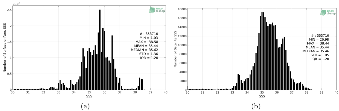
Figure 2: Histograms of SSS from Surface drifters (a) and SMOS-L3-BEC-OA-V1-9DAYS-0.25DEG (b) considering all match-up pairs per bins of 0.1 over the SMOS coastal zone ( \geq 800 km) 60N-60S Pi-MEP region and for the full satellite product period.
