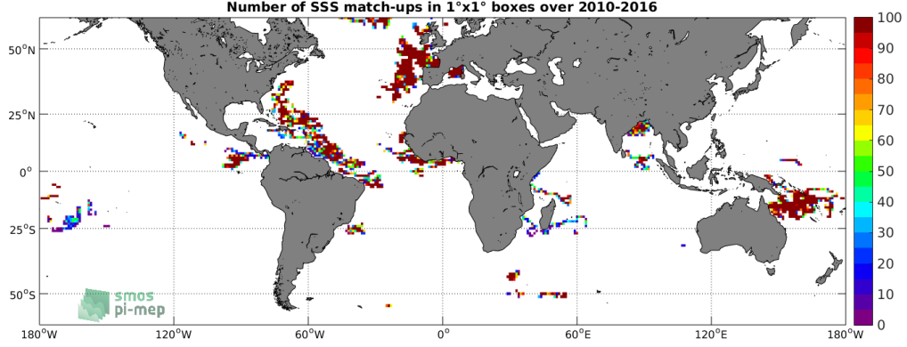
Figure 3: Number of SSS match-ups between Surface drifters SSS and the SMOS-L3-BEC-OA-V1-9DAYS-0.25DEG SSS product for the SMOS coastal zone ( \pm 800\text{km} ) 60N-60S Pi-MEP region over 1^\circ \times 1^\circ boxes and for the full satellite product period.
