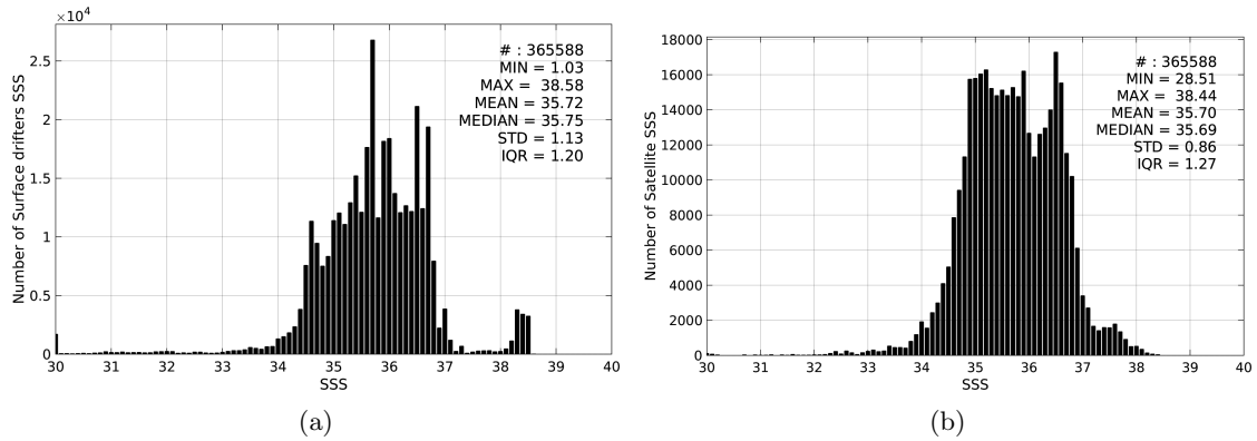
Figure 2: Histograms of SSS from Surface drifters (a) and SMOS-L3-BEC-OA-V1-9DAYS-0.25DEG (b) considering all match-up pairs per bins of 0.1 over the SMOS coastal zone ( \geq 800 km) 60N-60S Pi-MEP region and for the full satellite product period.
