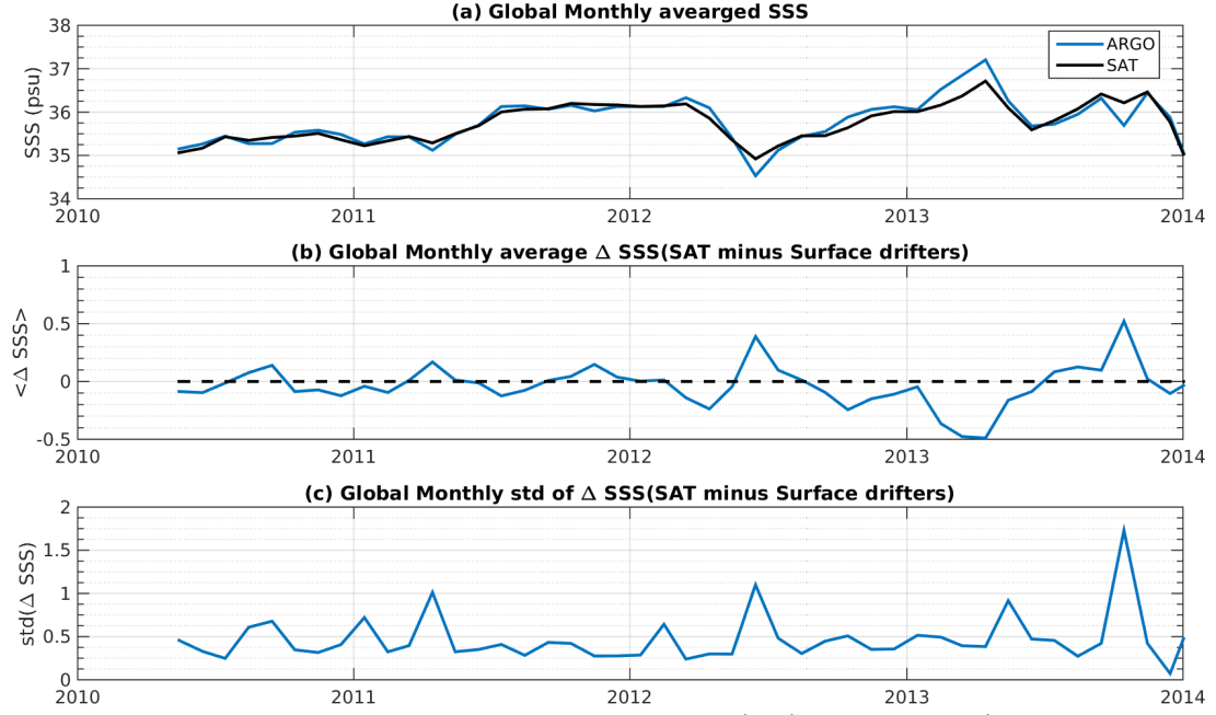
Figure 6: Time series of the monthly averaged mean SSS (top), mean \Delta SSS (Satellite - Surface drifters) and STD of \Delta SSS (Satellite - Surface drifters) over the SMOS coastal zone ( \pm 800\text{km} ) 60N-60S Pi-MEP region considering all match-ups collected by the Pi-MEP platform.
