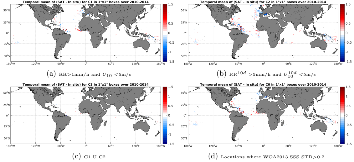
Figure 11: Temporal mean gridded over spatial boxes of size 1^\circ \times 1^\circ of \Delta SSS (SMOS-L3-BEC-OA-V1-9DAYS-0.25DEG - Surface drifters) for 4 different subdatasets corresponding to: RR > 1\text{mm/h} and U_{10} < 5\text{m/s} (a), RR^{10d} > 5\text{mm/h} and U_{10}^{10d} < 5\text{m/s} (b), C1 U C2 (c), Locations where WOA2013 SSS STD > 0.2 (d).
