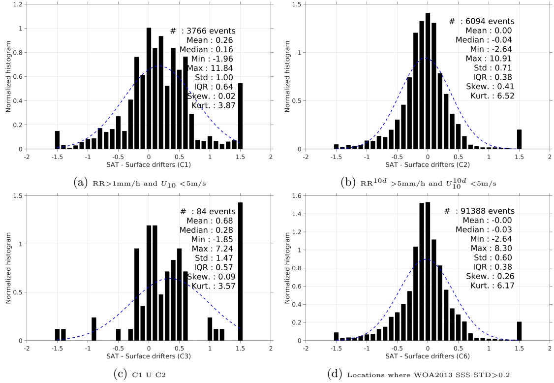
Figure 12: Normalized histogram of \Delta SSS (SMOS-L3-BEC-OA-V1-9DAYS-0.25DEG - Surface drifters) for 6 different subdatasets corresponding to: RR > 1\text{mm/h} and U_{10} < 5\text{m/s} (a), RR^{10d} > 5\text{mm/h} and U_{10}^{10d} < 5\text{m/s} (b), C1 U C2 (c), Locations where WOA2013 SSS STD > 0.2 (d).
