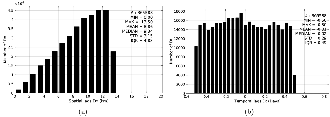
Figure 4: Histograms of the spatial (a) and temporal (b) lags between the time of the Surface drifters measurements and the date of the corresponding SMOS-L3-BEC-OA-V1-9DAYS-0.25DEG SSS product.
