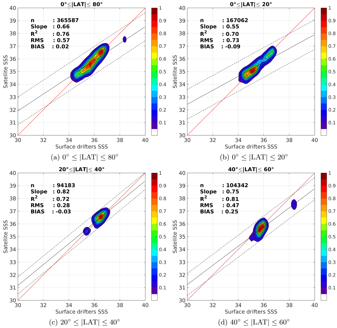
Figure 8: Contour maps of the concentration of SMOS-L3-BEC-OA-V1-9DAYS-0.25DEG SSS (y-axis) versus Surface drifters SSS (x-axis) at match-up pairs for different latitude bands. For each plot, the red line shows x=y . The black thin and dashed lines indicate a linear fit through the data cloud and the \pm 95\% confidence levels, respectively. The number match-up pairs n , the slope and R^2 coefficient of the linear fit, the root mean square (RMS) and the mean bias between satellite and in situ data are indicated for each latitude band in each plots.
