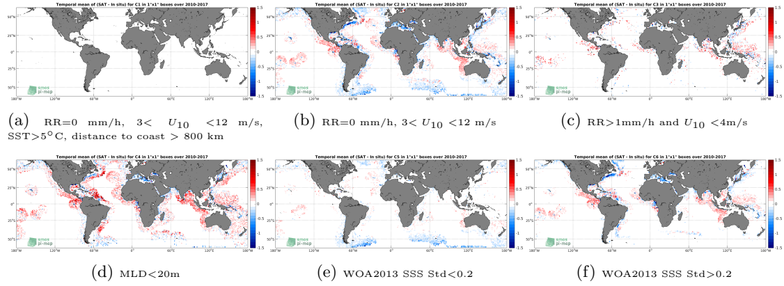
Figure 12: Temporal mean gridded over spatial boxes of size 1^\circ \times 1^\circ of \Delta SSS (SMOS-L3-BEC-OA-V1-9DAYS-0.25DEG - Argo) for 6 different subdatasets corresponding to: RR=0 mm/h, 3 < U_{10} < 12 m/s, SST > 5^\circ C , distance to coast > 800 km (a), RR=0 mm/h, 3 < U_{10} < 12 m/s (b), RR > 1 mm/h and U_{10} < 4 m/s (c), MLD < 20 m (d), WOA2013 SSS Std < 0.2 (e), WOA2013 SSS Std > 0.2 (f).
