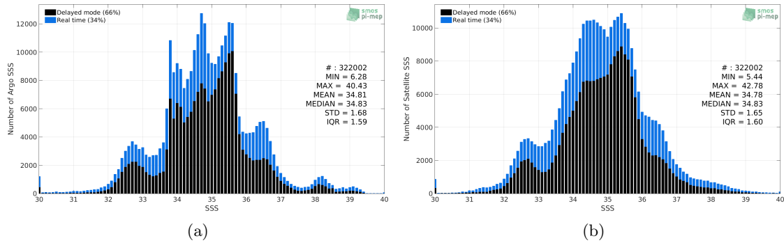
Figure 2: Histograms of SSS from Argo (a) and SMOS-L3-BEC-OA-V1-9DAYS-0.25DEG (b) considering all match-up pairs per bins of 0.1 over the SMOS coastal zone (¡800km) 60N-60S Pi-MEP region and for the full satellite product period.
