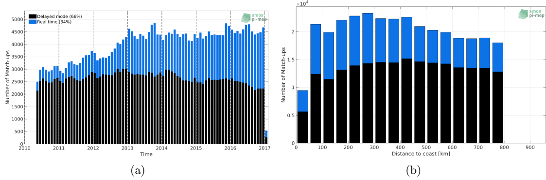
Figure 1: Number of match-ups between Argo and SMOS-L3-BEC-OA-V1-9DAYS-0.25DEG SSS as a function of time (a) and as function of the distance to coast (b) over the SMOS coastal zone (¡800km) 60N-60S Pi-MEP region and for the full satellite product period.
