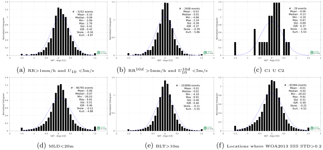
Figure 13: Normalized histogram of \Delta SSS (SMOS-L3-BEC-OA-V1-9DAYS-0.25DEG - Argo) for 6 different subdatasets corresponding to: RR > 1\text{mm/h} and U_{10} < 5\text{m/s} (a), RR^{10d} > 5\text{mm/h} and U_{10}^{10d} < 5\text{m/s} (b), C1 U C2 (c), MLD < 20\text{m} (d), BLT > 10\text{m} (e), Locations where WOA2013 SSS STD > 0.2 (f).
