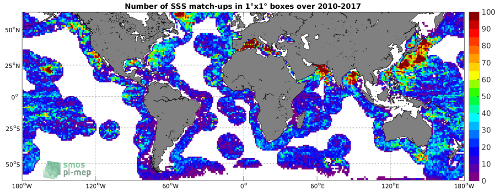
Figure 4: Number of SSS match-ups between Argo SSS and the SMOS-L3-BEC-OA-V1-9DAYS-0.25DEG SSS product for the SMOS coastal zone ( \approx 800\text{km} ) 60N-60S Pi-MEP region over 1^\circ \times 1^\circ boxes and for the full satellite product period.
