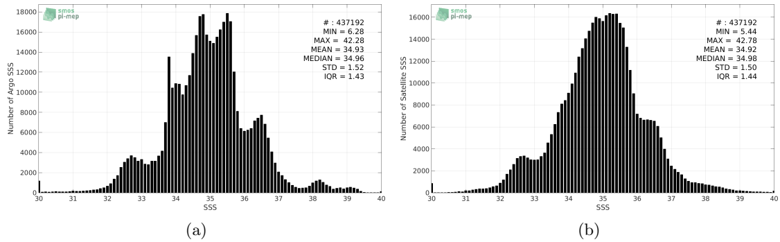
Figure 2: Histograms of SSS from Argo (a) and SMOS-L3-BEC-OA-V1-9DAYS-0.25DEG (b) considering all match-up pairs per bins of 0.1 over the SMOS coastal zone ( \geq 800 km) 60N-60S Pi-MEP region and for the full satellite product period.
