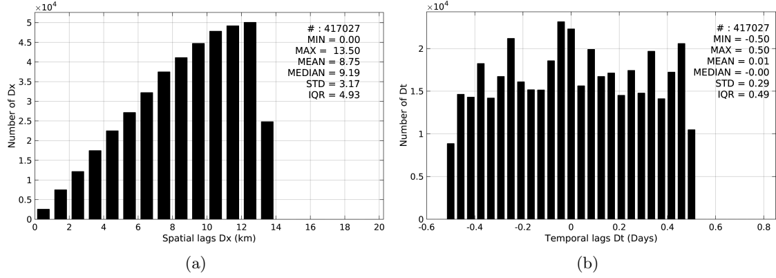
Figure 5: Histograms of the spatial (a) and temporal (b) lags between the time of the Argo measurements and the date of the corresponding SMOS-L3-BEC-OA-V1-9DAYS-0.25DEG SSS product.
