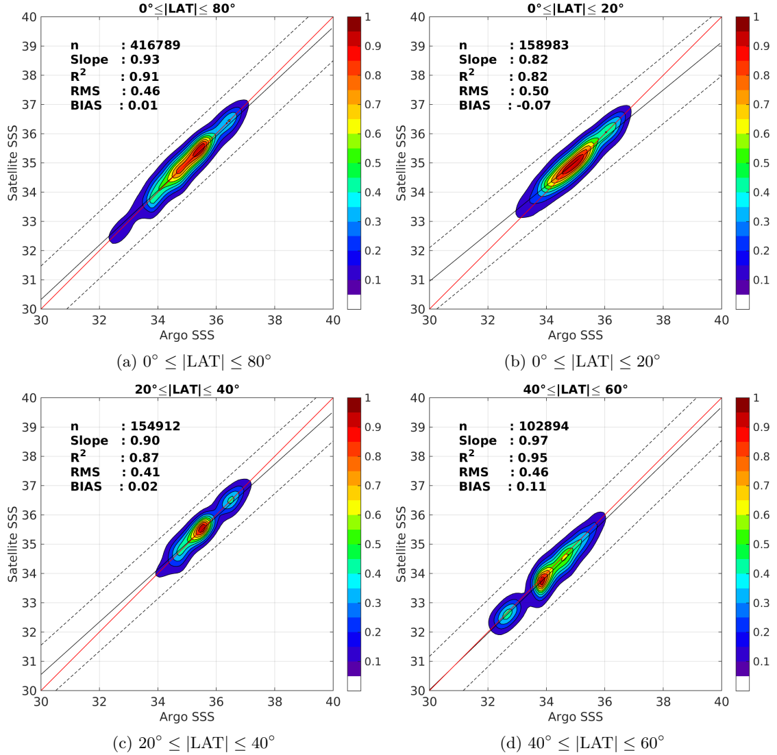
Figure 9: Contour maps of the concentration of SMOS-L3-BEC-OA-V1-9DAYS-0.25DEG SSS (y-axis) versus Argo SSS (x-axis) at match-up pairs for different latitude bands. For each plot, the red line shows x=y . The black thin and dashed lines indicate a linear fit through the data cloud and the \pm 95\% confidence levels, respectively. The number match-up pairs n , the slope and R^2 coefficient of the linear fit, the root mean square (RMS) and the mean bias between satellite and in situ data are indicated for each latitude band in each plots.
