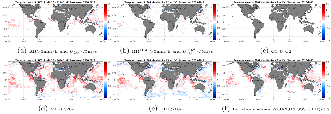
Figure 12: Temporal mean gridded over spatial boxes of size 1^\circ \times 1^\circ of \Delta SSS (SMOS-L3-BEC-OA-V1-9DAYS-0.25DEG - Argo) for 6 different subdatasets corresponding to: RR > 1\text{mm/h} and U_{10} < 5\text{m/s} (a), RR^{10d} > 5\text{mm/h} and U_{10}^{10d} < 5\text{m/s} (b), C1 U C2 (c), MLD < 20\text{m} (d), BLT > 10\text{m} (e), Locations where WOA2013 SSS STD > 0.2 (f).
