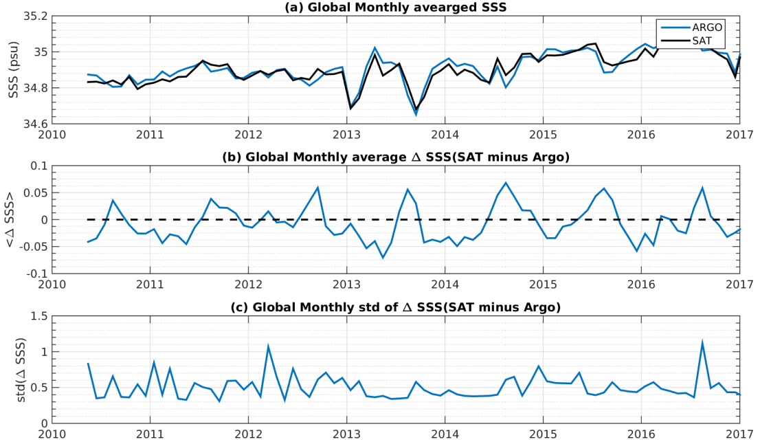
Figure 7: Time series of the monthly averaged mean SSS (top), mean \Delta SSS (Satellite - Argo) and STD of \Delta SSS (Satellite - Argo) over the SMOS coastal zone ( \geq 800\text{km} ) 60N-60S Pi-MEP region considering all match-ups collected by the Pi-MEP platform.
