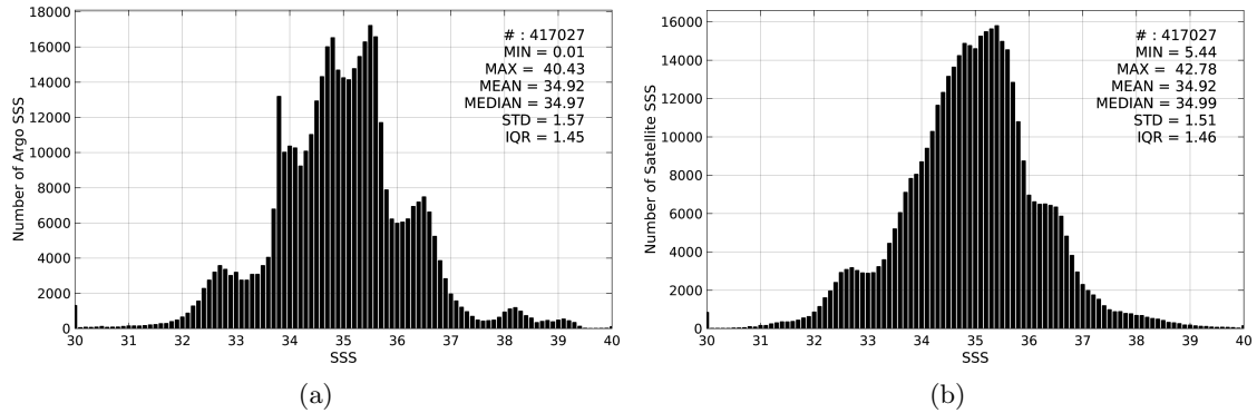
Figure 2: Histograms of SSS from Argo (a) and SMOS-L3-BEC-OA-V1-9DAYS-0.25DEG (b) considering all match-up pairs per bins of 0.1 over the SMOS coastal zone ( \geq 800 km) 60N-60S Pi-MEP region and for the full satellite product period.
