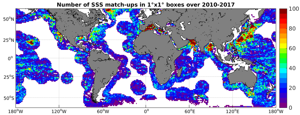
Figure 4: Number of SSS match-ups between Argo SSS and the SMOS-L3-BEC-OA-V1-9DAYS-0.25DEG SSS product for the SMOS coastal zone ( \geq 800\text{km} ) 60N-60S Pi-MEP region over 1^\circ \times 1^\circ boxes and for the full satellite product period.
