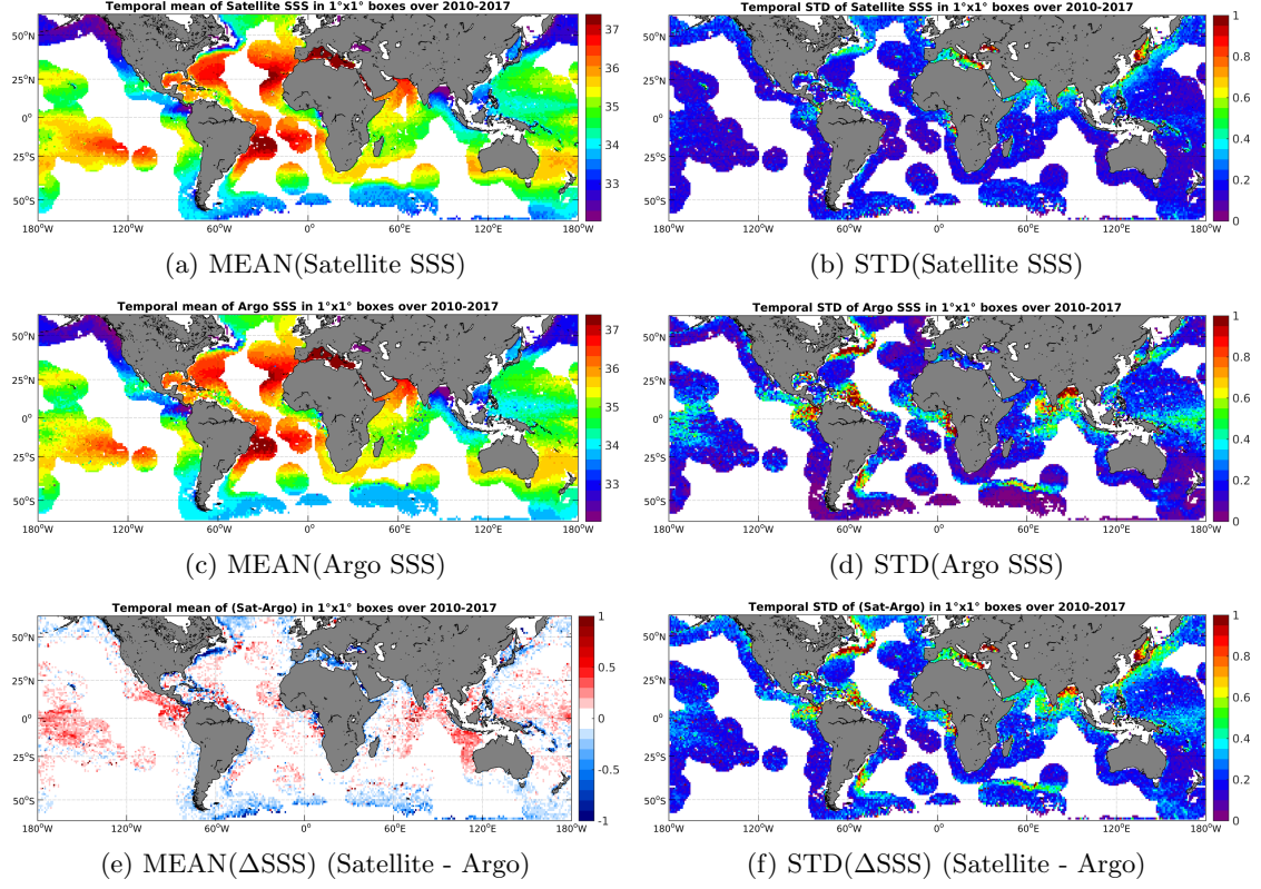
Figure 6: Temporal mean (left) and STD (right) of SSS from SMOS-L3-BEC-OA-V1-9DAYS-0.25DEG (top), Argo (middle), and of \Delta SSS (Satellite - Argo). Only match-up pairs are used to generate these maps.
