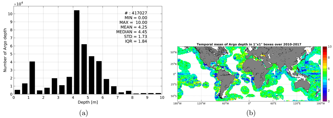
Figure 3: Histograms of the depth of the upper level SSS measurements from Argo in the Match-up DataBase for the SMOS coastal zone ( \geq 800\text{km} ) 60N-60S Pi-MEP region (a) and temporal mean spatial distribution of pressure of the in situ SSS data over 1^\circ \times 1^\circ boxes and for the full satellite product period (b).
