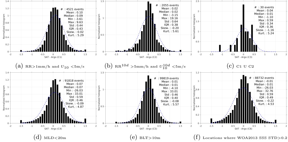
Figure 13: Normalized histogram of \Delta SSS (SMOS-L3-BEC-OA-V1-9DAYS-0.25DEG - Argo) for 6 different subdatasets corresponding to: RR > 1\text{mm/h} and U_{10} < 5\text{m/s} (a), RR^{10d} > 5\text{mm/h} and U_{10}^{10d} < 5\text{m/s} (b), C1 U C2 (c), MLD < 20\text{m} (d), BLT > 10\text{m} (e), Locations where WOA2013 SSS STD > 0.2 (f).
