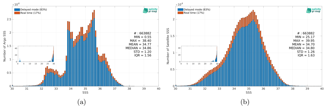
Figure 3: Histograms of SSS from Argo (a) and SMOS SSS L2-AVERAGED v700 (ESA) (b) considering all match-up pairs per bins of 0.1 over the SMOS coastal zone (<800km) 60N-60S Pi-MEP region and for the full satellite product period.
