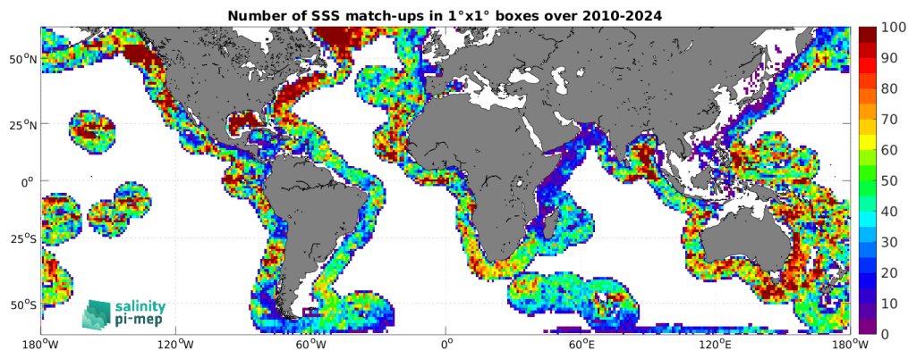
Figure 5: Number of SSS match-ups between Argo SSS and the SMOS SSS L2-AVERAGED v700 (ESA) SSS product for the SMOS coastal zone ( <800\text{km} ) 60N-60S Pi-MEP region over 1^\circ \times 1^\circ boxes and for the full satellite product period.
