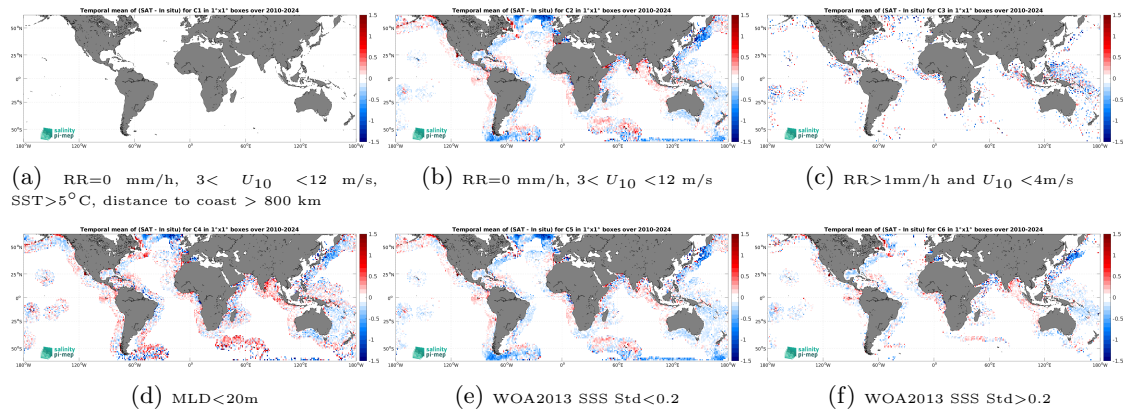
Figure 14: Temporal mean gridded over spatial boxes of size 1^\circ \times 1^\circ of \Delta SSS (SMOS SSS L2-AVERAGED v700 (ESA) - Argo) over 6 different subdatasets corresponding to:RR=0 mm/h, 3 < U_{10} < 12 m/s, SST >5^\circ C, distance to coast > 800 km (a), RR=0 mm/h, 3 < U_{10} < 12 m/s (b), RR >1 mm/h and U_{10} < 4 m/s (c),MLD <20 m (d),WOA2013 SSS Std <0.2 (e),WOA2013 SSS Std >0.2 (f).
