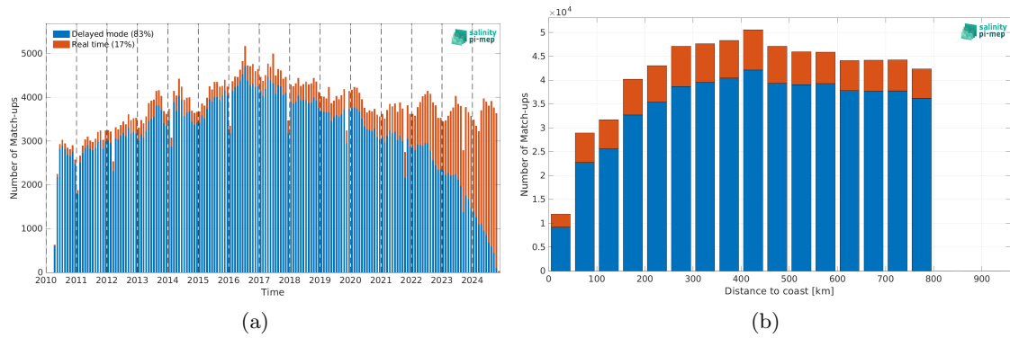
Figure 2: Number of match-ups between Argo and SMOS SSS L2-AVERAGED v700 (ESA) SSS as a function of time (a) and as function of the distance to coast (b) over the SMOS coastal zone (<800km) 60N-60S Pi-MEP region and for the full satellite product period.
