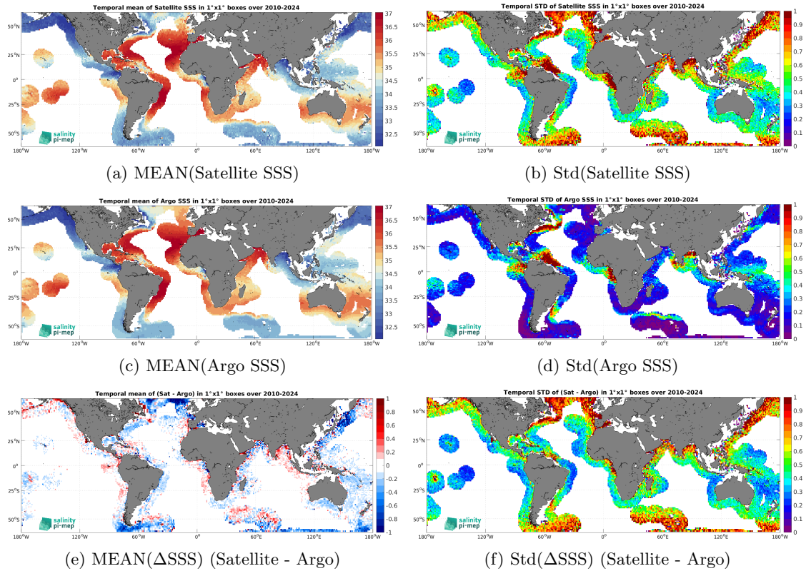
Figure 7: Temporal mean (left) and Std (right) of SSS from SMOS SSS L2-AVERAGED v700 (ESA) (top), Argo (middle), and of \Delta SSS (Satellite - Argo). Only match-up pairs are used to generate these maps.
