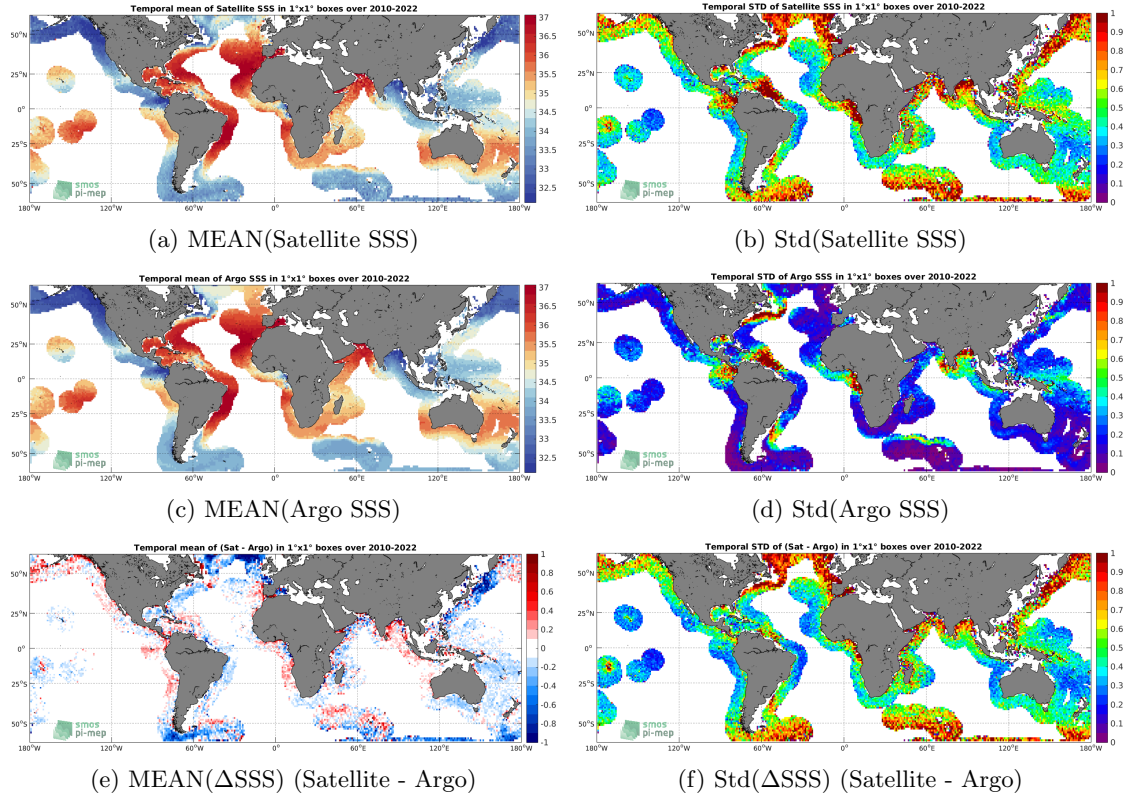
Figure 6: Temporal mean (left) and Std (right) of SSS from SMOS SSS L2-AVERAGED v700 (ESA) (top), Argo (middle), and of \Delta SSS (Satellite - Argo). Only match-up pairs are used to generate these maps.
