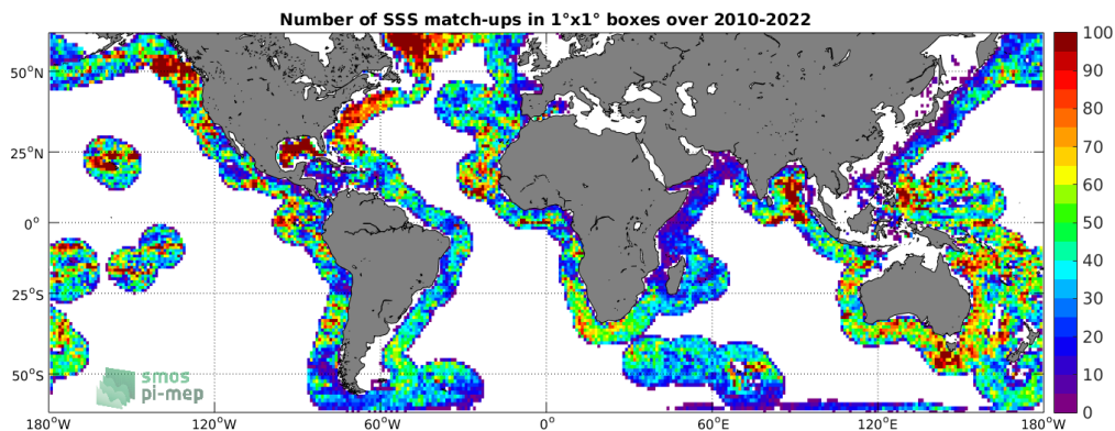
Figure 4: Number of SSS match-ups between Argo SSS and the SMOS SSS L2-AVERAGED v700 (ESA) SSS product for the SMOS coastal zone (<800km) 60N-60S Pi-MEP region over 1^\circ \times 1^\circ boxes and for the full satellite product period.
