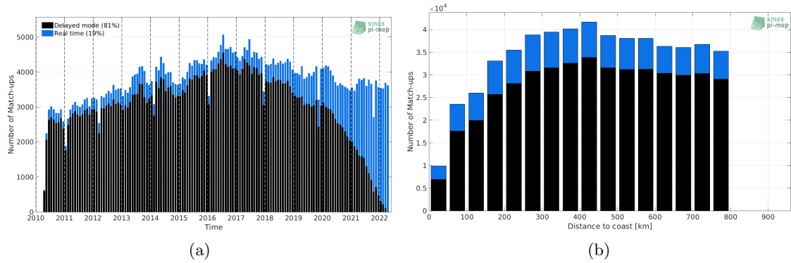
Figure 1: Number of match-ups between Argo and SMOS SSS L2-AVERAGED v700 (ESA) SSS as a function of time (a) and as function of the distance to coast (b) over the SMOS coastal zone (<800km) 60N-60S Pi-MEP region and for the full satellite product period.
