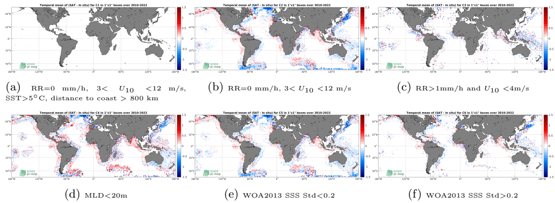
Figure 12: Temporal mean gridded over spatial boxes of size 1^\circ \times 1^\circ of \Delta SSS (SMOS SSS L2-AVERAGED v700 (ESA) - Argo) for 6 different subdatasets corresponding to:RR=0 mm/h, 3 < U_{10} < 12 m/s, SST >5^\circ C, distance to coast > 800 km (a), RR=0 mm/h, 3 < U_{10} < 12 m/s (b), RR >1 mm/h and U_{10} < 4 m/s (c),MLD <20 m (d),WOA2013 SSS Std <0.2 (e),WOA2013 SSS Std >0.2 (f).
