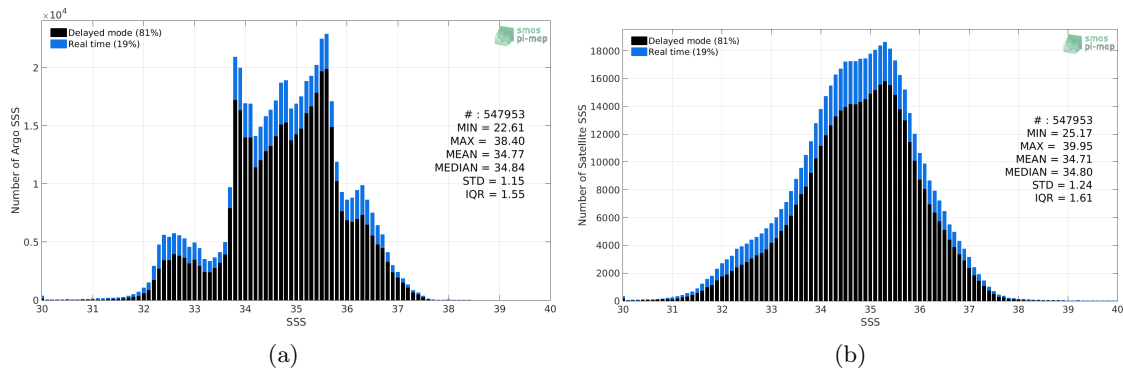
Figure 2: Histograms of SSS from Argo (a) and SMOS SSS L2-AVERAGED v700 (ESA) (b) considering all match-up pairs per bins of 0.1 over the SMOS coastal zone (<800km) 60N-60S Pi-MEP region and for the full satellite product period.
